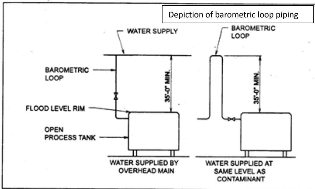
BAROMETRIC LOOP
