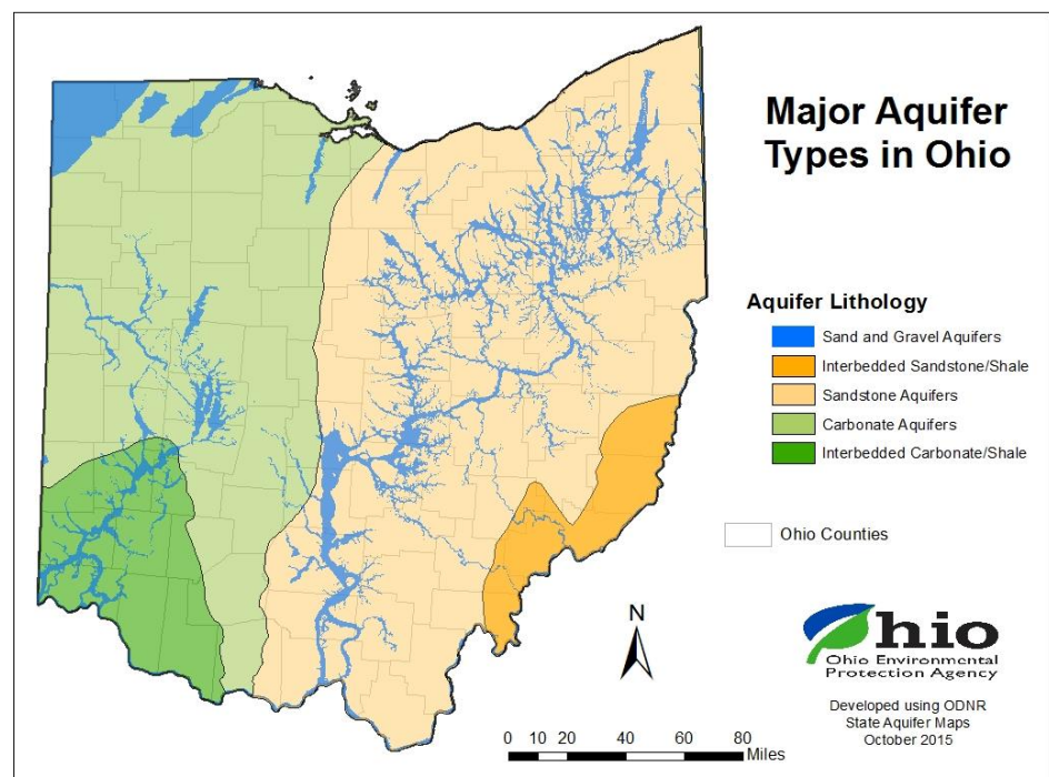
Figure 1 — Major Aquifer Types in Ohio
