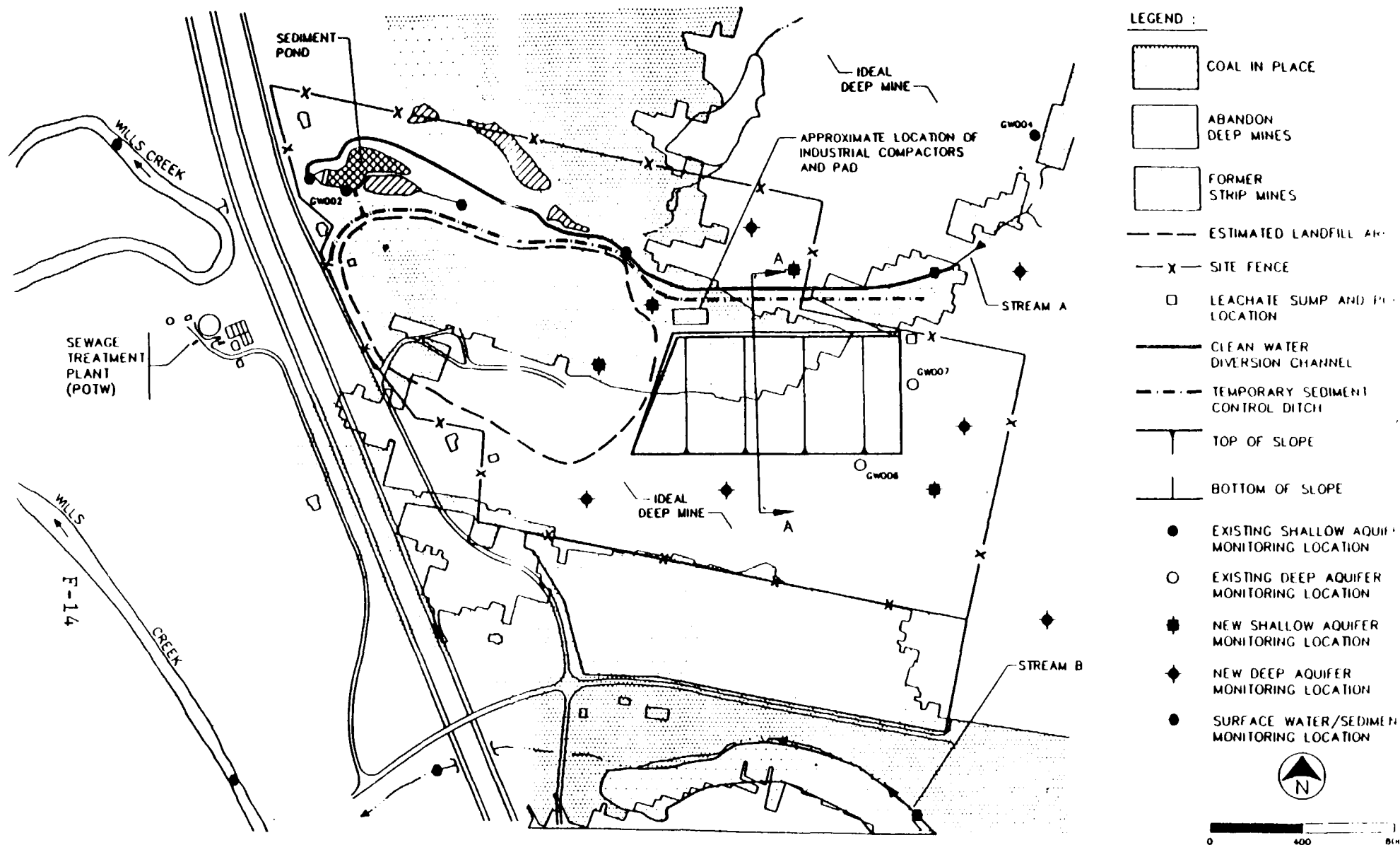
FIGURE 14 ALTERNATIVE 5 ONSITE LANDFILL FULTZ LANDFILL SITE, FEASIBILITY STUDY REPORT
