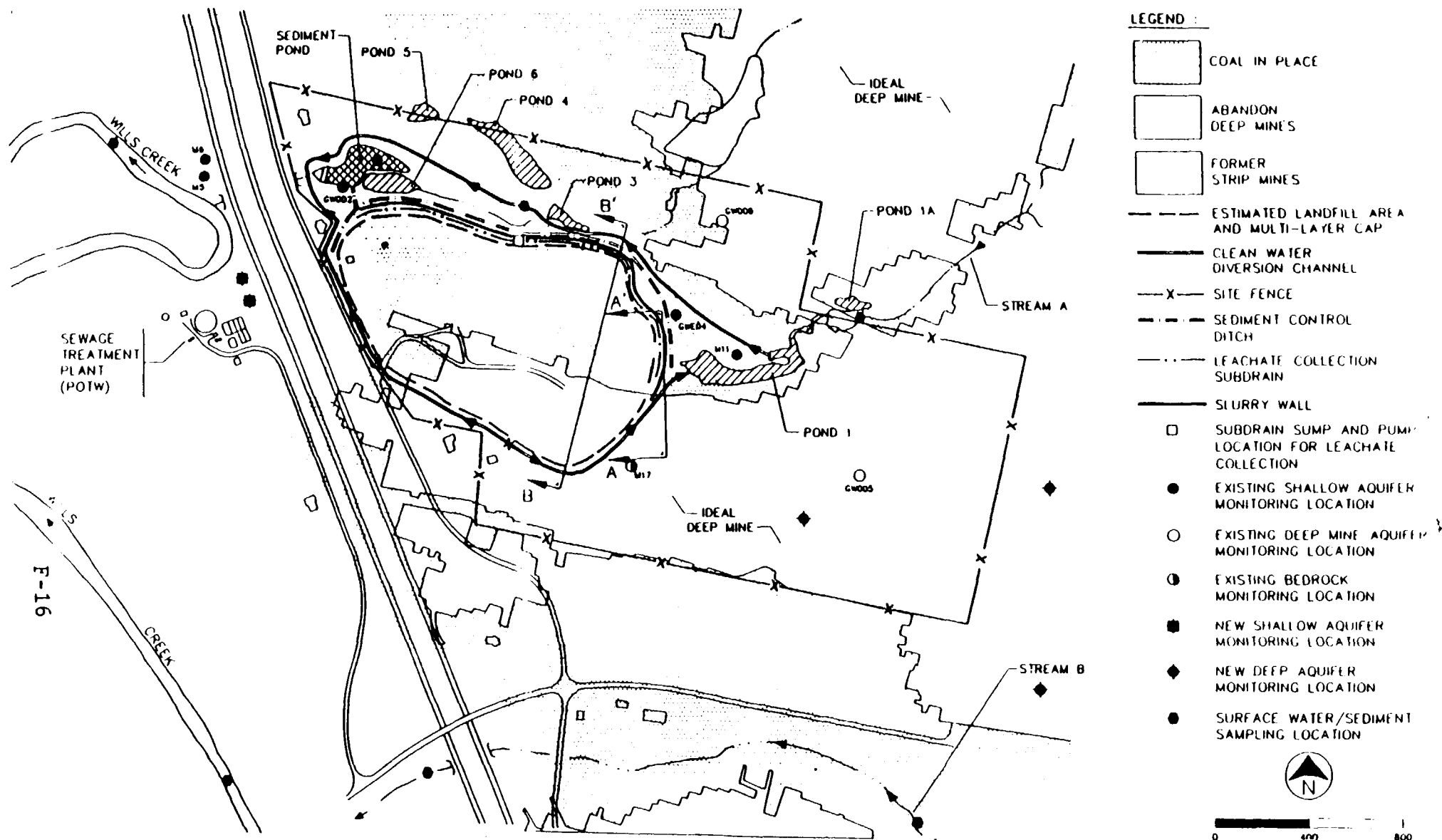
FIGURE 16 ALTERNATIVE 6 MULTI-LAYER CAP WITH SUBSURFACE BARRIER FULTZ LANDFILL SITE, FEASIBILITY STUDY REPORT
