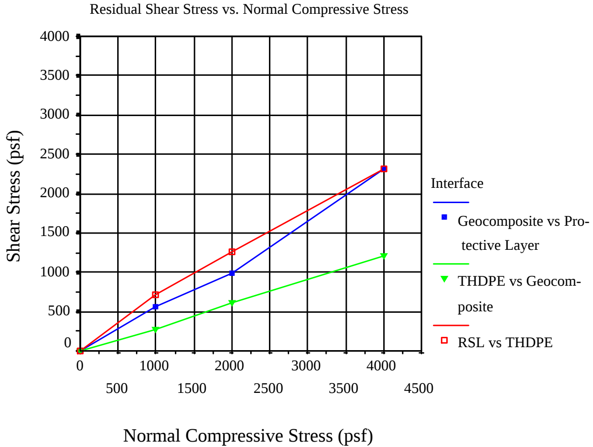
Figure 4-7 An example of individual nonlinear residual shear strength envelopes derived from the lowest residual shear testing data at each normal compressive stress for each of three interfaces in a composite system. The shear stress below 1000 psf normal compressive stress was estimated by drawing a line from the origin to the shear stress at 1000 psf normal compressive stress for each interface. If normal compressive loads greater than 4000 psf are expected at the facility, then additional testing at higher normal compressive loads will be necessary.
