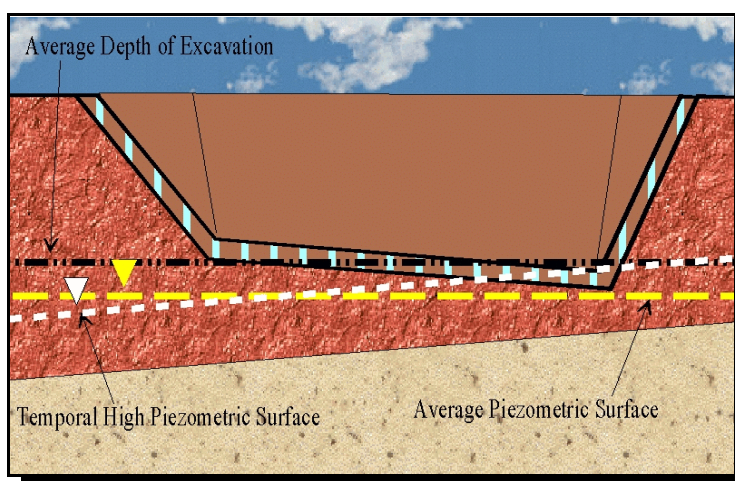
Figure 7-3 Example of how using the average depth of excavation (double-dot dashed line) and the average elevation of the piezometric surface (large dashed line) result in the conclusion that hydrostatic uplift will not occur, which is incorrect. Note that the temporal high piezometric surface (small dashed line) does intersect the liner system (hashed area) creating the potential for hydrostatic uplift that must be analyzed.
