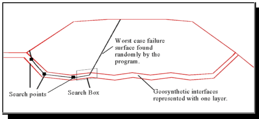
Figure 8-14 Cross Section A-A'. Example translational failure surface found by directing modeling software to a specific interface.
