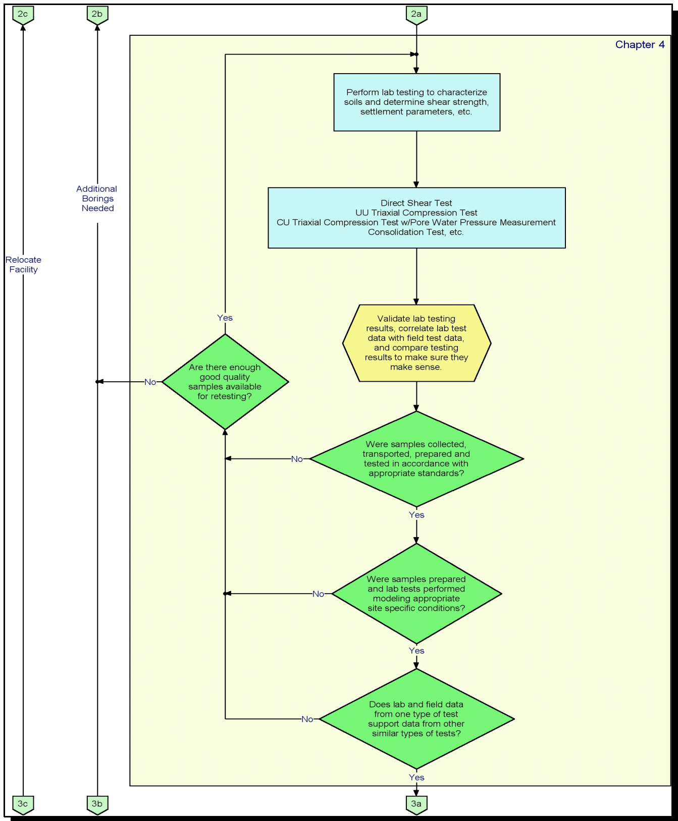
Page 2. Geotechnical and stability analyses flow chart.
