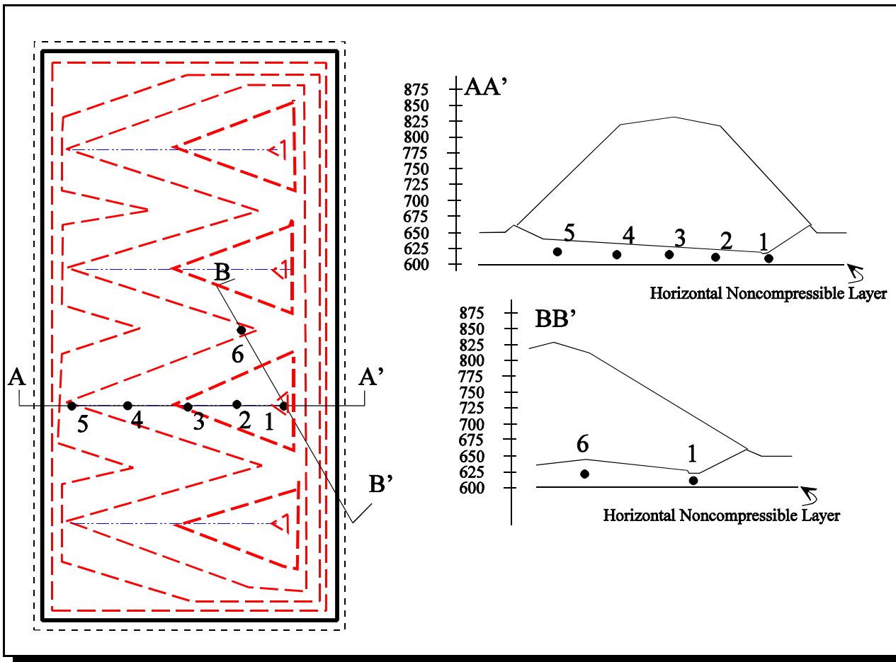
Figure 6-3 Example plan view and cross sections showing some of the locations selected for settlement analysis.
