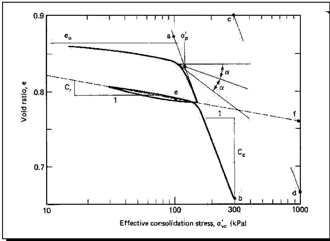
Figure 6-1 Overconsolidated stress diagram. From Ex. Figure 8.9, Holts and Kovacs, pp. 316
