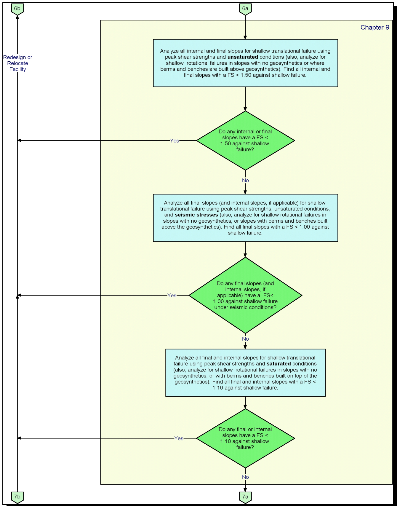
Page 6. Geotechnical and stability analyses flow chart.
