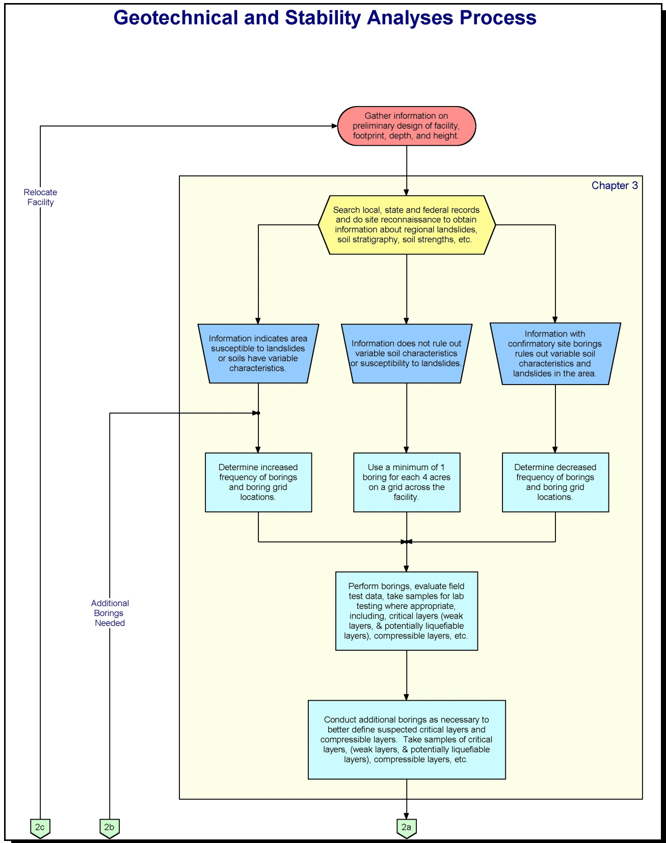
Figure 2-3 Page 1. Geotechnical and stability analyses flow chart.
