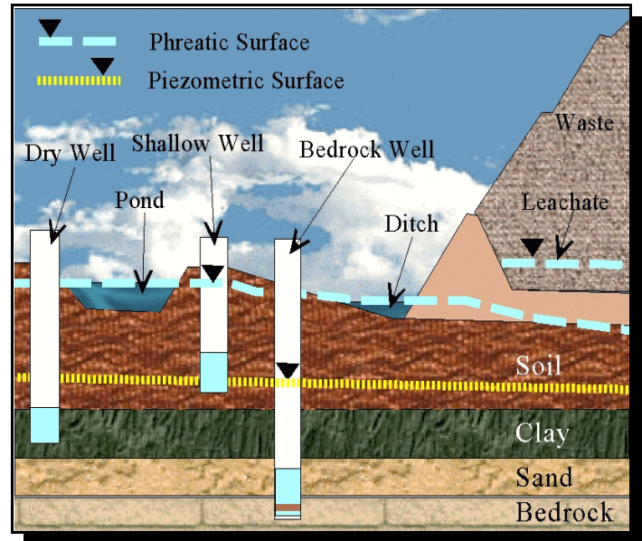
Figure 8-3 Examples of phreatic and piezometric surfaces .
