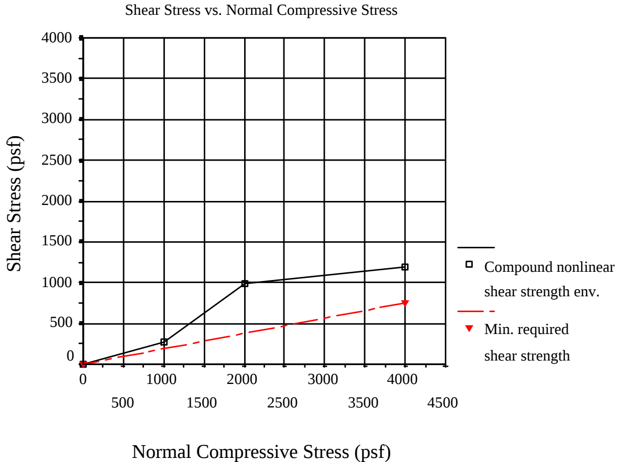
Figure 4-8 An example of a compound nonlinear residual shear strength envelope created from the individual nonlinear residual shear strength envelopes of three interfaces of a composite system. When the residual shear strength envelope is compared to the minimum residual shear strength specified in the authorizing document, it can be seen that the composite system exhibits enough residual shear strength at all normal compressive stresses expected at the facility that, and thus minimum required residual shear strength is exceeded. This ensures that all the tested materials can be used during construction of composite systems when residual shear strength conditions are expected. If normal compressive loads greater than 4000 psf are expected at the facility, then additional testing at higher normal compressive loads will be necessary.
