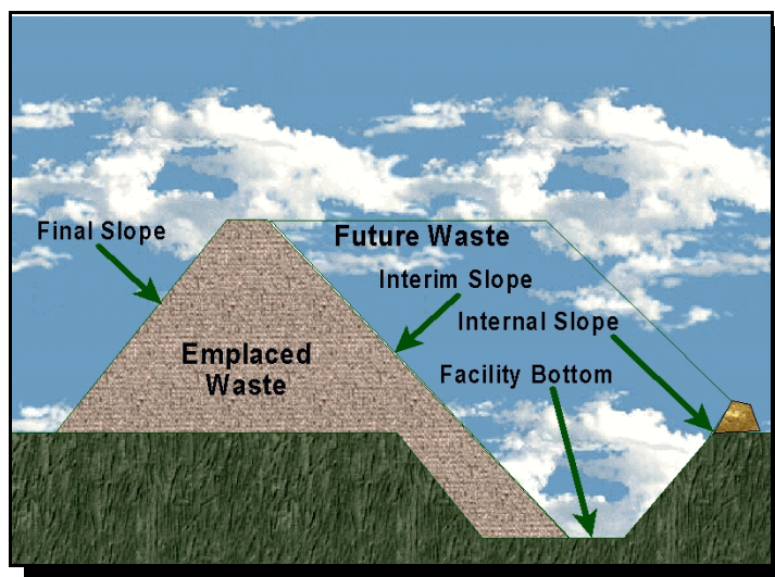
Figure f-1 An example of a typical landfill progression showing internal , interim , and final slopes , and the facility bottom . These types of slopes may also be present at other types of waste containment facilities.
