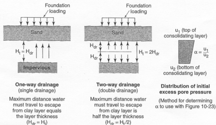
Figure 10-24 Vertical drainage conditions in consolidation theory.
