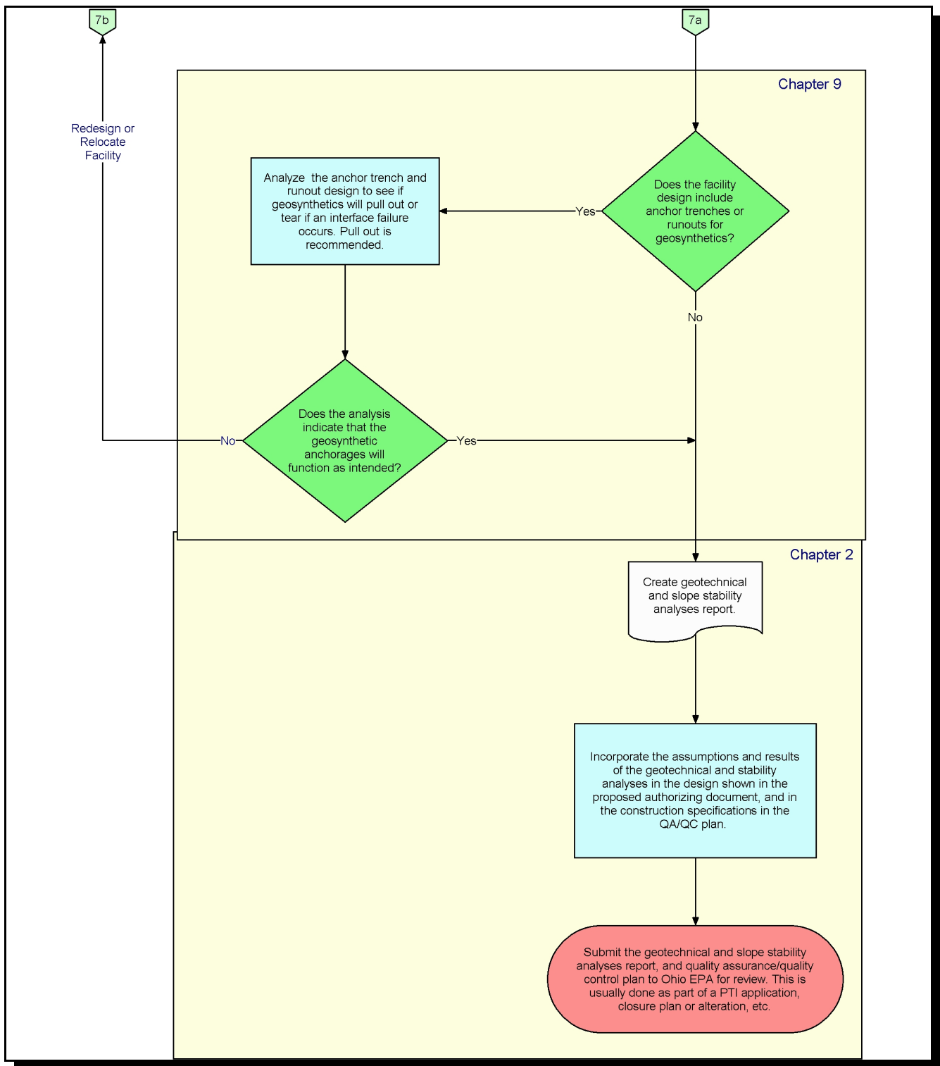
Page 7. Geotechnical and stability analyses flow chart.
