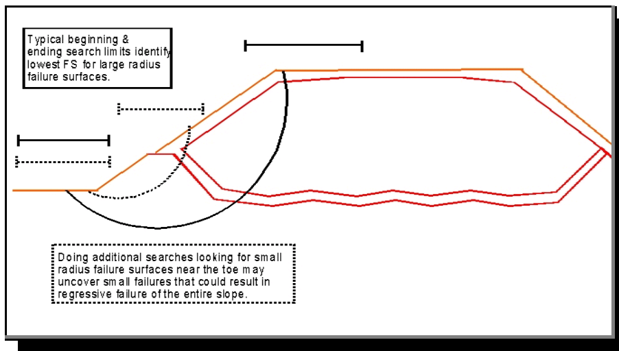
Figure 8-15 Example of using different search limits to look for different size failure surfaces.
