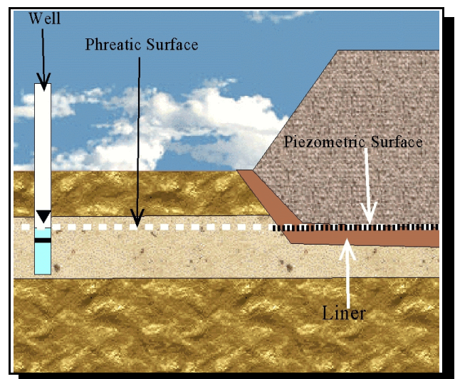
Figure 8-6 Example of a piezometric surface created by engineered components of a waste containment facility .
