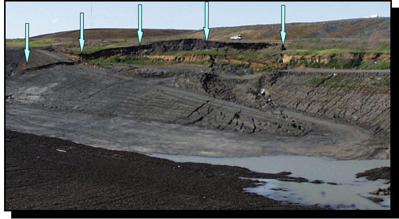
Figure 8-2 A complex rotational failure at a Texas landfill. White arrows identify the failure escarpment. For scale, note the pickup truck above the failure escarpment. Photograph courtesy of Dr. Timothy D. Stark, PE, University of Illinois, Urbana.
