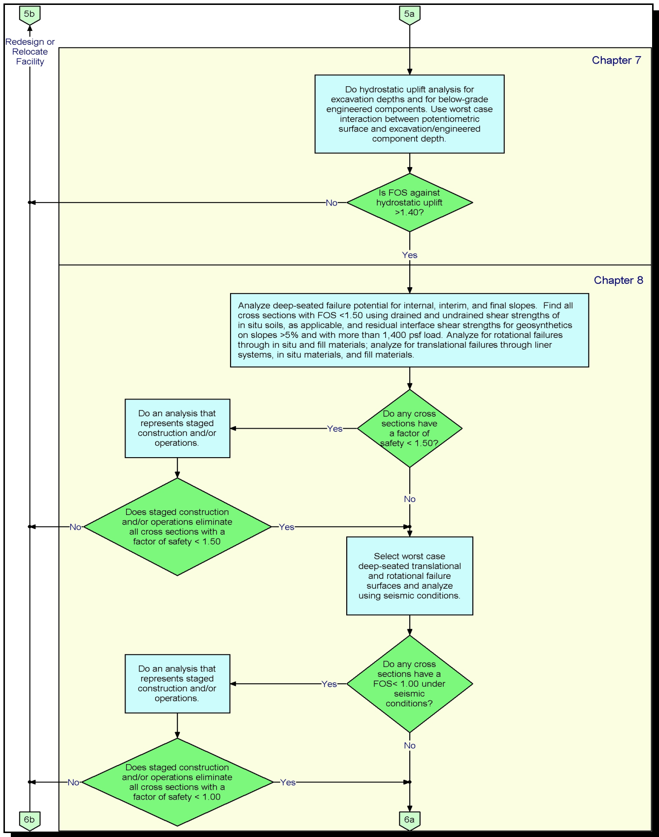
Page 5. Geotechnical and stability analyses flow chart.
