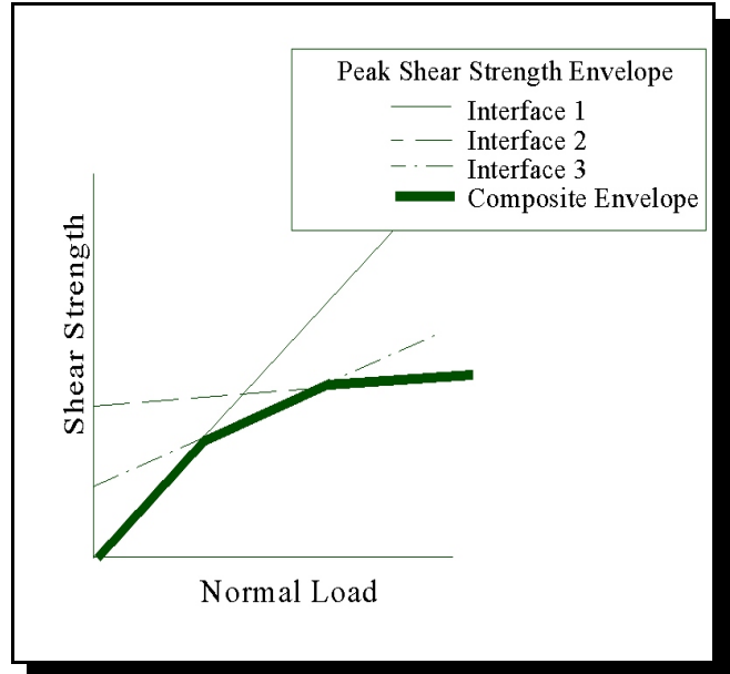
Figure 4-1 Example of a compound peak shear strength envelope for a multi-layered engineered component of a waste containment facility .
