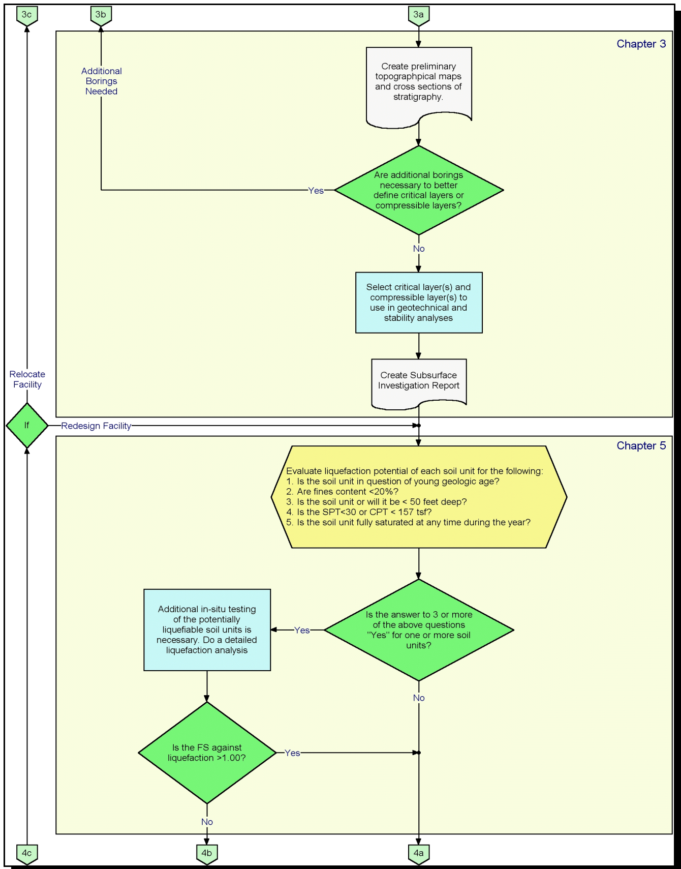
Page 3. Geotechnical and stability analyses flow chart.
