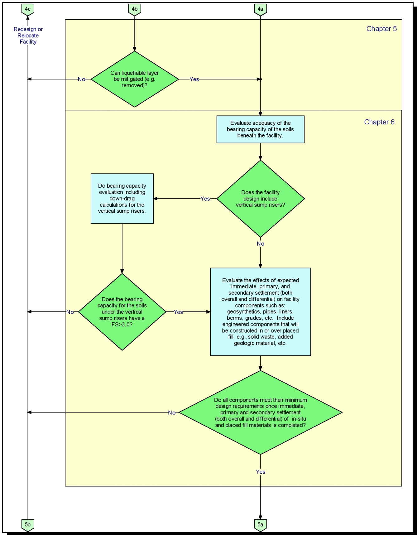
Page 4. Geotechnical and stability analyses flow chart.
