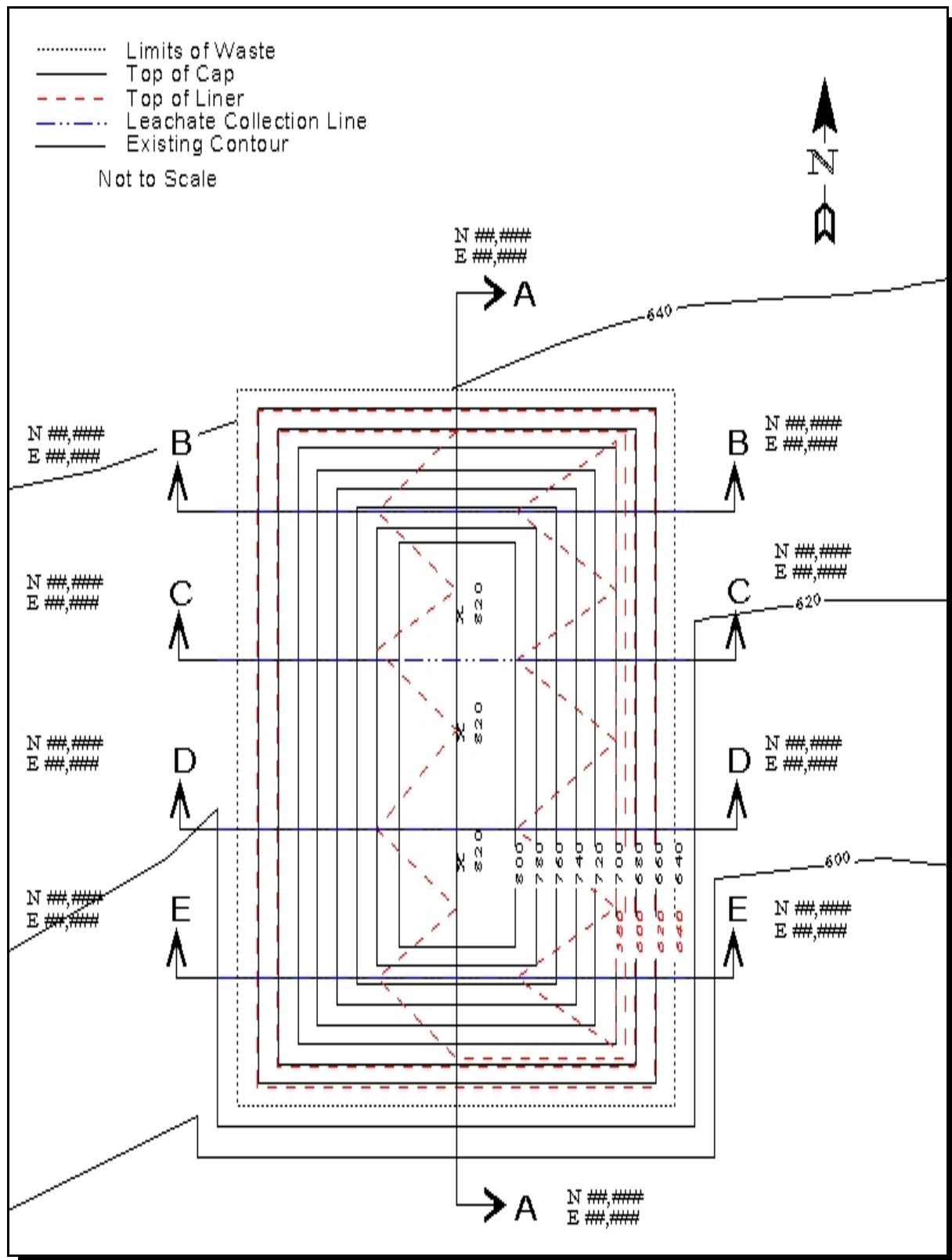
Figure 8-12 Example plan view showing top and bottom elevations and the location of cross sections that were analyzed for stability.
