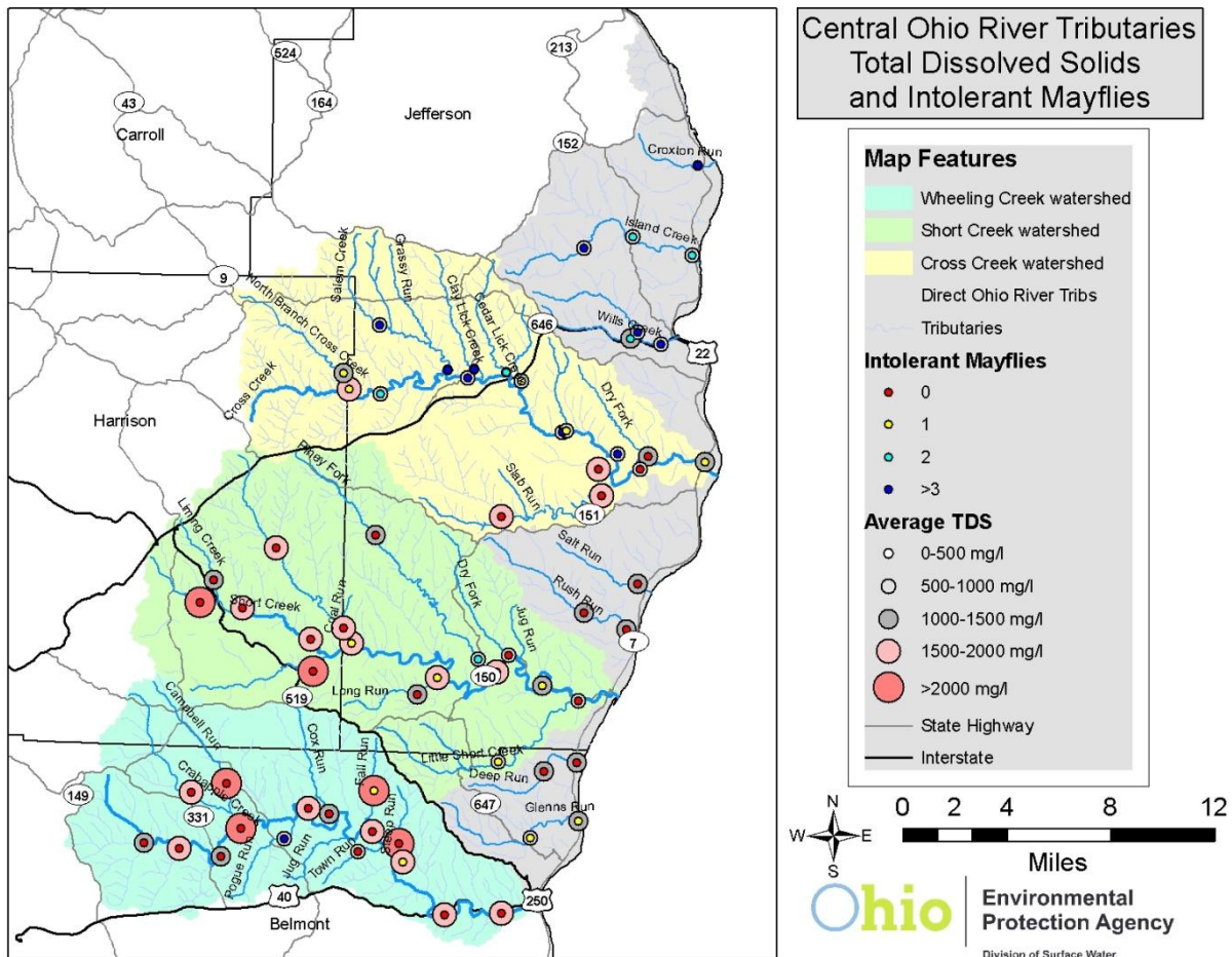
Figure 12. Number of sensitive mayfly taxa compared to the presence of TDS in the CORT study area, 2010.
