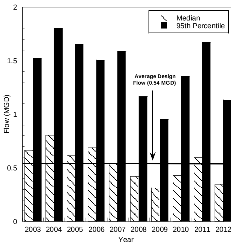
Figure 5. Annual median and 95th percentile effluent flows for the Wintersville WWTP, 2003 - 2012.
