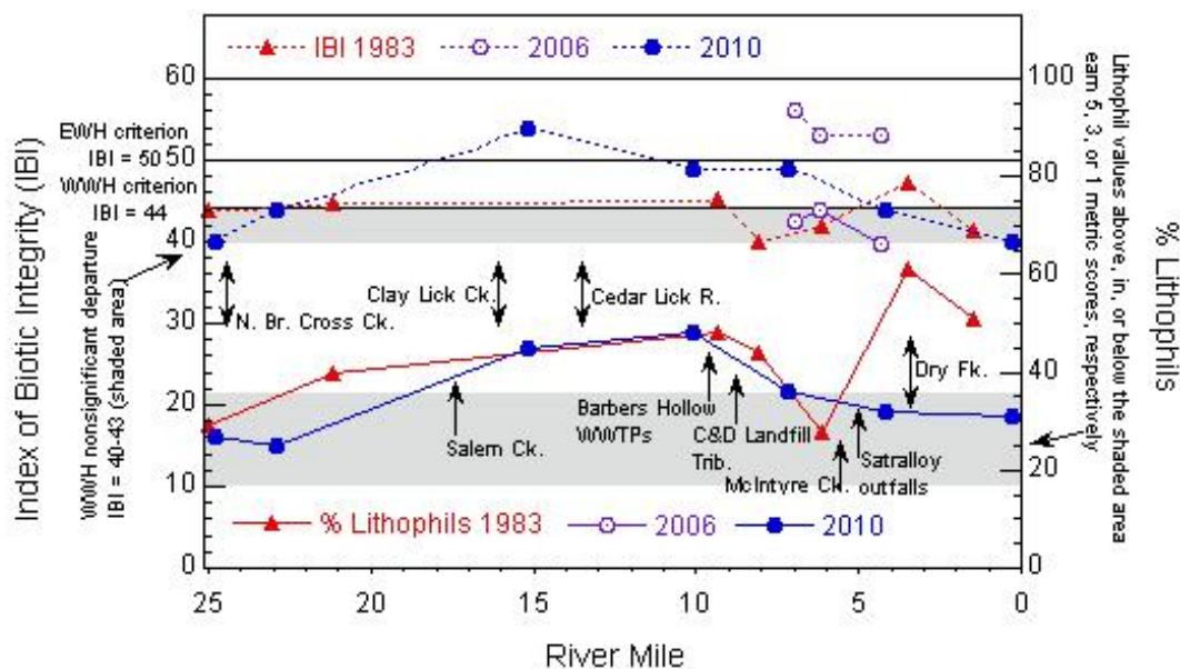
Figure 11. Comparison of IBI scores (left y axis) with the percentage of lithophilic fish (right y axis) in Cross Creek, 1983-2010. Declines downstream from the C&D Landfill implicate it as a source of excessive sediment pollution.
