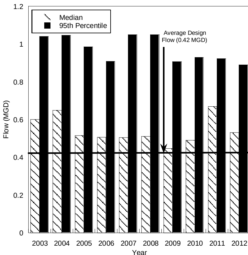
Figure 6. Annual median and 95th percentile effluent flows for the Jefferson M WWTP, 2003 - 2012.
