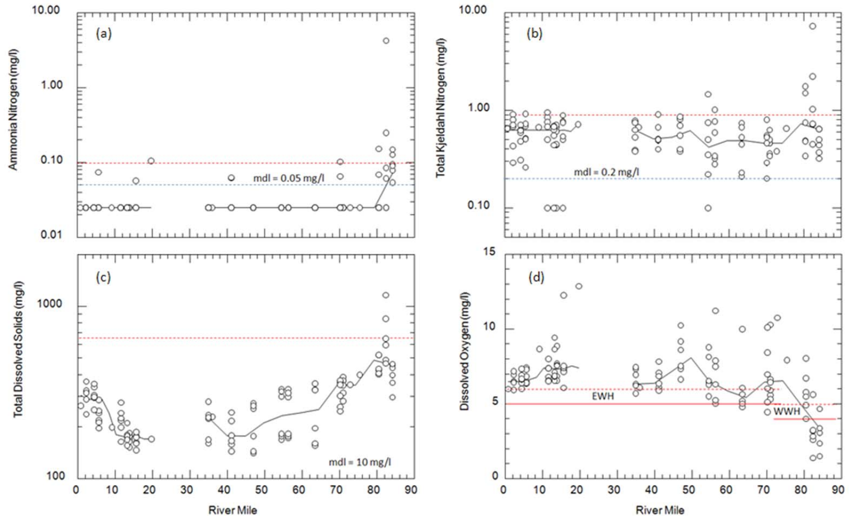
Figure 18. Longitudinal profiles of (a) ammonia nitrogen, (b) total Kjeldahl nitrogen, (c) total dissolved solids, and (d) dissolved oxygen measured in samples collected from the East Fork Little Miami River, 2012. Dashed red lines in plots (a), (b) and (c) suggest elevated levels. The blue lines in (a) and (b) indicate analytical detection limits. The red lines in (d) depict water quality criteria: dashed lines are 24 h average criteria, solid lines are instantaneous.
