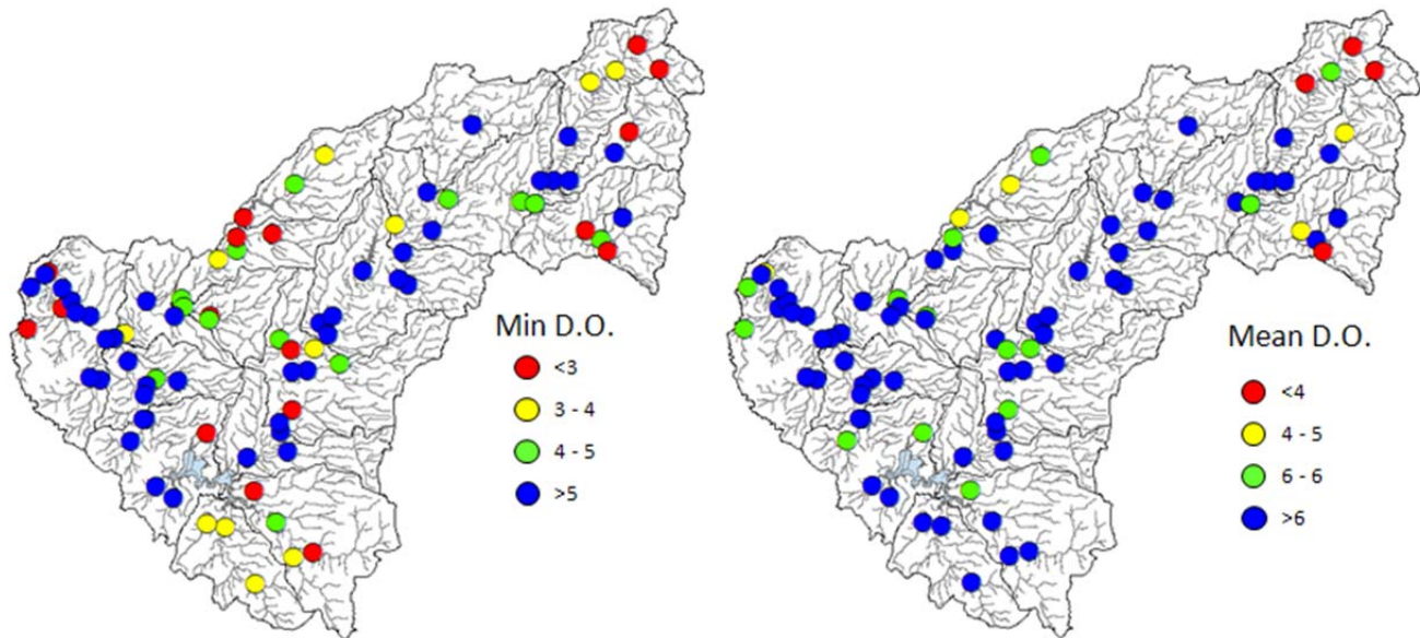
Figure 16. Minimum and mean field dissolved oxygen concentrations measured during the 2012 survey of the East Fork Little Miami River basin.
