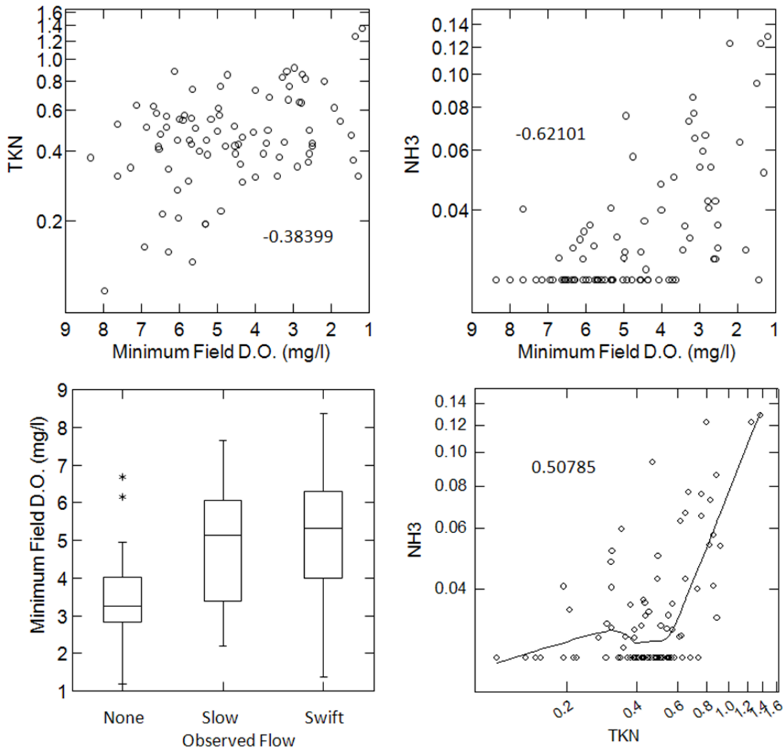
Figure 30. Top row: relationships between minimum dissolved oxygen concentrations measured during the field survey and TKN and NH3-N. Bottom row: distributions of minimum dissolved oxygen concentrations binned by categorical levels of observed flow, and the relationship between TKN and NH3-N. Data are from Cluster Groups 21 and 25.
