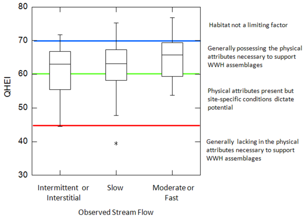
Figure 21. Distributions of QHEI scores for East Fork LMR tributaries sampled in the 2012 survey plotted by observed stream flow, and in relation to broadly functional narrative ranges.
