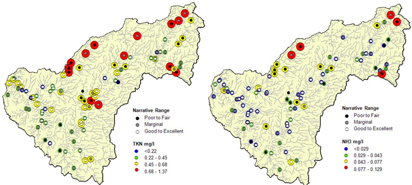
Figure 35. Overlays of macroinvertebrate assemblage ratings on total Kjeldahl nitrogen and ammonia nitrogen concentrations for sites sampled in the East Fork LMR basin, 2012. Compare these plots with those in Figure 29.
