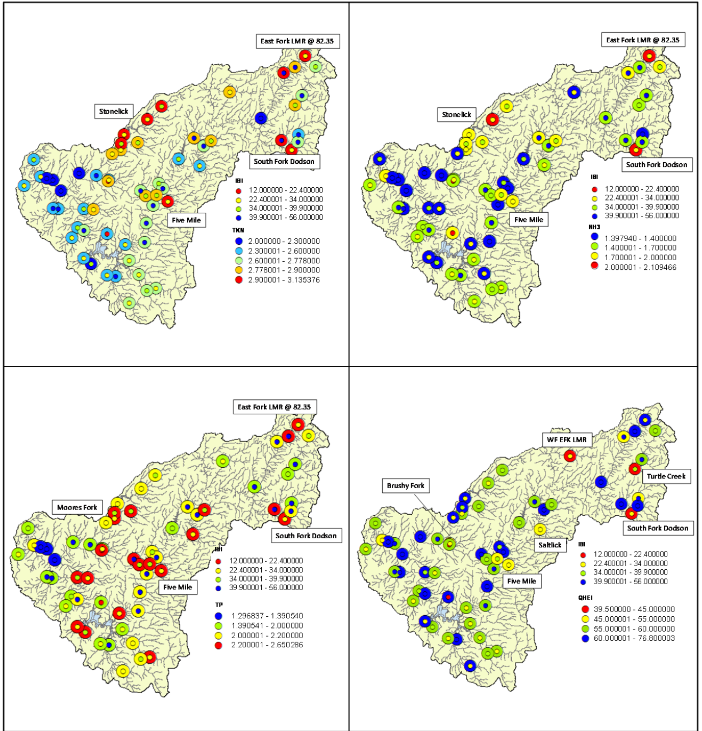
Figure 29. Overlays of IBI scores on (from left to right) total Kjeldahl nitrogen, ammonia nitrogen, total phosphorus and QHEI scores. Selected sites with one or more elevated indicators are labeled.
