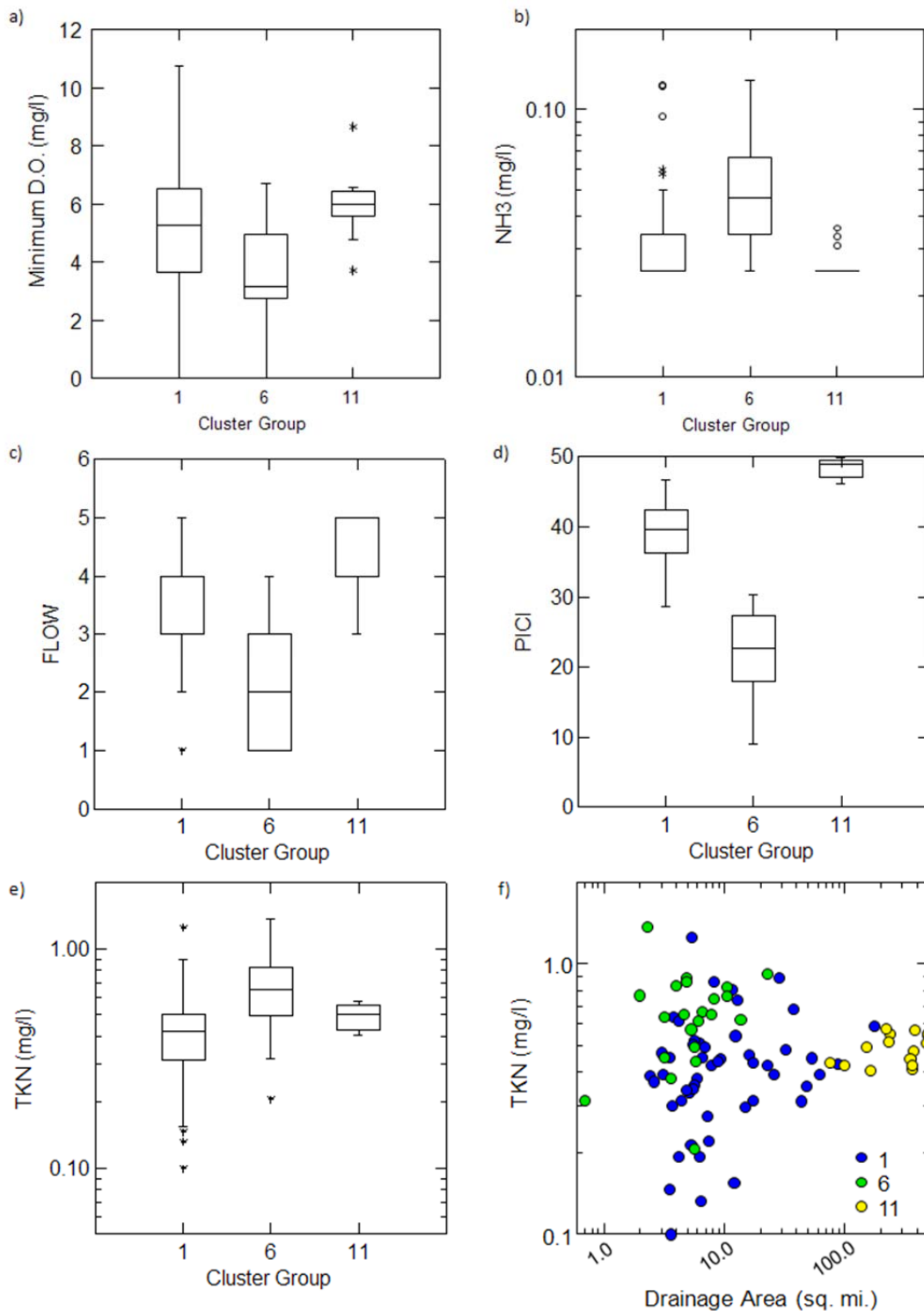
Figure 34. Distributions of a) minimum D.O. concentrations, b) mean ammonia concentrations, c) categorical levels of flow (1- no flow to 5 fast flow), d) an index of macroinvertebrate assemblage condition based on qualitative metrics (PICI), and e) average TKN concentrations within groups identified by hierarchical cluster analysis. Plot f) shows the relationship between mean TKN concentrations and drainage area for sites sampled in the East Fork LMR basin. Sites are color-coded by hierarchical cluster groups.
