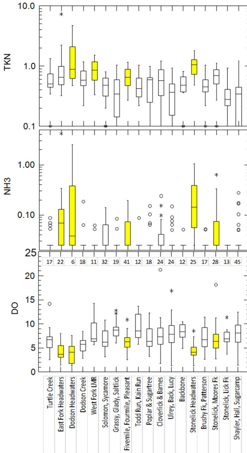
Figure 15. Distributions of total Kjeldahl nitrogen, ammonia nitrogen and dissolved oxygen stratified by 12-HUCs within the East Fork LMR basin. Yellow-shaded boxes show distributions containing values that are potentially stressful to aquatic life. Data from the East Fork mainstem downstream from Fayetteville are excluded.
