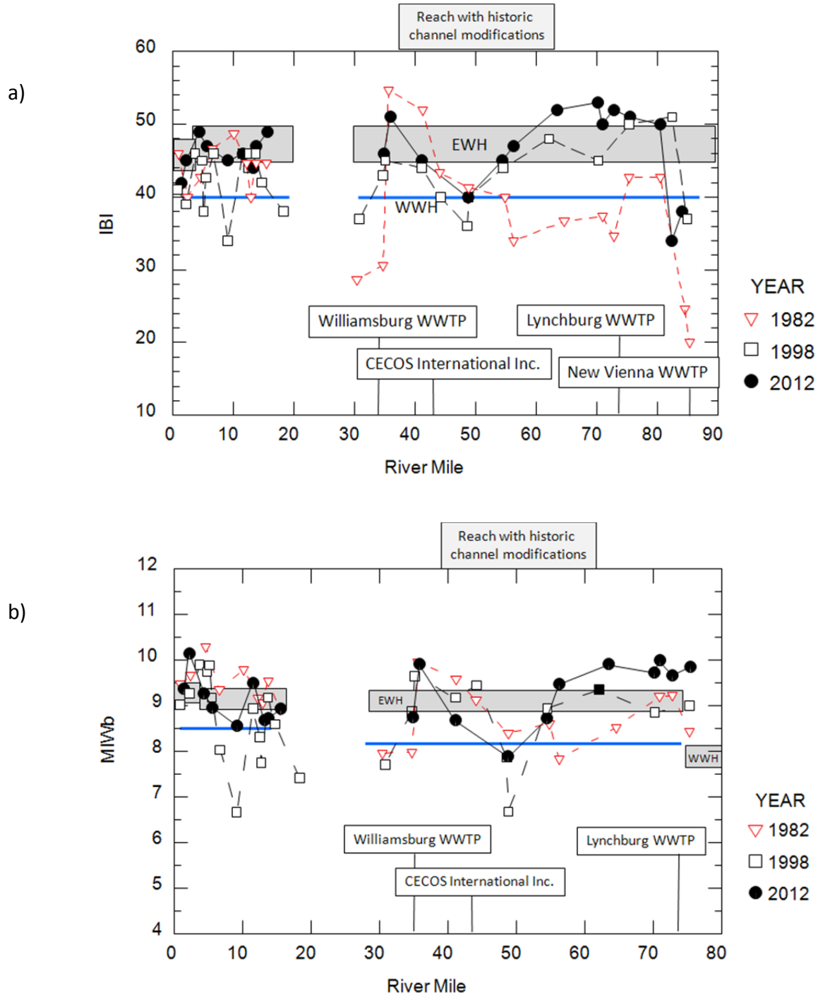
Figure 31. Longitudinal plots of (a) IBI and MIwb (b) scores by river mile for the East Fork Little Miami River mainstem, 1982, 1998 and 2012. Existing biocriteria are noted by the gray-shaded horizontal bars. The WWH biocriteria are shown by blue lines for perspective. Locations of permitted dischargers for the reach upstream from Harsha Lake are annotated along the x-axis (see Figure 32 for detail of the reach downstream from Harsha Lake).
