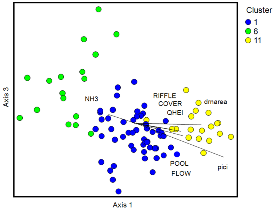
Figure 33. Sites sampled in the East Fork Little Miami River arrayed by two axes derived from an ordination 15 of assemblage attributes. The color-coded groupings were defined by hierarchical cluster analysis. Environmental measures correlating with Axis 1 ( r^2 > 0.3 ) are superimposed on the plot (the length of the superimposed lines show relative degree of correlation). The variable “PICI” is an indicator of macroinvertebrate assemblage quality based on assemblage attributes from qualitative samples that lack ICI scores. The “PICI” correlates well with the ICI 16 (also, n.b. , the correlation between “PICI” and Axis 1 is 0.89).
