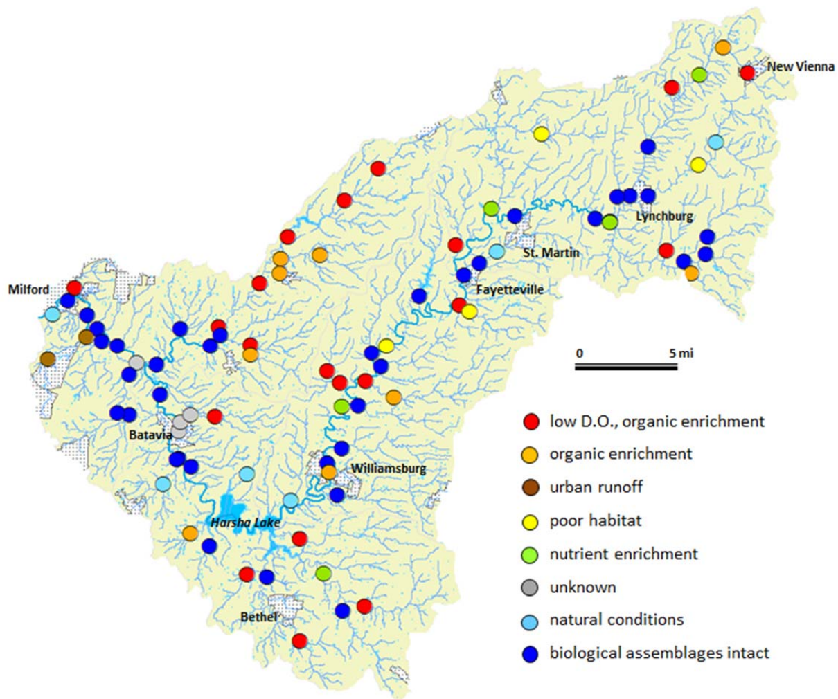
Figure 1. Locations sampled during the 2012 East Fork Little Miami River survey color-coded to condition status as arrayed by the most proximate cause (where applicable) of impairment ( n.b. , low dissolved oxygen is typically a manifestation of organic enrichment, whereas organic enrichment is a more encompassing source of stress).
