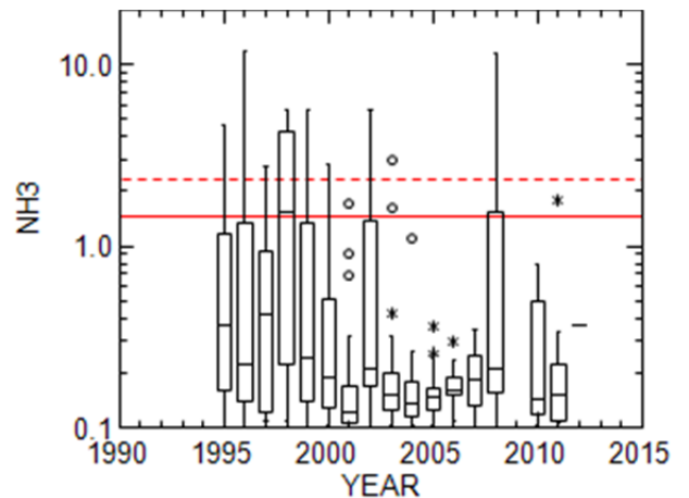
Figure 12. Distributions of third quarter ammonia nitrogen concentrations measured in the Middle East Fork WWTP effluent 1995-2012 in relation to weekly (dashed red line) and monthly (solid red line) permit limits.
