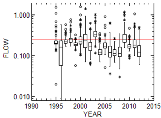
Figure 11. Distributions of third quarter flows from the Batavia WWTP 1995-2012 in relation to the average design flow (0.236 mgd, red line in plot).
