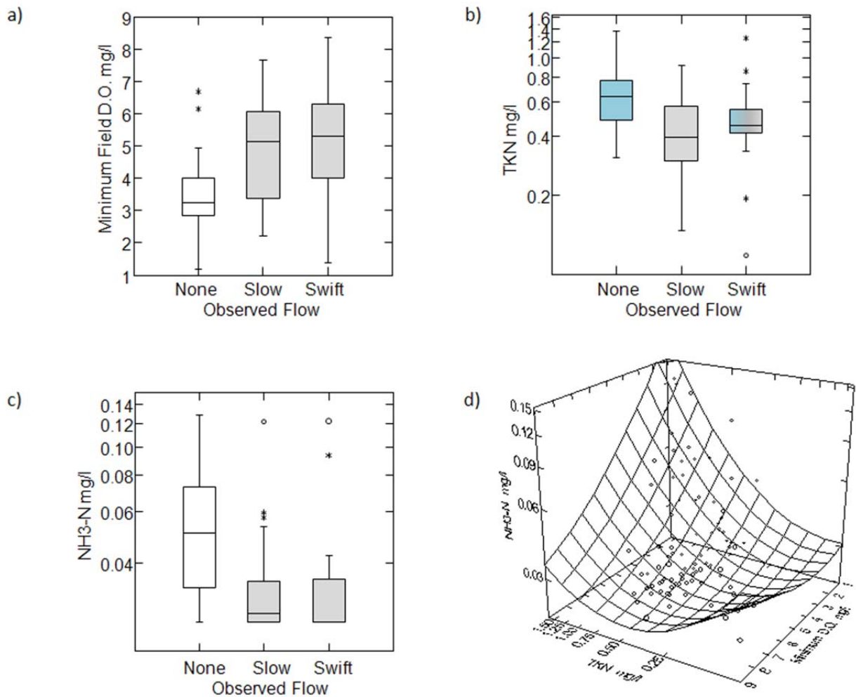
Figure 14. Distributions of (a) minimum field dissolved oxygen, (b) total Kjeldahl nitrogen (TKN) and (c) ammonia nitrogen (NH 3 -N) in relation to categorical levels of observed stream flow, and (d) a 3-dimensional scatter plot of the relationship between minimum dissolved oxygen, TKN and NH 3 -N. In this representation, 61% of the variance in NH 3 -N is explained. Data are from sites sampled in the East Fork LMR, 2012.
