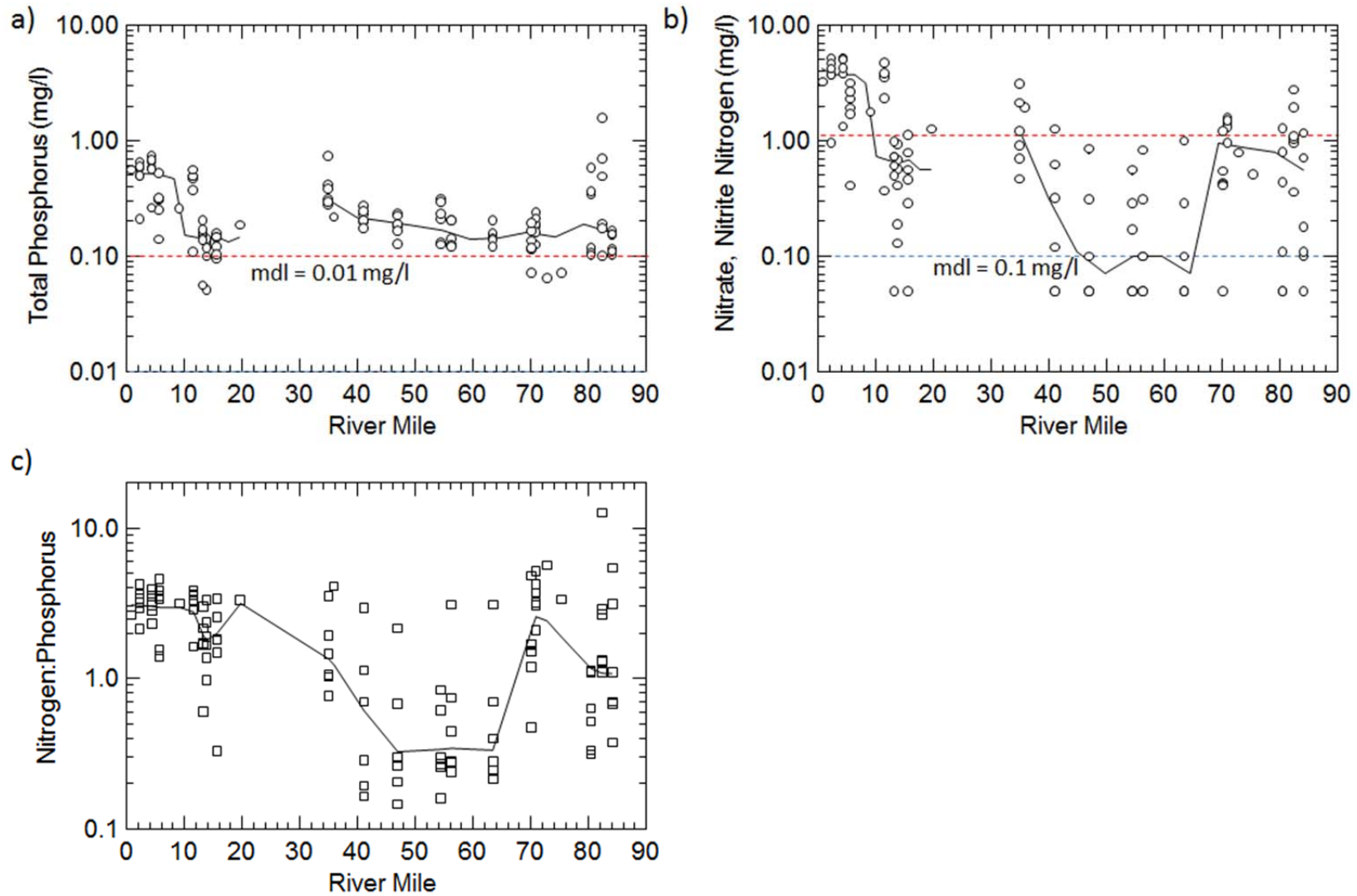
Figure 19. Longitudinal profiles of (a) total phosphorus and (b) nitrate, nitrite nitrogen measured in water samples collected from the East Fork Little Miami River, 2012. Dashed red lines in plots (a) and (b) suggest elevated levels, and the blue lines indicate analytical detection limits. Nitrogen to phosphorus ratio are given in (c); note the strong tendency towards nitrogen limitation.
