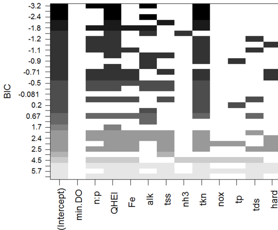
Figure 27. Graphical representation of all-subsets regression between IBI scores and the parameters listed on the x-axis for sites included in Cluster 21. The y-axis shows the Bayesian Information Criterion (BIC). The most parsimonious models are those that include the fewest explanatory variables (x-axis) and have the lowest BIC value (e.g., TKN as a single explanatory variable is the most parsimonious, though that model may not necessarily have the highest explanatory power). Visual inspection of the overall pattern of sequences, along with inspecting the differences in explanatory power of suggested models (e.g., the TKN only model compared to the TKN+QHEI+ALK+N:P model) helps to gauge the influence of collinearity, and whether additional explanatory variables are making a significant or marginal contribution.
