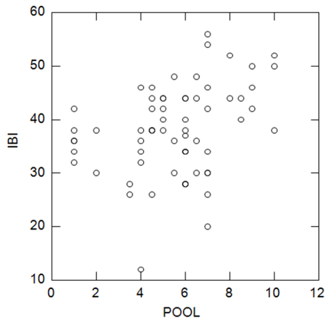
Figure 22. Fish Index of Biotic Integrity (IBI) scores plotted by pool metric scores. East Fork LMR tributaries, 2012.
