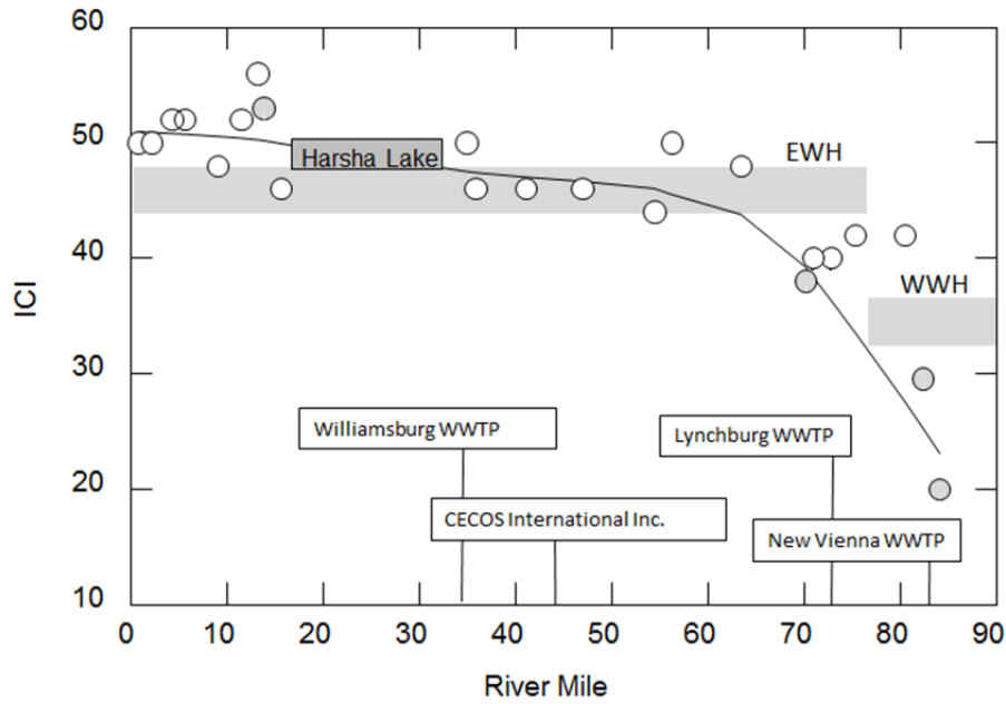
Figure 36. ICI scores plotted by river mile for the East Fork Little Miami River, 2012, in relation to publicly owned treatment works and Harsha Lake. Gray-shaded regions of the plot denote the range of non-significant departure from the given biocriterion. Shaded points were given numeric scores based on narrative assessments.
