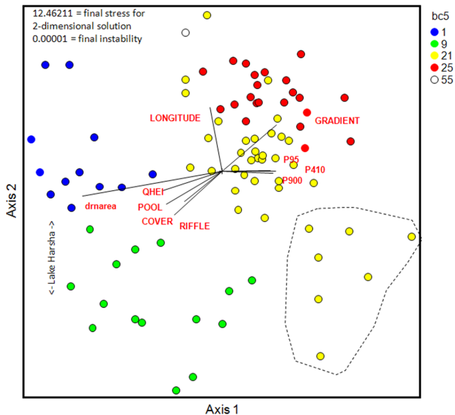
Figure 23. An ordination of fish assemblages sampled from the East Fork Little Miami River basin, 2012. Axis scores were generated by Nonmetric Multidimensional Scaling based on Bray-Curtis distances. Points are color coded to groups suggested by hierarchical clustering using Bray-Curtis distances and linking via the flexible beta method (McCune and Grace 2002). Environmental variables correlating with axes scores are shown as an overlay, with the relative strength of association (minimum R^2=0.3 ) being represented by the length of the respective overlay lines.
