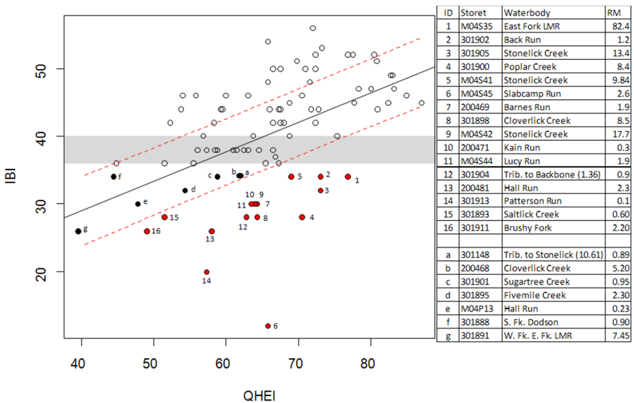
Figure 2. Index of Biotic Integrity (IBI) scores plotted on Qualitative Habitat Evaluation Index (QHEI) scores for sites sampled in the East Fork Little Miami River basin, 2012. The solid line is from ordinary least squares regression, and the dashed red lines show the 50 th percentile prediction intervals (PI). Points falling below non-significant departure of the WWH biocriterion (gray-shaded region) are color-coded according to proximity to the lower PI. Red points are likely stressed beyond limitations imposed by local habitat quality; black-filled points are primarily limited by local habitat quality. Note that Slabcamp Run (point 6) functions as a primary headwater stream.
