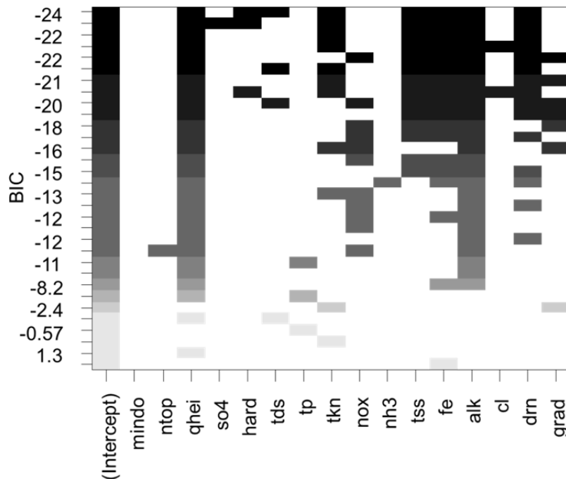
Figure 28. Graphical representation of all-subsets regression between IBI scores and the parameters listed on the x-axis for sites included in Cluster 25. The y-axis shows the Bayesian Information Criterion (BIC).
