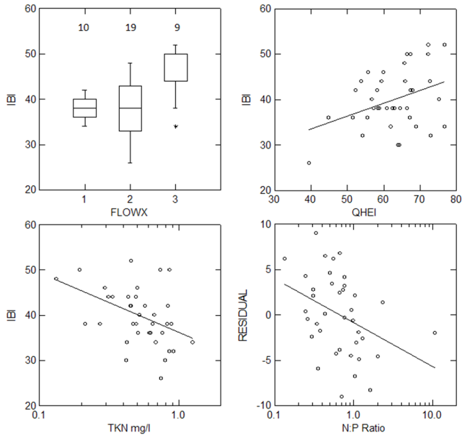
Figure 26. Graphical representation of relationships given by the ANCOVA model relating IBI scores to environmental variables for Cluster 21.
