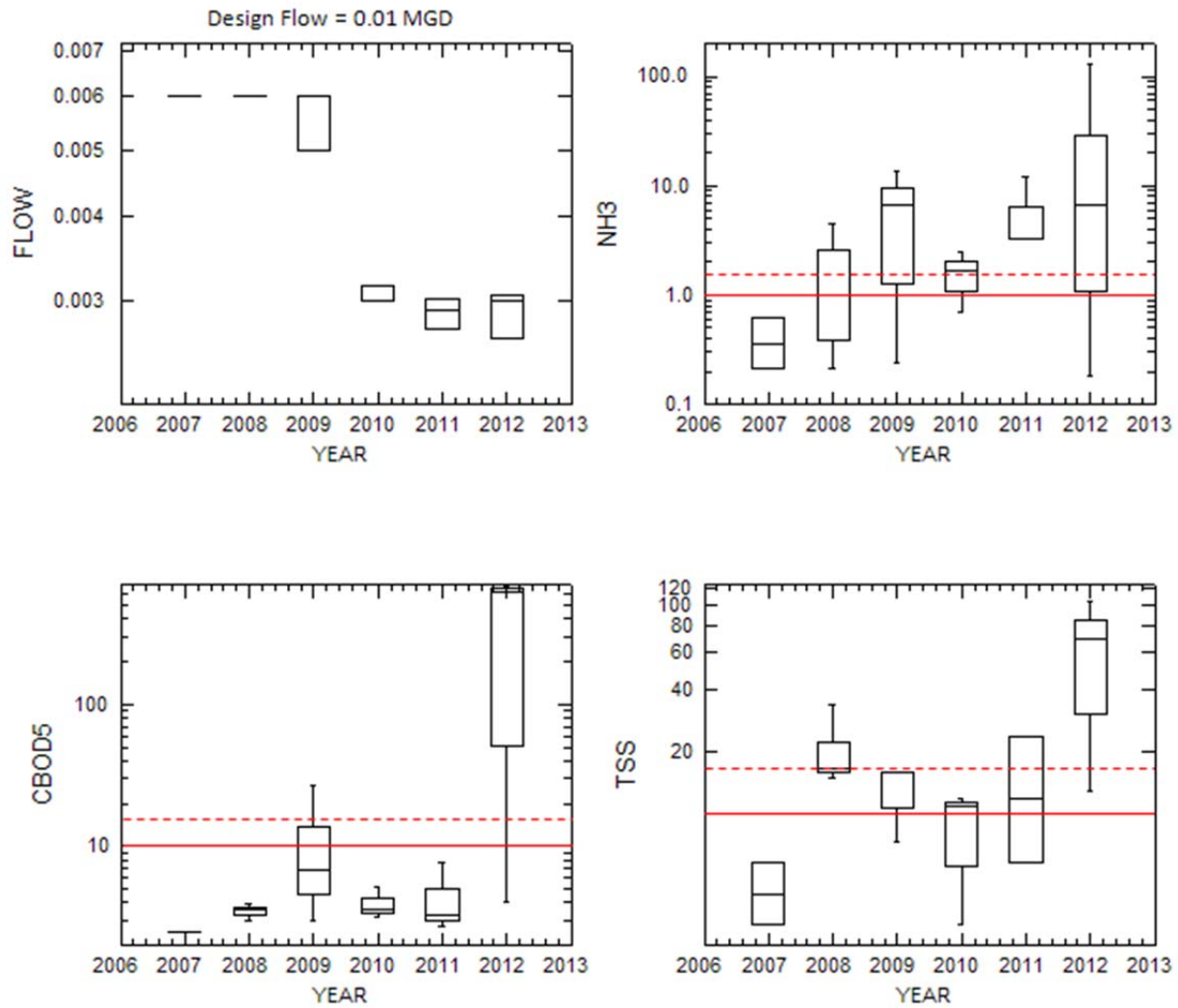
Figure 13. Third quarter plant flows and concentrations of ammonia nitrogen, CBOD5 and TSS reported by the Locust Ridge Nursing Home, 2007-2012. Note that samples reported for 2012 were for land-applied effluent. The plant was under construction in 2012 and did not discharge to Light Run.
