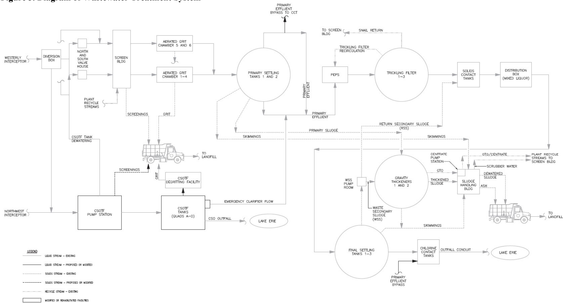
Figure 3. Diagram of Wastewater Treatment System
