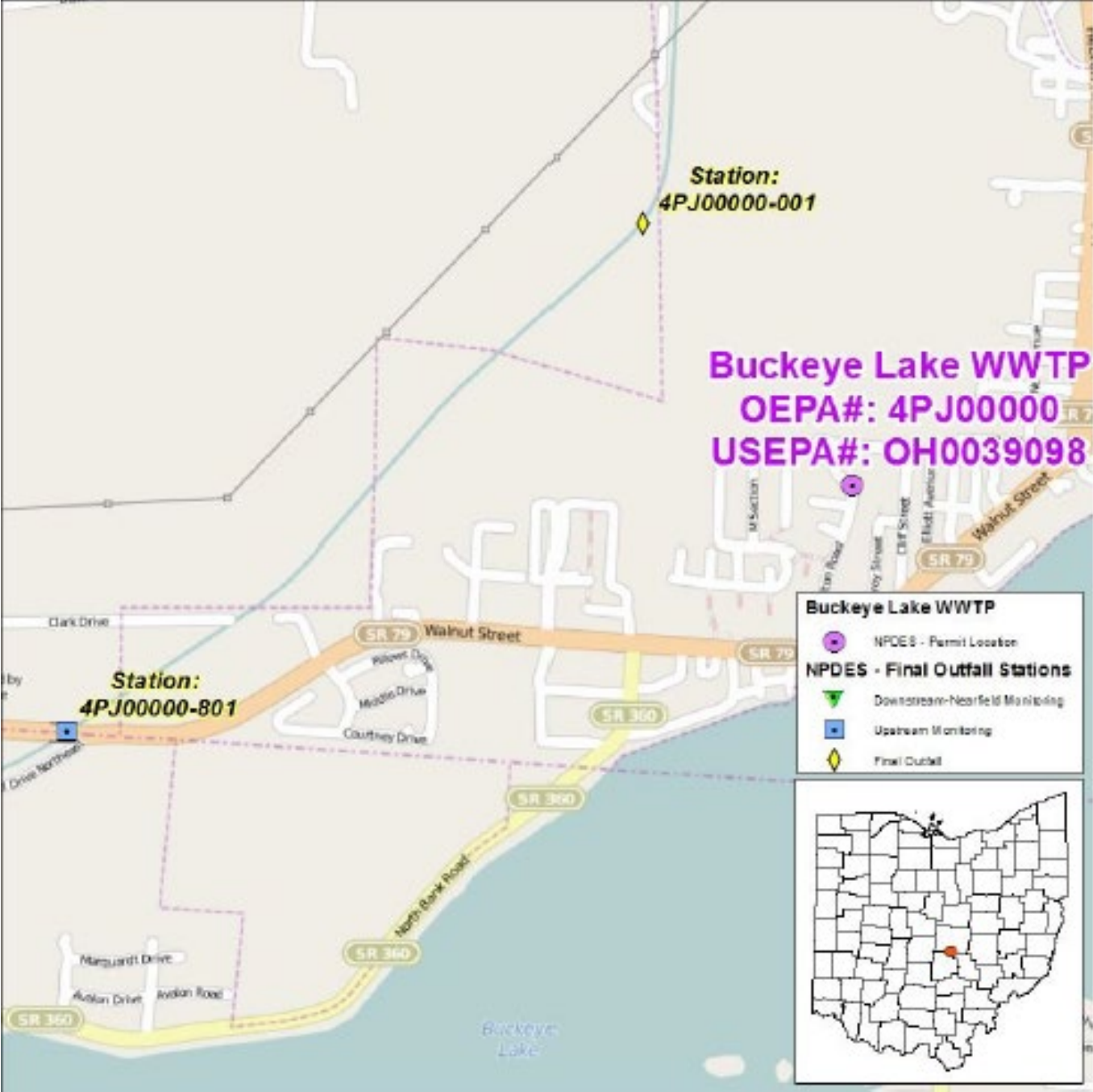
Figure 1. Location of Buckeye Lake WWTP
