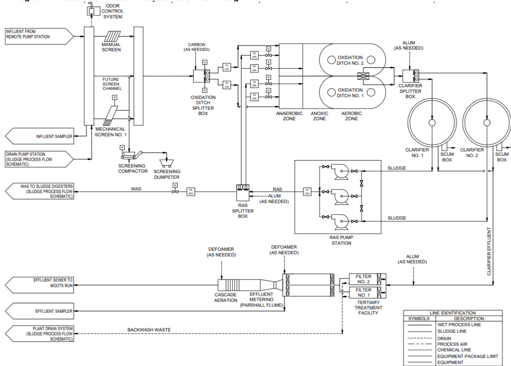
Figure 2. Diagram of Wastewater Treatment System at 3 MGD Design
