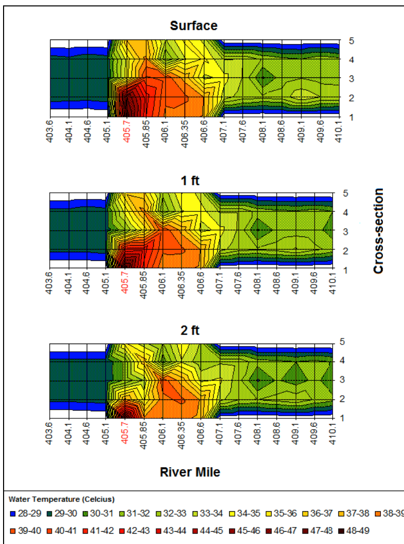
Figure 4. Temperature gradient observed on 8/09/07 in the vicinity of the J. M. Stuart discharge (ORM 405.7) at the surface, 1 ft and, 2 ft depth contours. Temperature gradients are shown in 1°C increments (colors labeled). Cross-section refers to locations where temperature data was collect (1 = Ohio shore 5 ft contour, 3 = mid-channel, 5 = Kentucky shore 5 ft contour). Water flow is from left to right.
