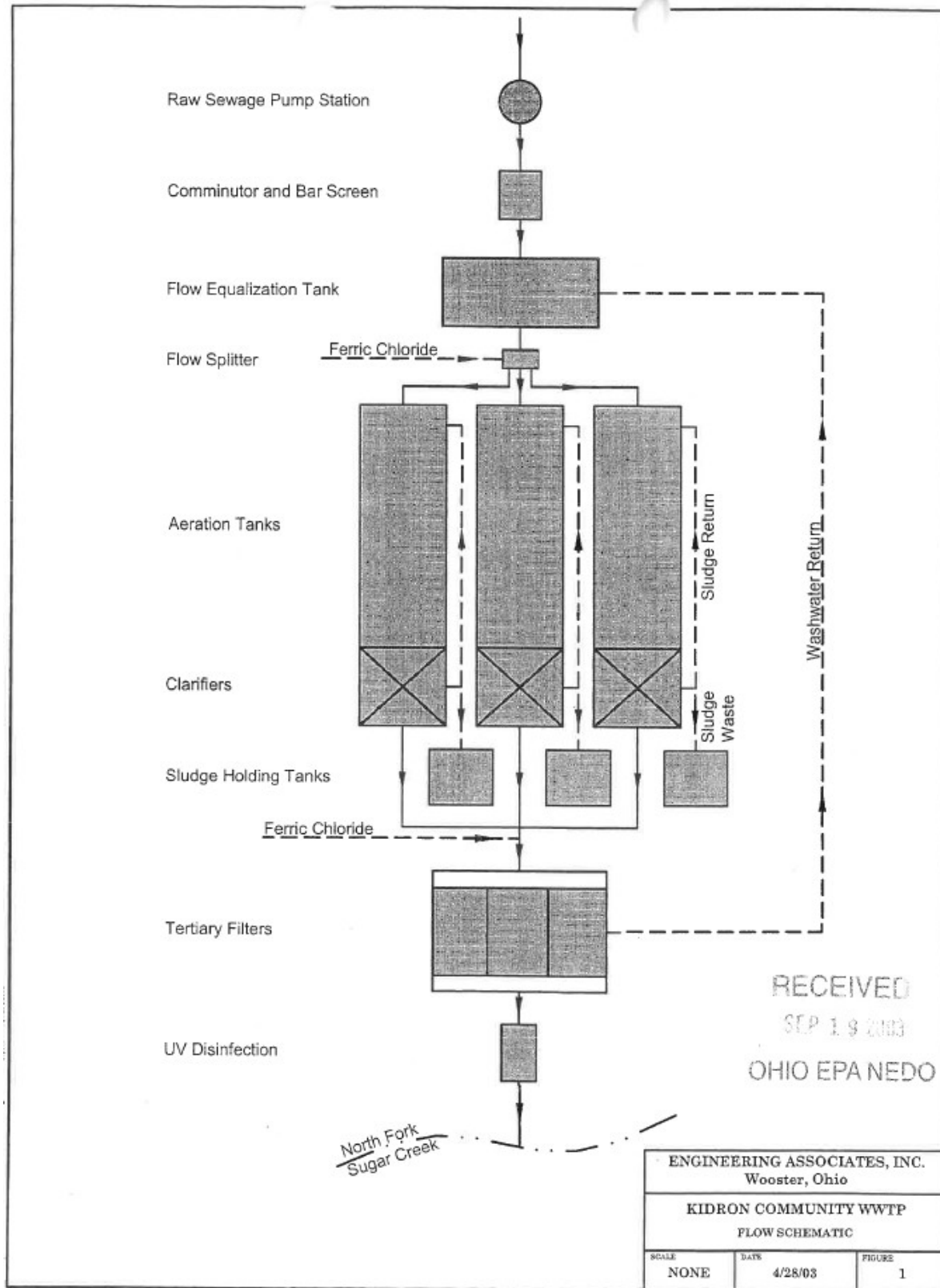
Figure 2. Kidron WWTP Schematic
