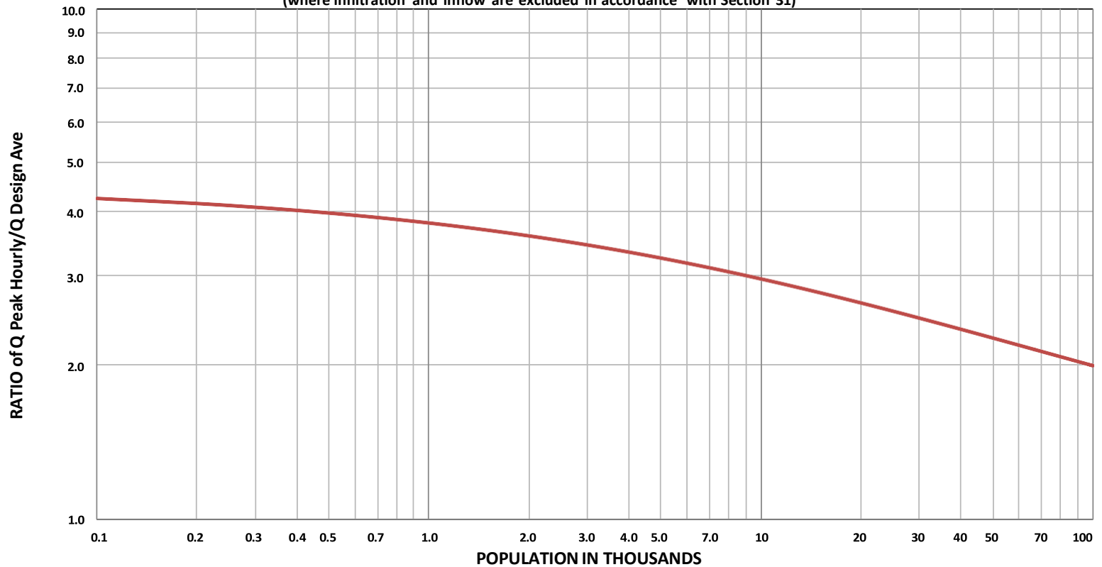
FIGURE 1 RATIO OF PEAK HOURLY FLOW TO DESIGN AVERAGE FLOW (where infiltration and inflow are excluded in accordance with Section 31)
