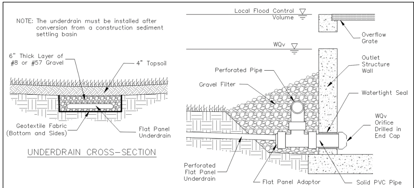
Figure 2.7.3 Dry Extended Detention Basin Outlet with Underdrain (after Delaware County Engineer)
