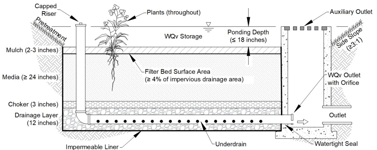
Figure 2.9.1 Schematic Sections of Bioretention (not to scale)
