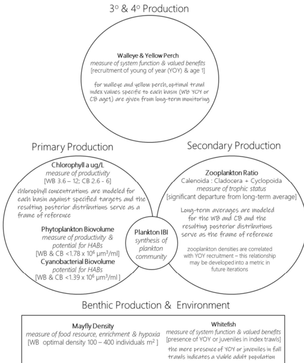
Figure I-3 – Schematic of the Lake Erie Aquatic Life Use and assessment framework.
