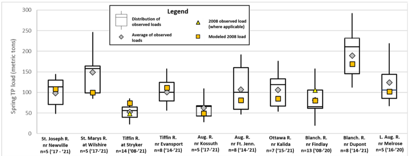
Figure 42. Model verification results. Box plots show the distribution (minimum: bottom of lower tail, 25th percentile: bottom of box, median: middle of box, 75th percentile: top of box, and maximum: top of upper tail) of observed spring season total phosphorus loads for all spring seasons with data available for each monitoring gage since 2008. Number of seasons and the years of available data are listed below the label for each gage. The gray diamonds show the average observed spring season load. Yellow triangles show the observed 2008 spring load for two stations where monitoring was active that year. The orange boxes show the TMDL existing, spring 2008, mass balance modeled results broken out to each of these monitoring stations.
