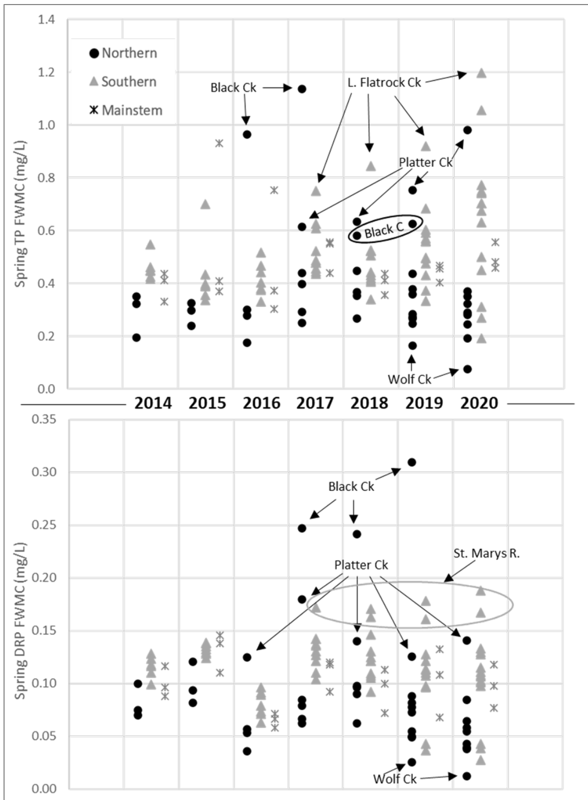
Figure 40. Total phosphorus (top) and dissolved reactive phosphorus (bottom) spring FFWMCs for all Maumee watershed monitoring stations with available water quality data for 2014–2020. Stations north and south of the Maumee River mainstem and stations on the mainstem are shown with different symbols. Not all stations have available data for each year.
