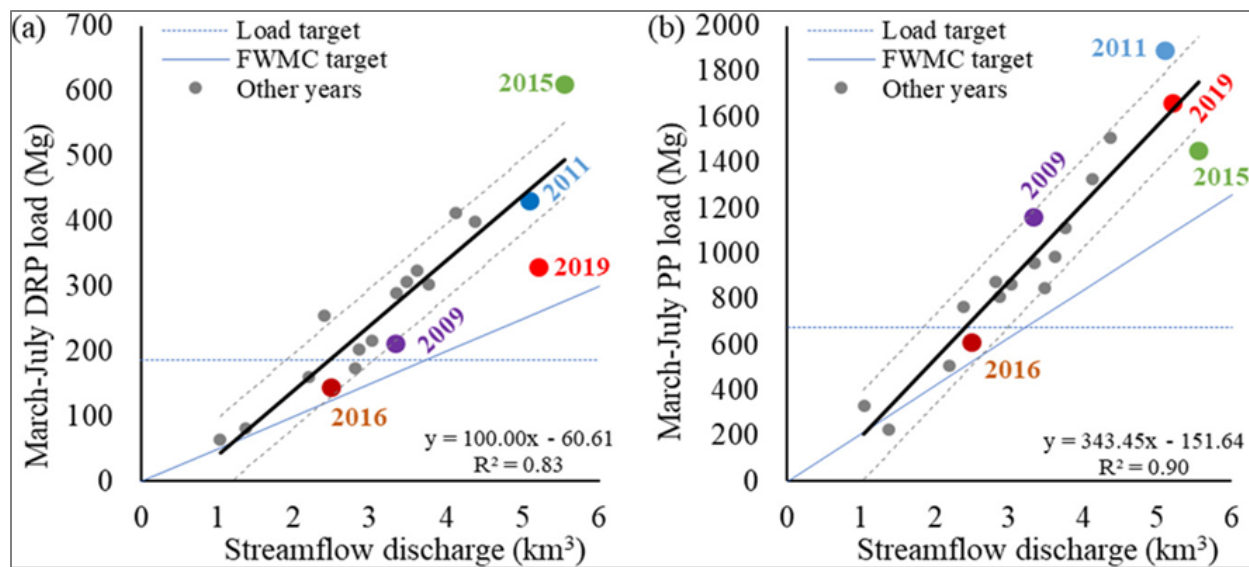
Figure 10. DRP load (a) and participate phosphorus (b) plotted against Maumee River “spring” loading season streamflow discharge showing results from 2002–2019, with several years labeled. The bold black lines show the linear relationship between load and discharge, with dashed gray lines showing 95th confidence intervals of that relationship. Other lines represent various target conditions (Guo et al., 2021).
