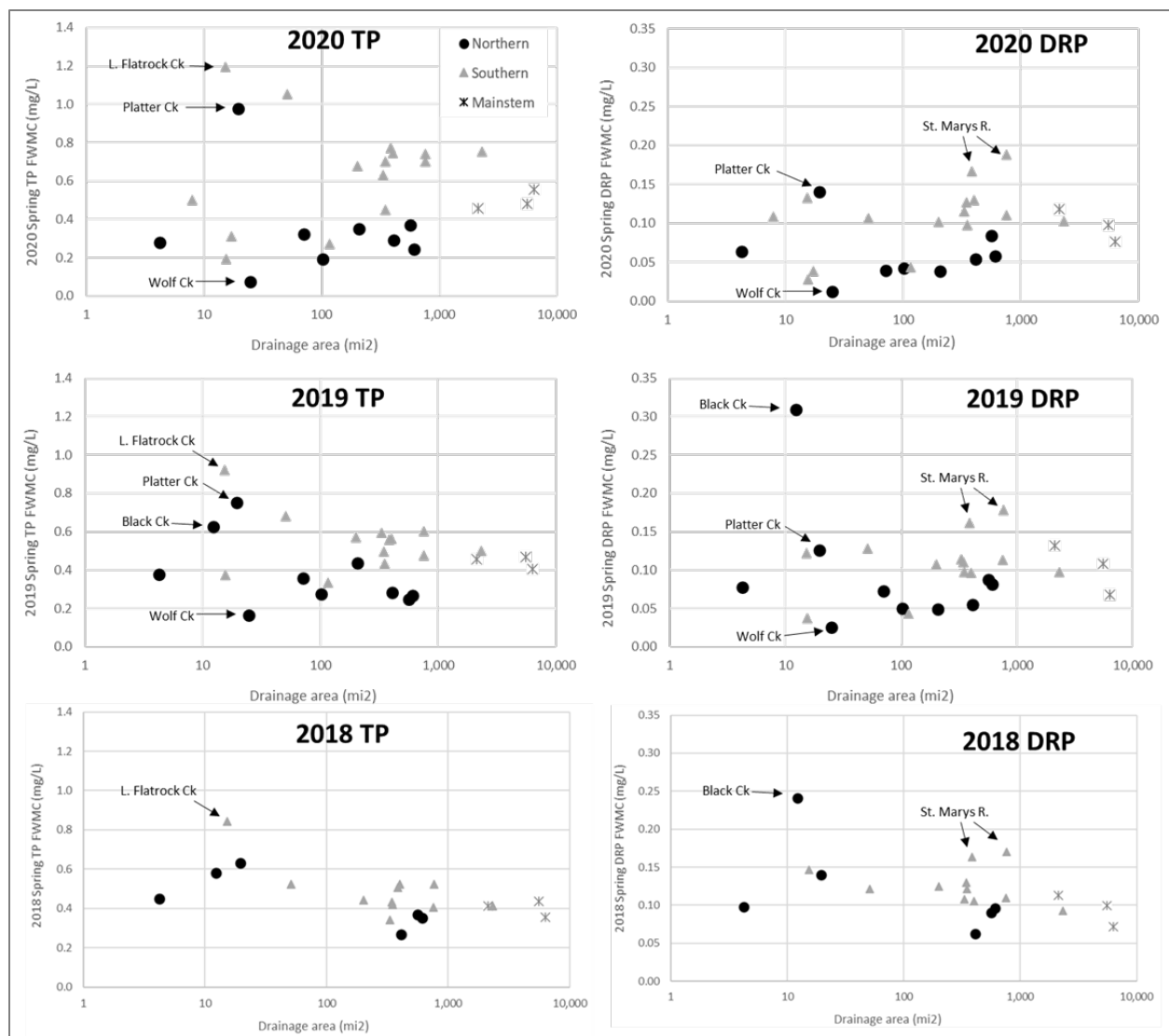
Figure 39. Total phosphorus (left) and dissolved reactive phosphorus (right) FWMCs for three different years plotted against monitoring station drainage area. Stations north and south of the Maumee River mainstem and stations on the mainstem are shown with different symbols. Not all stations have available data for each year.
