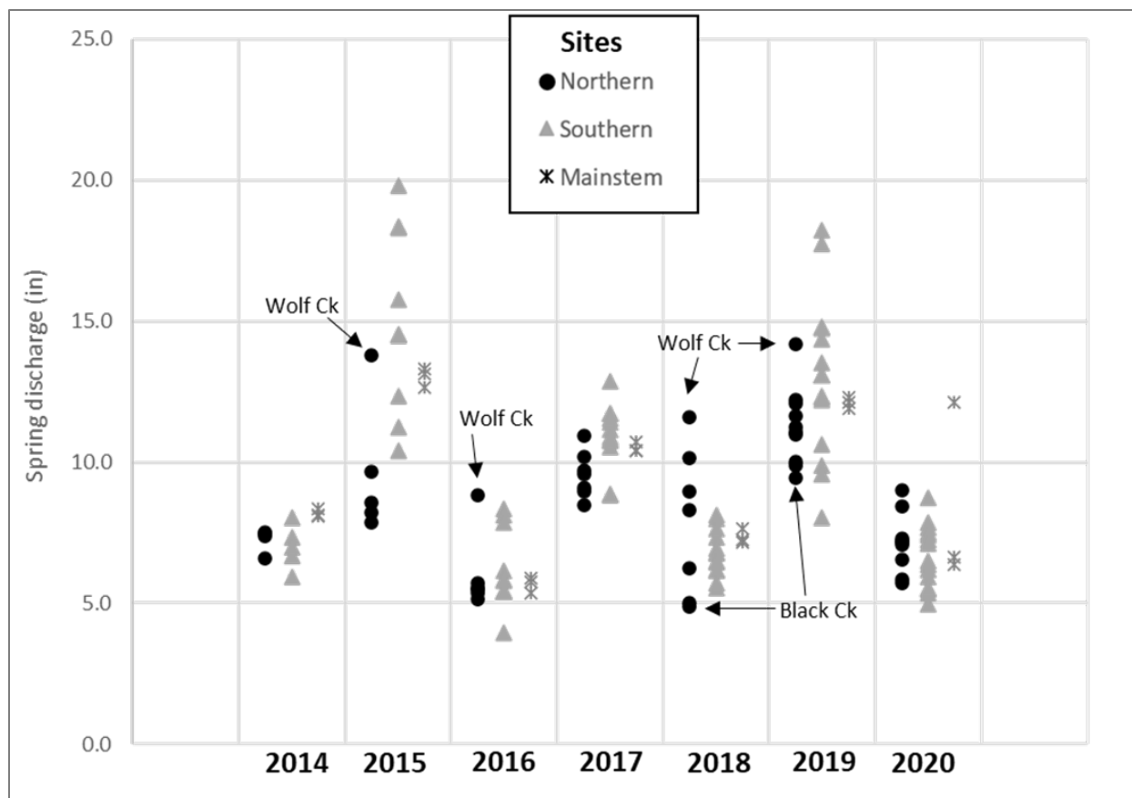
Figure 38. Spring stream discharge water yield for all Maumee watershed monitoring stations with available water quality data for 2014–2020. Stations north and south of the Maumee River mainstem and stations on the mainstem are shown with different symbols. Not all stations have available data for each year.
