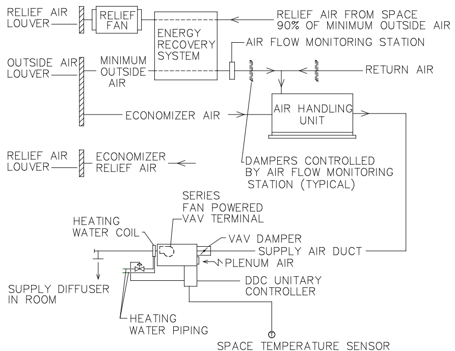
Series Fan Powered VAV Schematic Figure C-1
