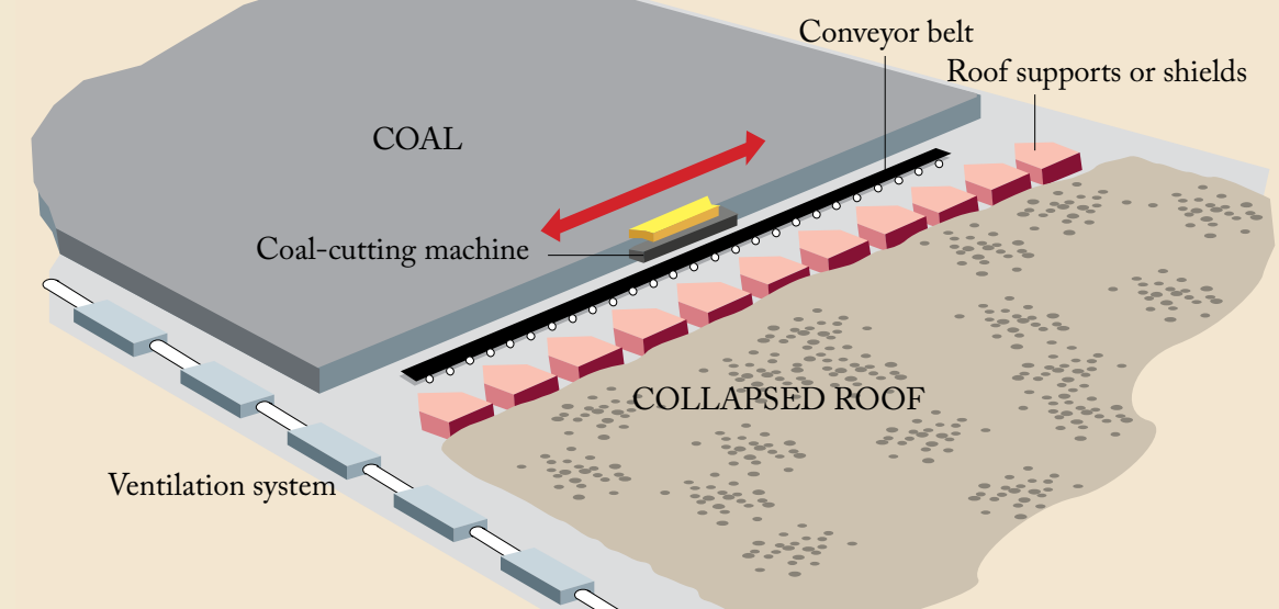
Figure 3—Longwall underground-mining method. In a longwall mine, a cutting machine moves back and forth across a panel of coal that can be up to 1,500 feet in width and 7,000 feet in length. The cut coal falls onto a flexible conveyor for removal. Hydraulic supports (shields) hold up the mine roof and protect the workers, and cutting machinery is advanced as the coal is cut. The roof in the mined-out area falls as the shields advance. (Graphic from The Columbus Dispatch , 2006, used with permission.)
