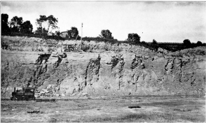
B.—View of the shale pit of the Medal Paving Brick Company near Wooster. Shale of the Black Hand member passes into sandstone near the top of the quarry face.
