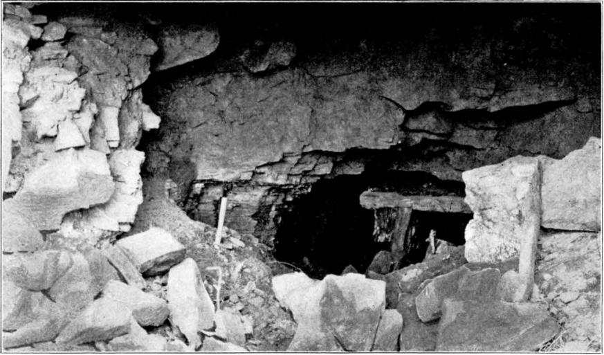
A.—A small drift mine in the Sharon or No. 1 coal on the north side of Chipewewa Valley. Note the sandstone roof.
