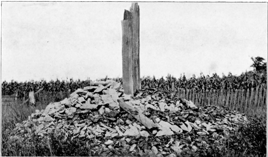
B.—Preparing a pile of limestone for burning. Note the alternate layers of coal and limestone.
