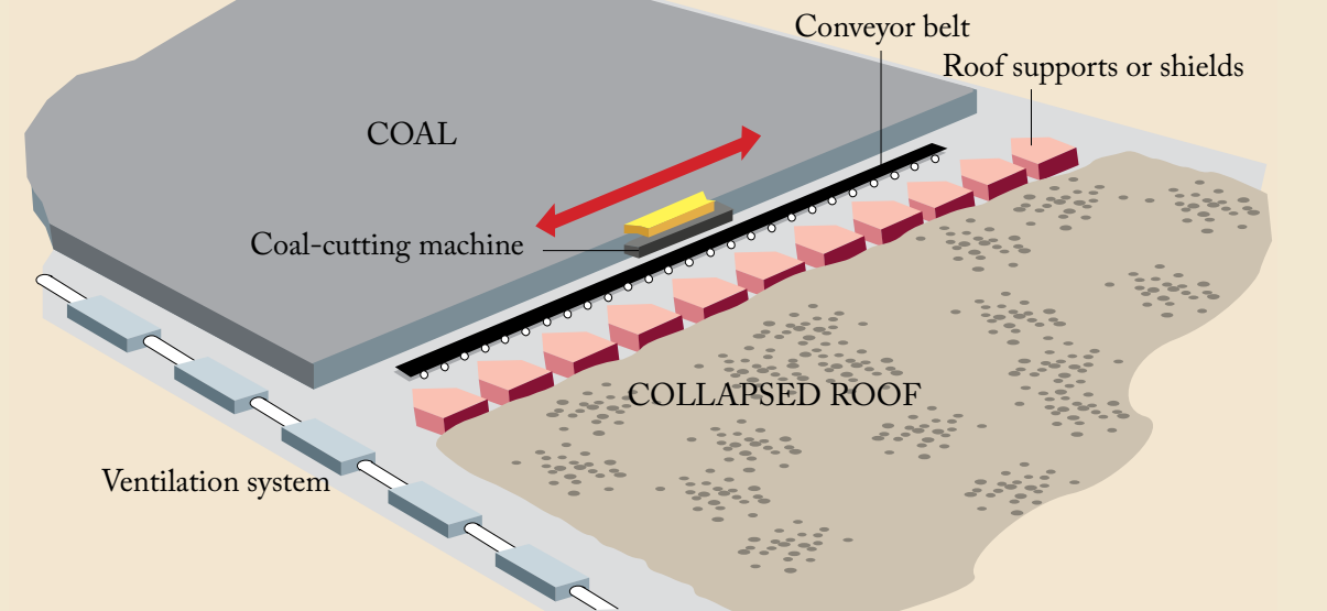
Figure 3.—Longwall underground-mining method. In a longwall mine, a cutting machine moves back and forth across a panel of coal that can be up to 1,100 feet in width and 7,000 feet in length. The cut coal falls onto a flexible conveyor for removal. Hydraulic roof supports (shields) hold up the mine roof and protect the workers and cutting machinery as advanced as the coal is cut. The roof in the mined-out area falls as the shields advance. (Graphic from The Columbus Dispatch , 2006, used with permission.)
