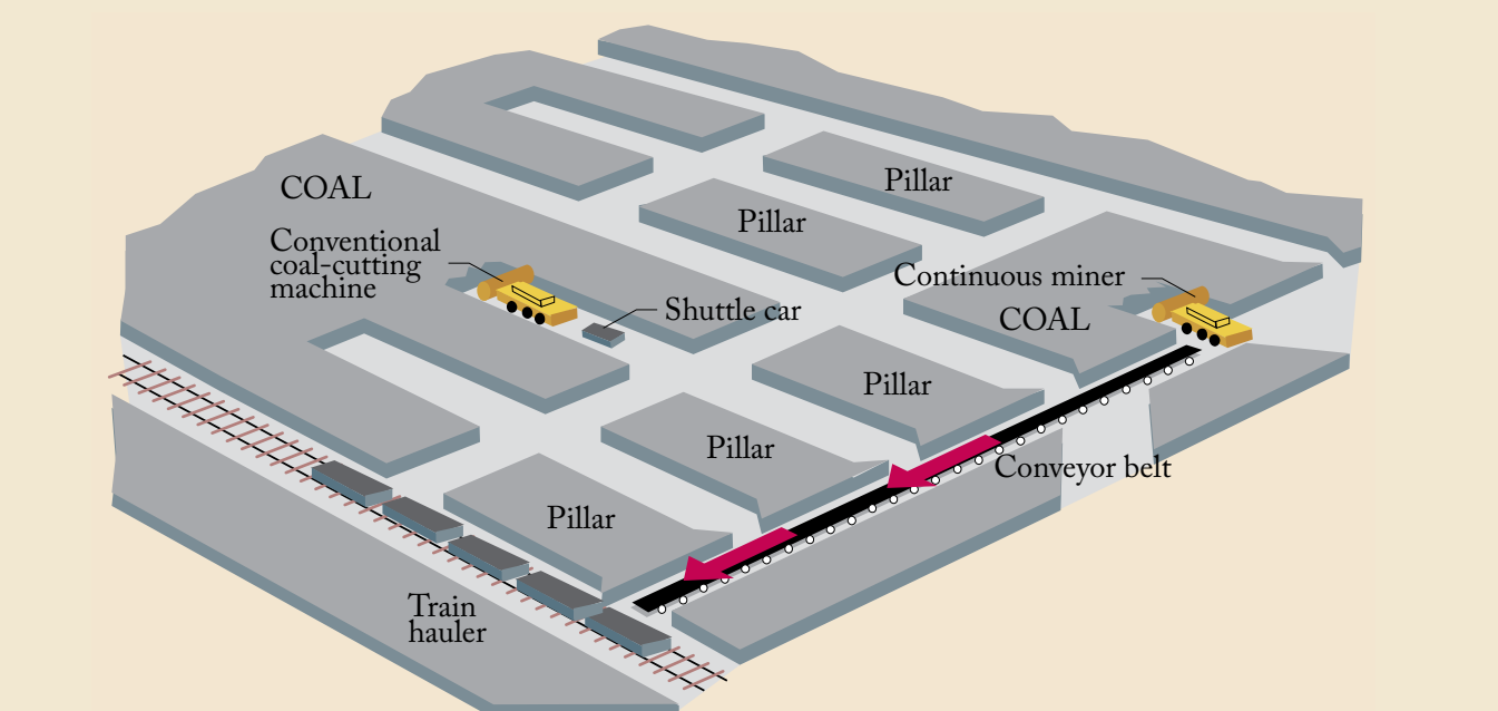
Figure 2.—Room-and-pillar underground mining method. In most older mines, the rooms were created by blasting and excavating the coal into shallow cuts that bailed coal to the surface. Most modern room-and-pillar mines use continuous-miner machinery to cut and directly feed the coal to a conveyor system that transports it to the surface. (Graphic from The Columbus Dispatch , 2006, used with permission.)
