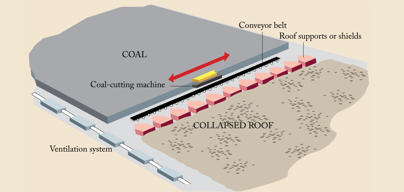
Figure 3.—Longwall underground mining method. In a longwall mine, a cutting machine moves back and forth across a panel of coal that can be up to 1,100 feet in width and 7,000 feet in length. The cut coal falls onto a flexible conveyor for removal. Hydraulic supports (shields) hold up the mine roof and protect the workers and cutting machinery as it advances as the coal is cut. The roof in the mined-out area falls as the shields advance. (Graphic from The Columbus Dispatch , 2006, used with permission.)
