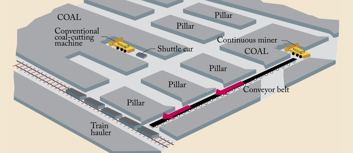
Figure 2—Room-and-pillar underground mining method. In most older mines, the rooms were created by blasting and excavating the coal into shuttle cars that hauled coal to the surface. Most modern room-and-pillar mines use continuous-miner machinery to cut and directly feed the coal to a conveyor system that transports it to the surface. (Graphic from The Columbus Dispatch , 2006, used with permission.)
