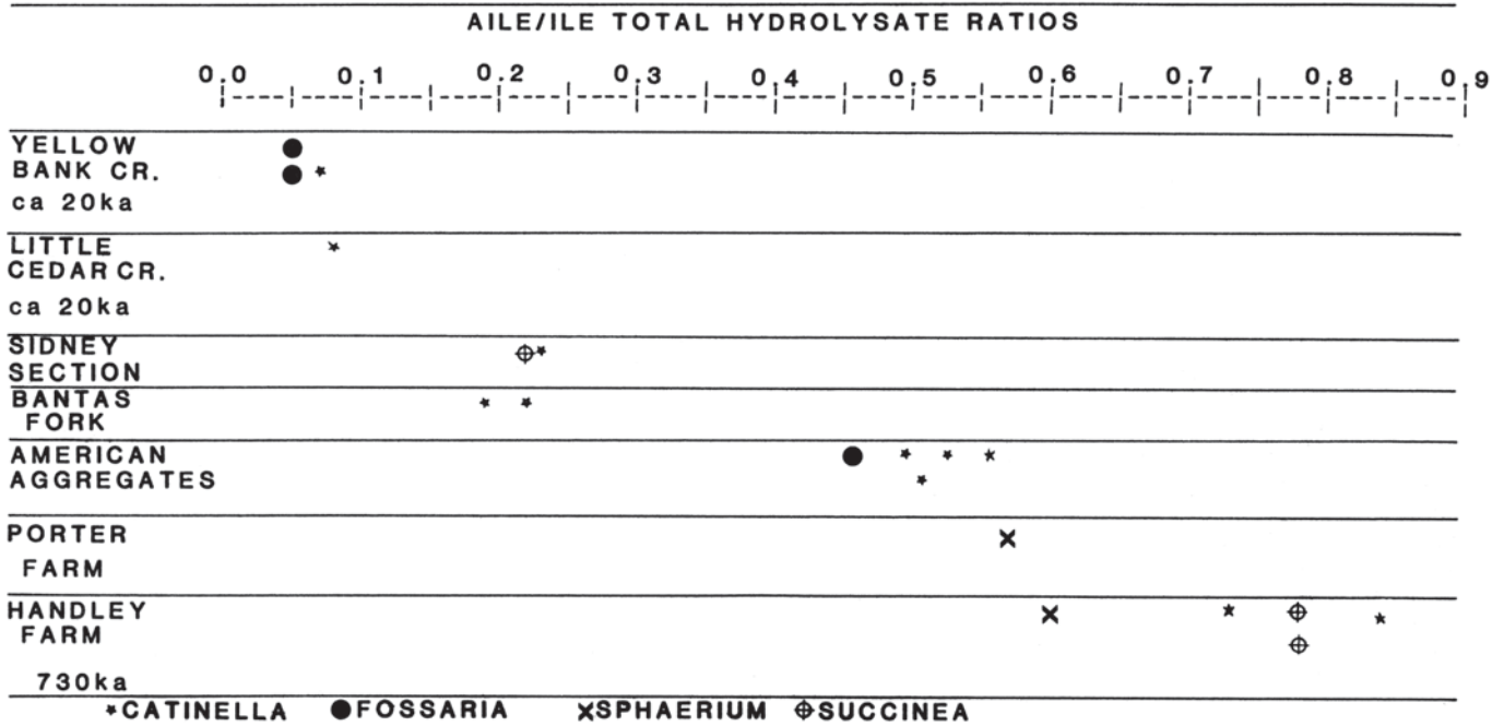
FIGURE 2.—Plot of aile/Ile ratios from samples in study area (see table 2).
