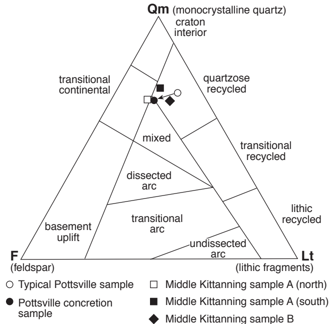
FIGURE 5.—Variations of interpreted source terrane from thin sections containing different cements (after Dickinson, 1985). Note the difference between the Pottsville carbonate concretion and the typically cemented Pottsville samples. The Middle Kittanning samples A and B are separated by only 0.05 meter. The two analyses for sample A were made within a concretion (north) and directly outside a concretion (south).
