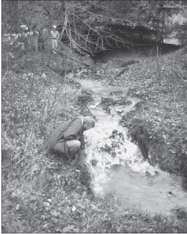
FIGURE 25.—Opening and discharge point of the Essex Mine, Hocking County, Ohio.
