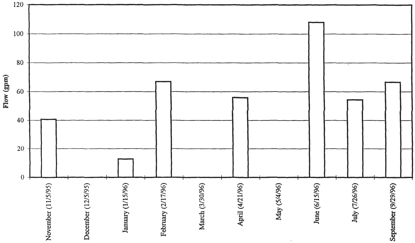
FIGURE 43.—Monthly ground-water influx into Rock Run, calculated as a residual of measurable flows.
