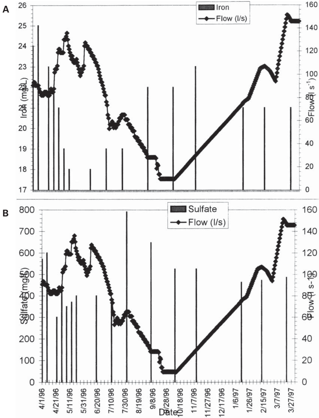
FIGURE 33.—Volumetric water flow and total iron (A) and total sulfate (B) concentrations (in mg/L) vs. time at the Essex Mine.
