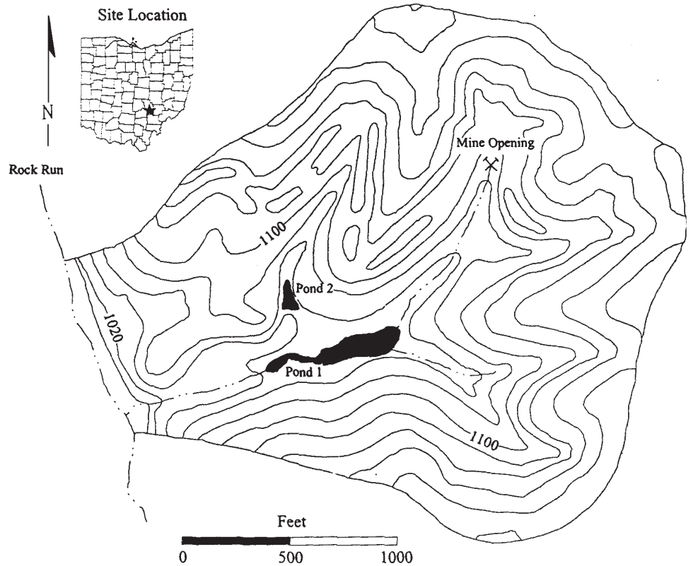
FIGURE 40.—Map of the watershed containing the Rock Run gob pile.
