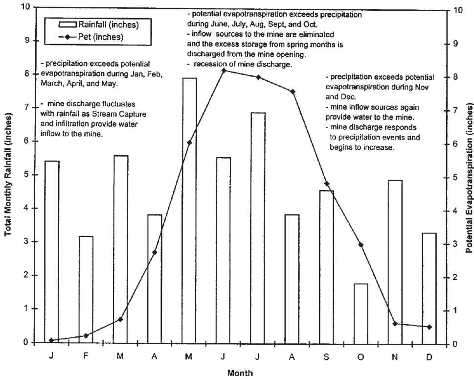
FIGURE 21.—Calculated potential evapotranspiration (Pet) and total monthly rainfall for the study area in 1996.
