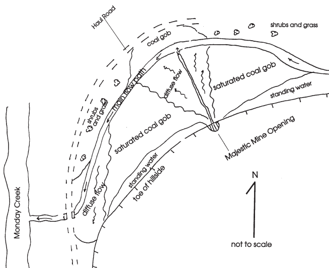
FIGURE 13.—Plan view of the Majestic Mine discharge area.
