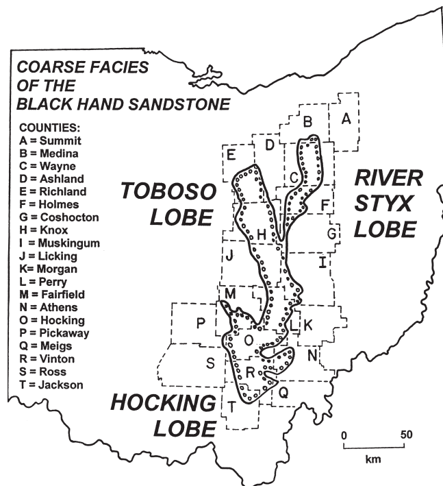
Figure 3-2.—Coarse facies of the Black Hand Sandstone, modified from Coogan and others (1981). The "Big Injun" lobe is present in the subsurface east of the River Styx lobe, approximately under the "River Styx" label (see figs. 22 and 29 in Szmuc, 1970).
