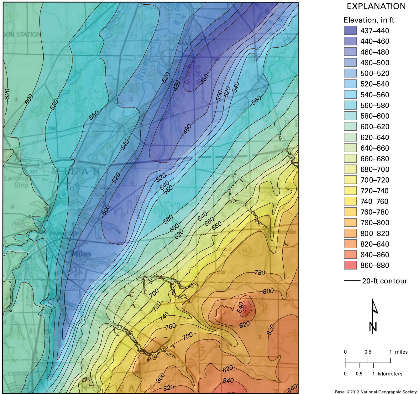
FIGURE 3. Bedrock topography of the Milan quadrangle. This map shows the elevation of the top of the bedrock surface, which over most of the mapped area also is the bottom of the glacial deposits.
