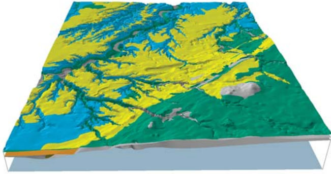
FIGURE 15. Three-dimensional view of the top surface of the Wisconsin lacustrine and beach sand (yellow) in the Milan quadrangle.
