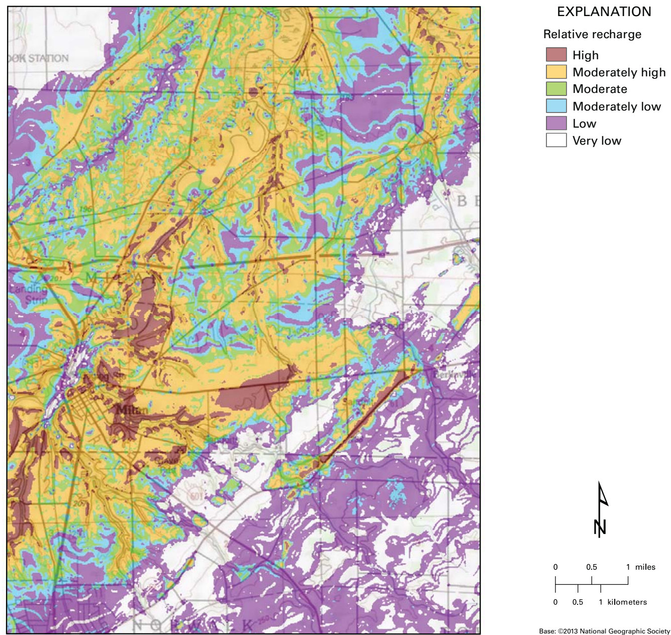
FIGURE 27. Relative ground-water recharge areas of the Milan quadrangle.
