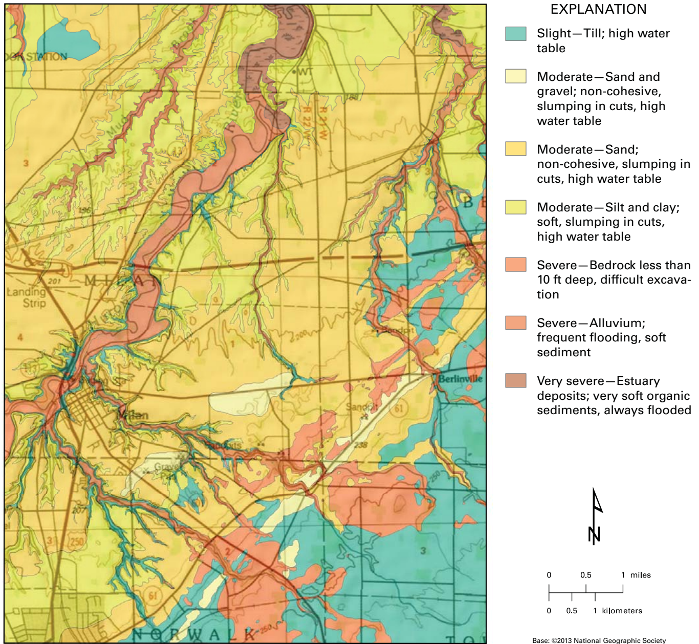
FIGURE 23. Limitations on construction and excavation in the Milan quadrangle.
