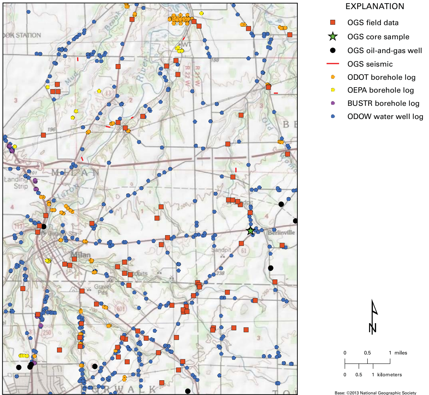
FIGURE 2. Subsurface data sources in the Milan quadrangle. OGS = Ohio Geological Survey; ODOT = Ohio Department of Transportation; OEPA = Ohio Environmental Protection Agency; BUSTR = Bureau of Underground Storage Tank Regulations.
