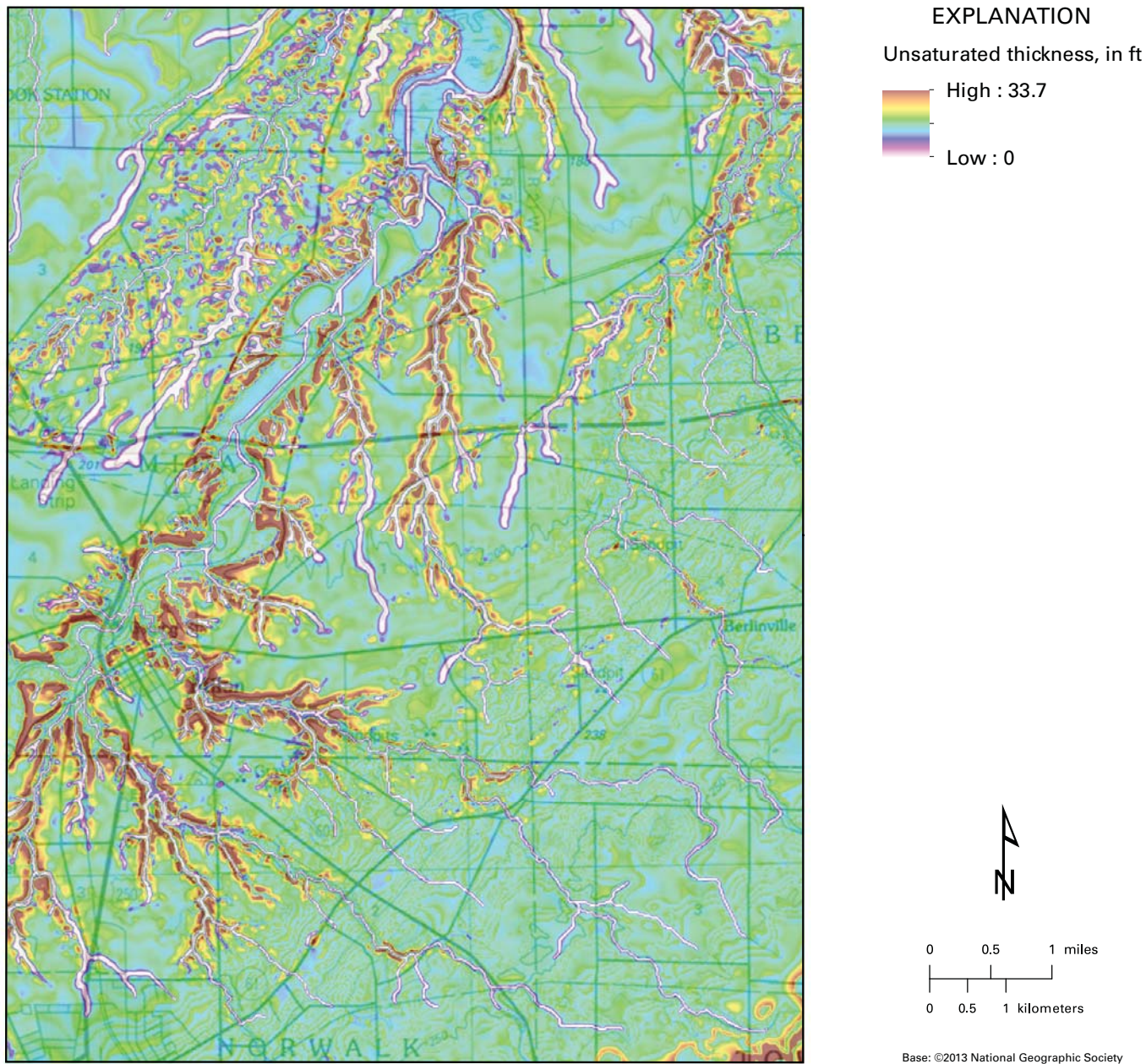
FIGURE 26. Unsaturated thickness of surficial units in the Milan quadrangle. This indicates the model estimate of depth to the unconfined water table.
