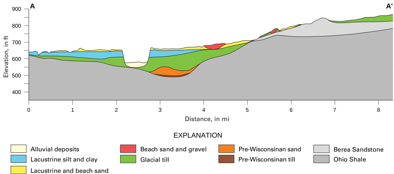
FIGURE 7. Typical cross section showing all of the geologic units in the Milan quadrangle. Cross section location shown in Figure 6.
