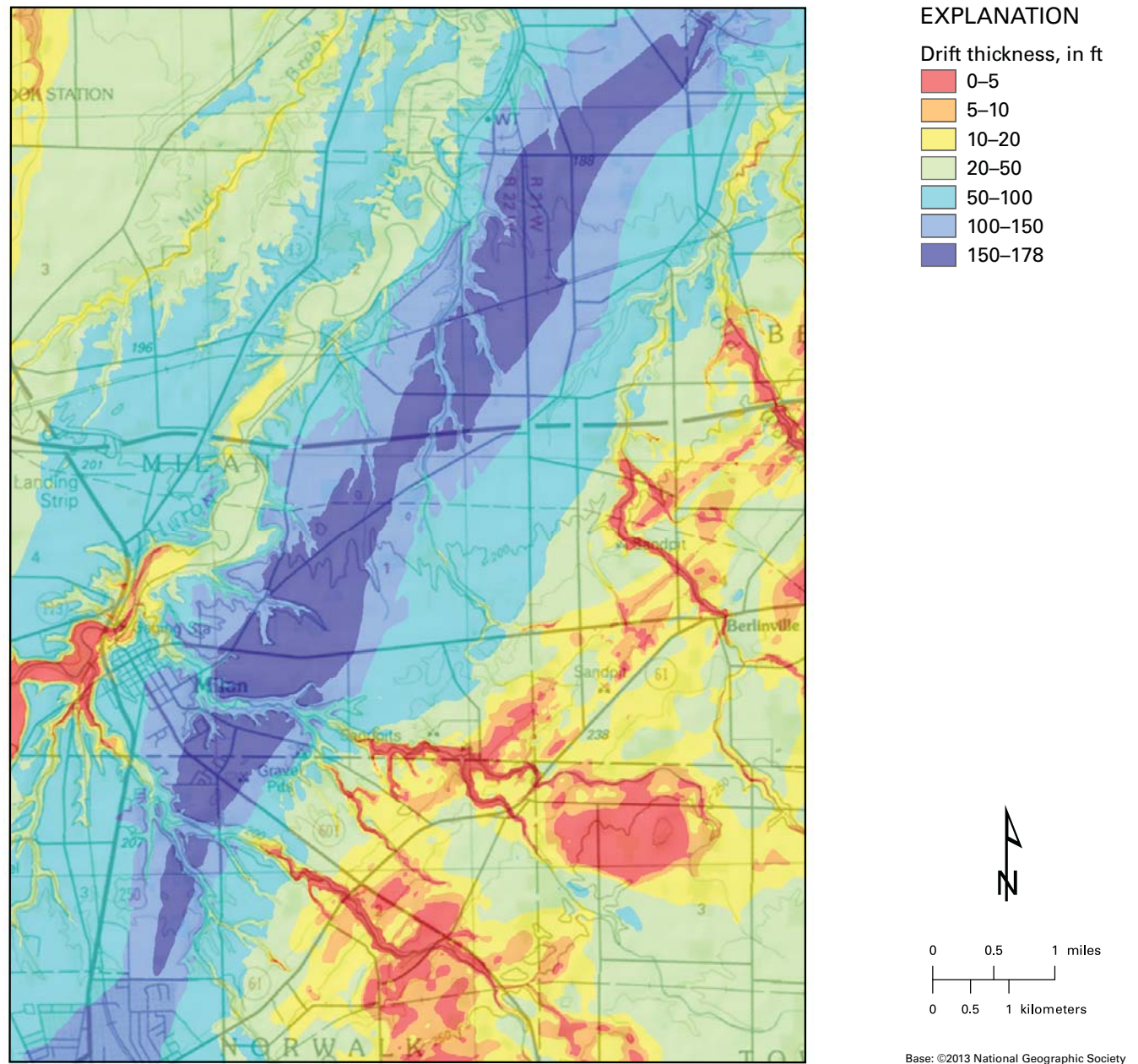
FIGURE 4. Drift thickness of the Milan quadrangle. This map shows the thickness of sediments from the top of the bedrock surface to the existing ground surface. The thickest deposits (dark blue) clearly define the long northeast-southwest valley that has been largely filled with glacial deposits and includes the best ground-water aquifer in the mapped area. Where the drift thickness is near zero (red areas), the bedrock is very thinly covered or exposed at the surface.
