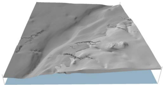
FIGURE 9. Three-dimensional view of the top surface of the Berea Sandstone (light gray) above the top of the Ohio Shale (dark gray) in the Milan quadrangle. This represents the surface of the bedrock as it was left after erosion and glacial scouring and prior to deposition of glacial and fluvial sediments, with the exception of the steep modern valleys incised into the bedrock.
