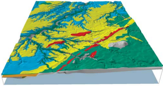
FIGURE 17. Three-dimensional view of the top surface of the Wisconsin beach ridge sand and gravel (red) in the Milan quadrangle.
