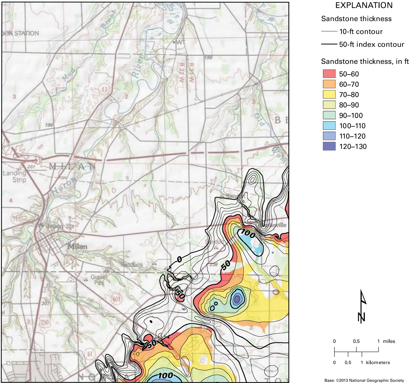
FIGURE 25. Map showing potential dimension stone resources in the Milan quadrangle. Black contours indicate the thickness of the Berea Sandstone. Color fill indicates thickness of resources that are at least 50 ft thick and have less than 20 ft of overburden.
