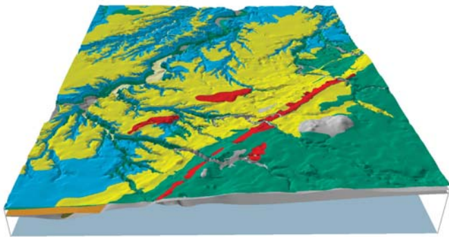
FIGURE 18. Three-dimensional view of the top surface of the Holocene alluvium (light yellow) in the Milan quadrangle.
