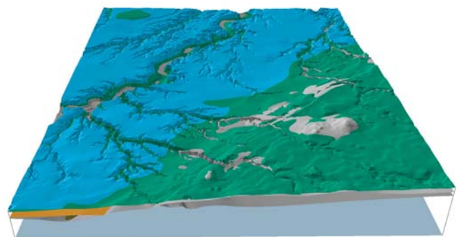
FIGURE 13. Three-dimensional view of the top surface of the Wisconsinan lacustrine silt and clay (blue) in the Milan quadrangle.
