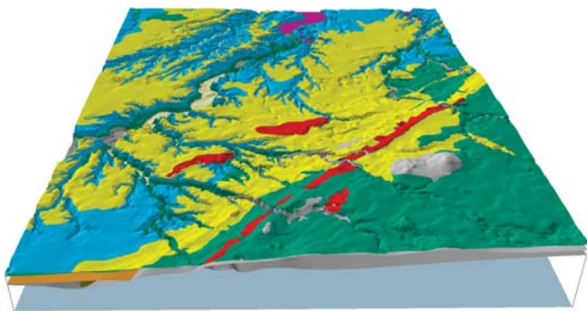
FIGURE 19. Three-dimensional view of the top surface of the Holocene estuary deposits (purple) in the Milan quadrangle. This map completes the sequence of the map “stack.” This map alone (in a 2-D top down view) shows how prior surficial mapping was done—only showing the materials present at the surface. The 3-D stack sequence mapping now allows access to the location and qualities of all near-surface materials.
