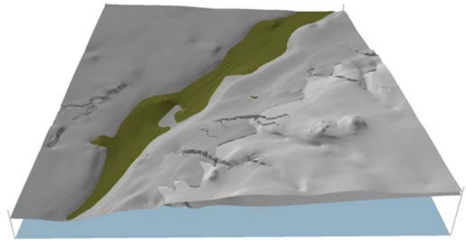
FIGURE 10. Three-dimensional view of the top surface of the pre-Wisconsinan till (brown) overlying the Ohio Shale (dark gray) in the Milan quadrangle.
