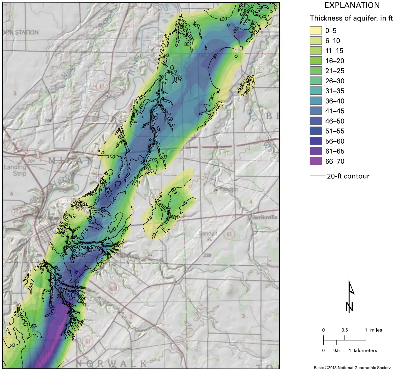
FIGURE 21. The thickness of the Milan quadrangle primary aquifer (pre-Wisconsinan sand) is shown in color; contours indicate the depth to this unit.
