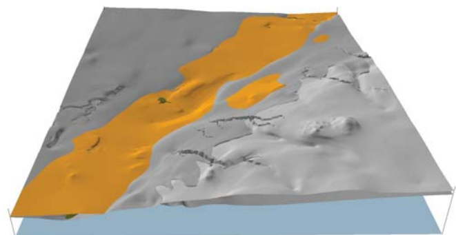
FIGURE 11. Three-dimensional view of the top surface of the pre-Wisconsinan sand (orange) overlying the Ohio Shale (dark gray) and pre-Wisconsinan till (brown) in the Milan quadrangle.
