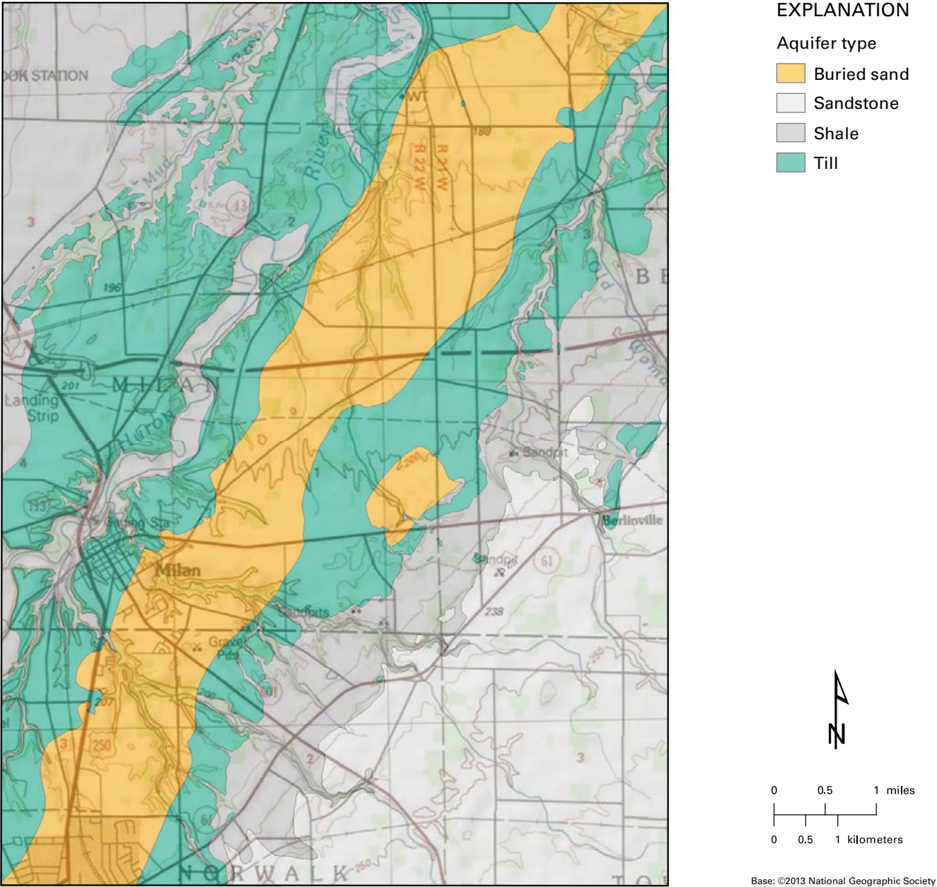
FIGURE 20. Ground-water resources of the Milan quadrangle. Construction of this map assumes that a minimum of 25 ft of casing is required to protect from surface contamination, and a minimum of 10 ft of screened aquifer interval below casing is generally needed for adequate production.
