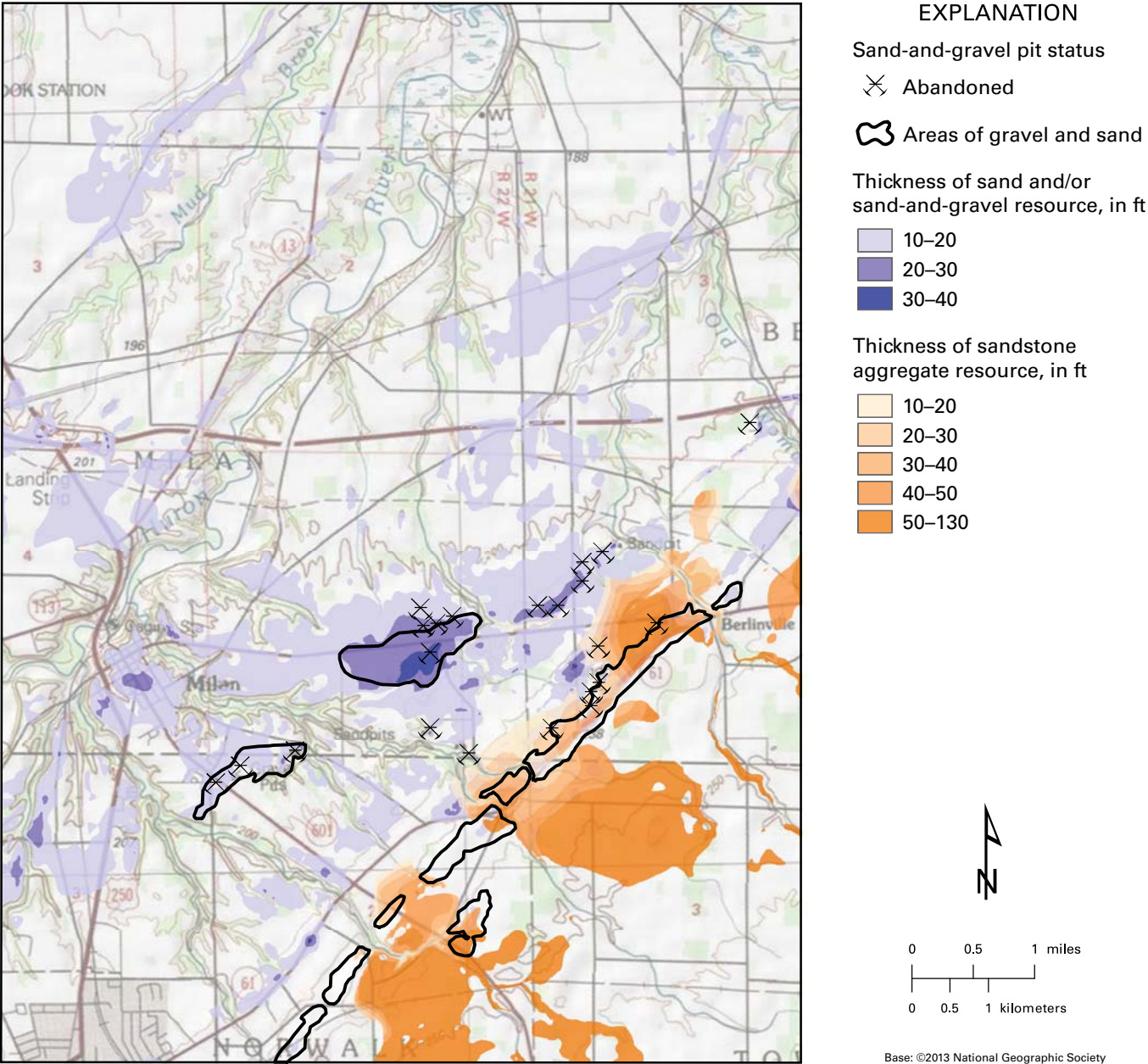
FIGURE 24. Aggregate resources in the Milan quadrangle.
