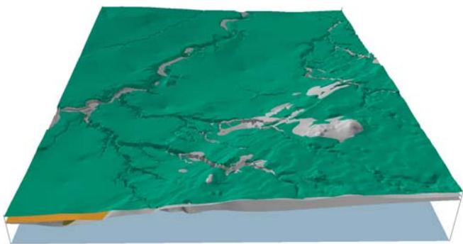
FIGURE 12. Three-dimensional view of the top surface of the Wisconsinan till (green) in the Milan quadrangle.
