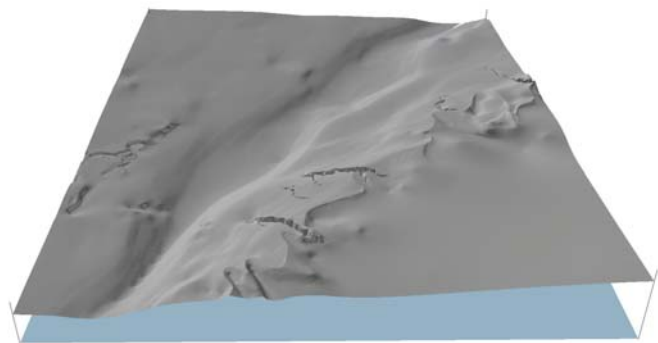
FIGURE 8. Three-dimensional view of the top surface of the Ohio Shale. This and subsequent 3-D views of the Milan quadrangle are from the south, with illumination from the northwest.
