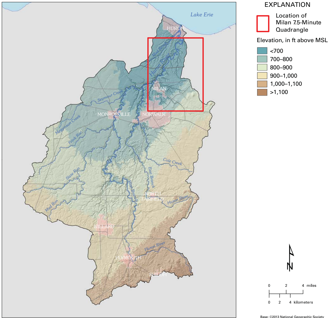
FIGURE 14. Extent of the Huron River watershed in Ohio.
