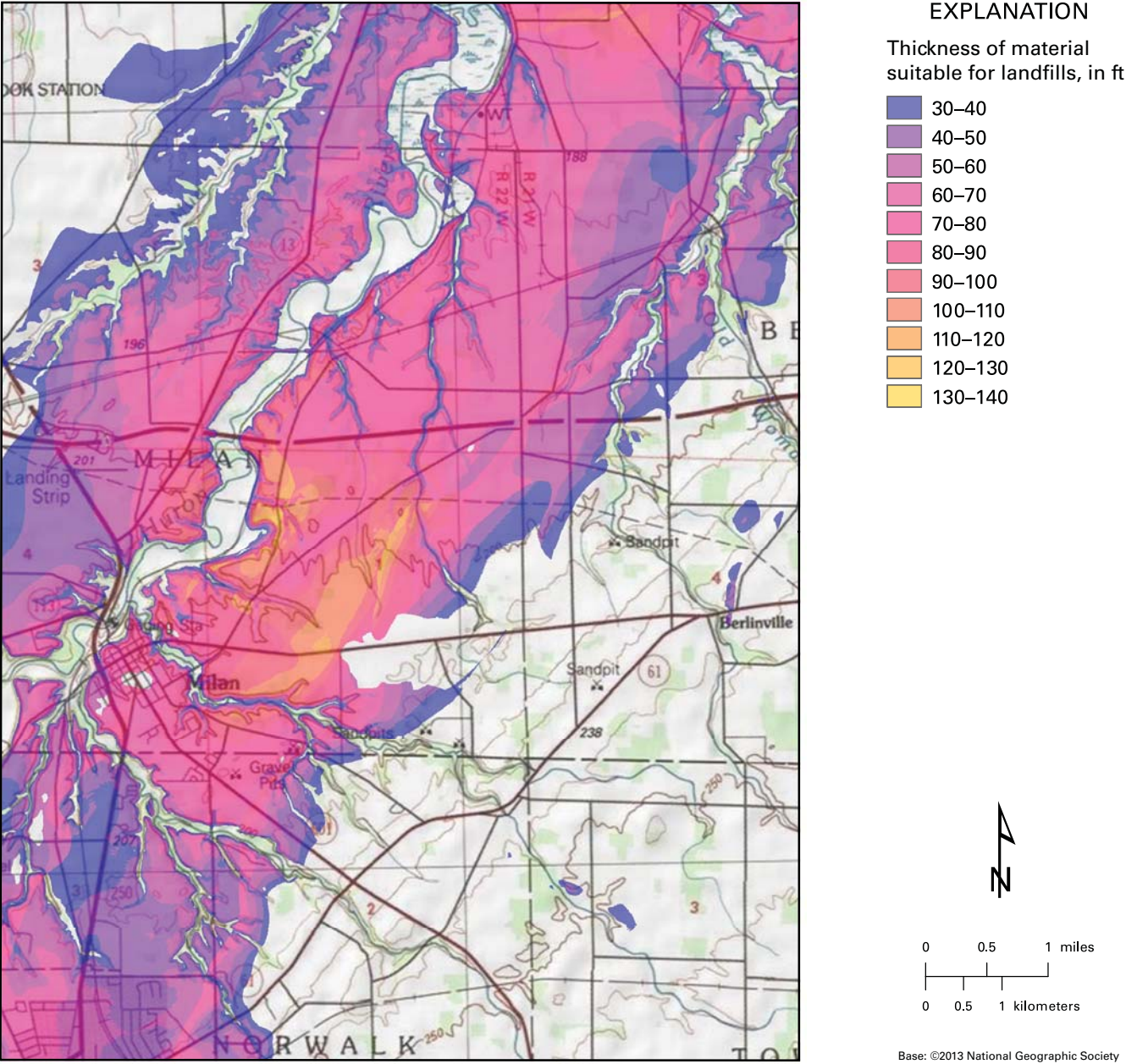
FIGURE 22. Areas suitable for landfills in the Milan quadrangle. Suitability requirements are a minimum of 30 ft of low-permeability material, with a minimum 20 ft of separation from aquifers, and a maximum high permeability cover of 20 ft.
