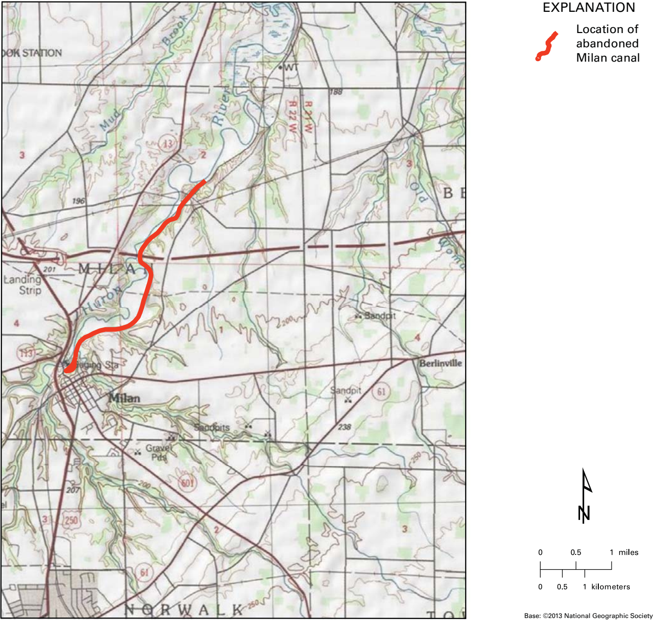
FIGURE 16. Location of the abandoned Milan Canal in the Milan 7.5-minute quadrangle.
