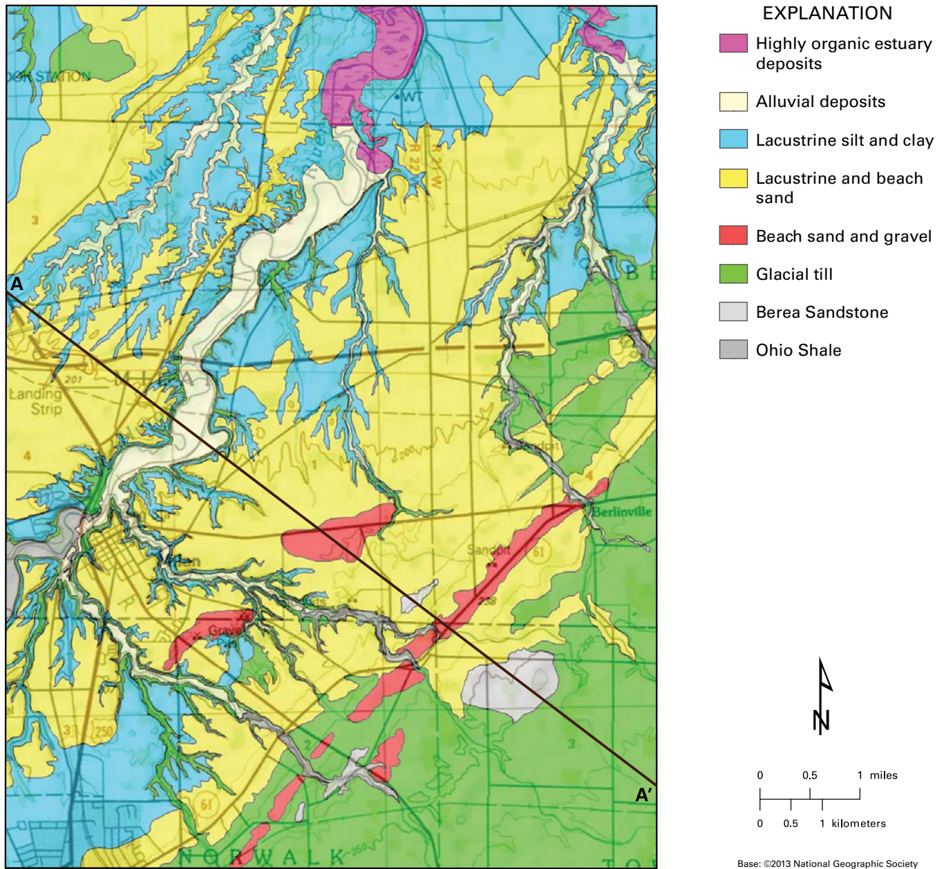
FIGURE 6. Surficial geology of the Milan quadrangle. Line A–A' indicates the location of the cross section shown in Figure 7.
