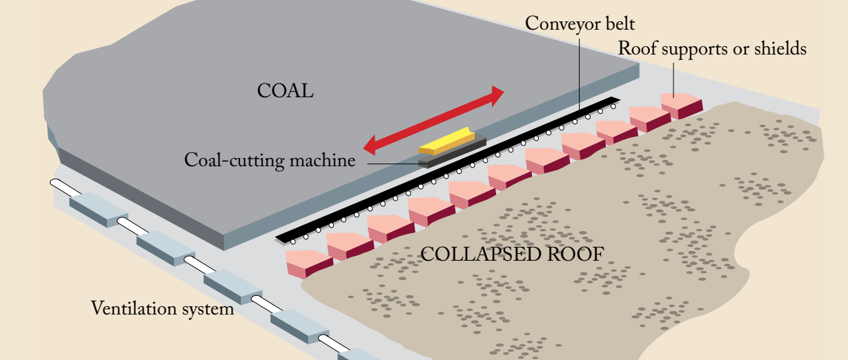
Figure 3.—Longwall underground-mining method. In a longwall mine, a cutting machine moves back and forth across a panel of coal that can be up to 1,100 feet in width and 7,000 feet in length. The cut coal falls onto a flexible conveyor for removal. Hydraulic supports (shields) hold up the mine roof and protect the workers, and cutting machinery is advanced as the coal is cut. The roof in the mined-out area falls as the shields advance. (Graphic from The Columbus Dispatch , 2006, used with permission.)
