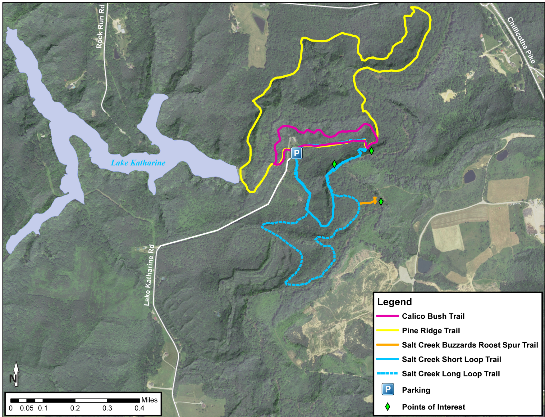
Lake Katharine State Nature Preserve trail map showing topography of the area and geologic sites discussed in the text.
