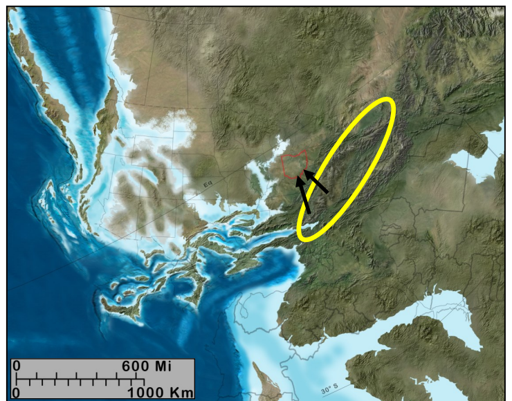
Figure 2. The general location of Ohio (outlined in red) during the Early Pennsylvanian Period. The Alleghenian mountains lie to the east (yellow oval). Also indicated is the approximate flow direction of Sharon sandstone deposition from the eastern Alleghenian mountains into Ohio. Base map credit: Key Time Slices of North America, ©2013 Colorado Plateau Geosystems, Inc.
