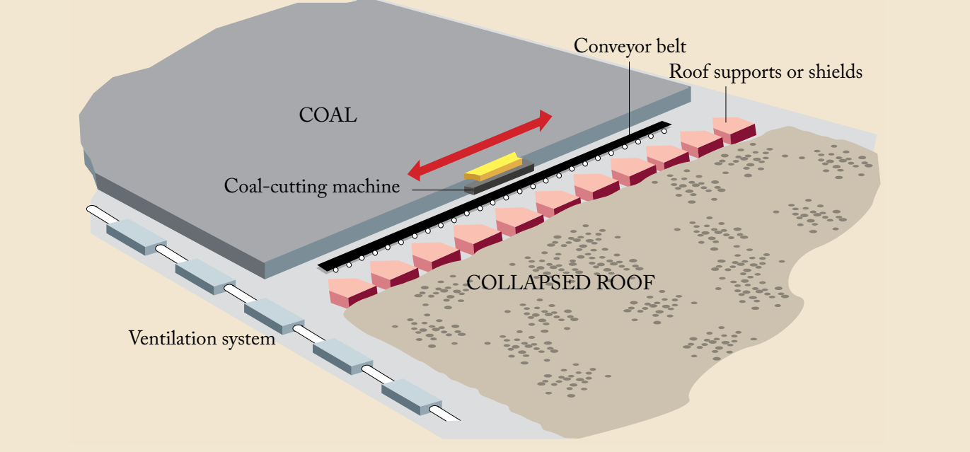
Figure 3—Longwall underground mining method. In a longwall mine, a cutting machine moves back and forth across a panel of coal that can be up to 1,100 feet in width and 7,000 feet in length. A flexible conveyor is used for removal. Hydraulic supports (shields) hold up the mine roof and protect the workers, and cutting machinery is advanced as the coal is cut. The roof in the mined-out area falls as the shields advance. (Graphic from The Columbus Dispatch , 2006, used with permission.)
