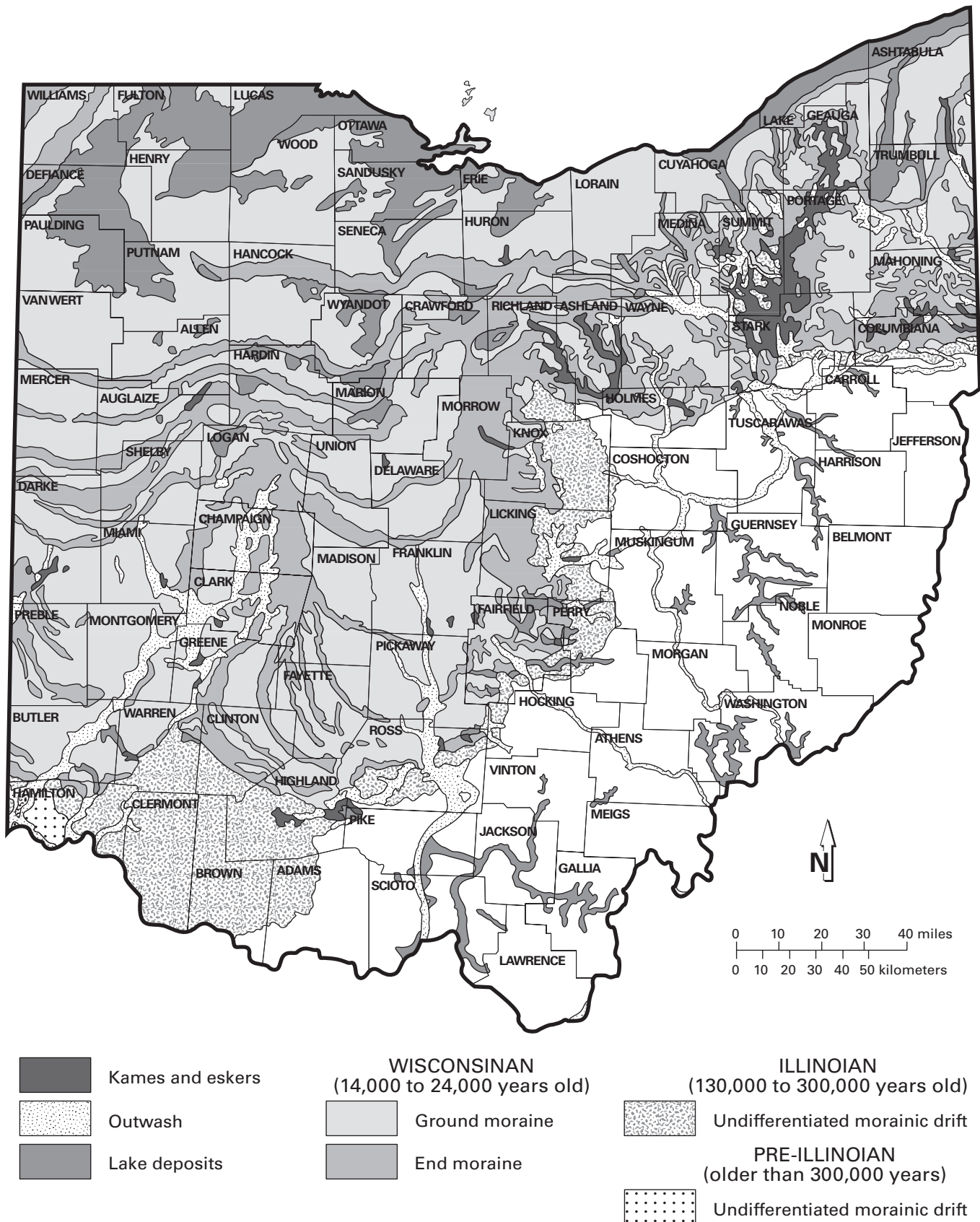
FIGURE 2.—Generalized map of the glacial deposits of Ohio. Continental glaciers advanced over the Ohio landscape several times during the Ice Age. These glaciers deposited unconsolidated materials on top of the bedrock over nearly two-thirds of the state. Most of Ohio's sand and gravel production comes from kames, eskers, and outwash, which were deposited by meltwater from the glaciers. Other glacially derived industrial minerals in Ohio include peat and clay.
