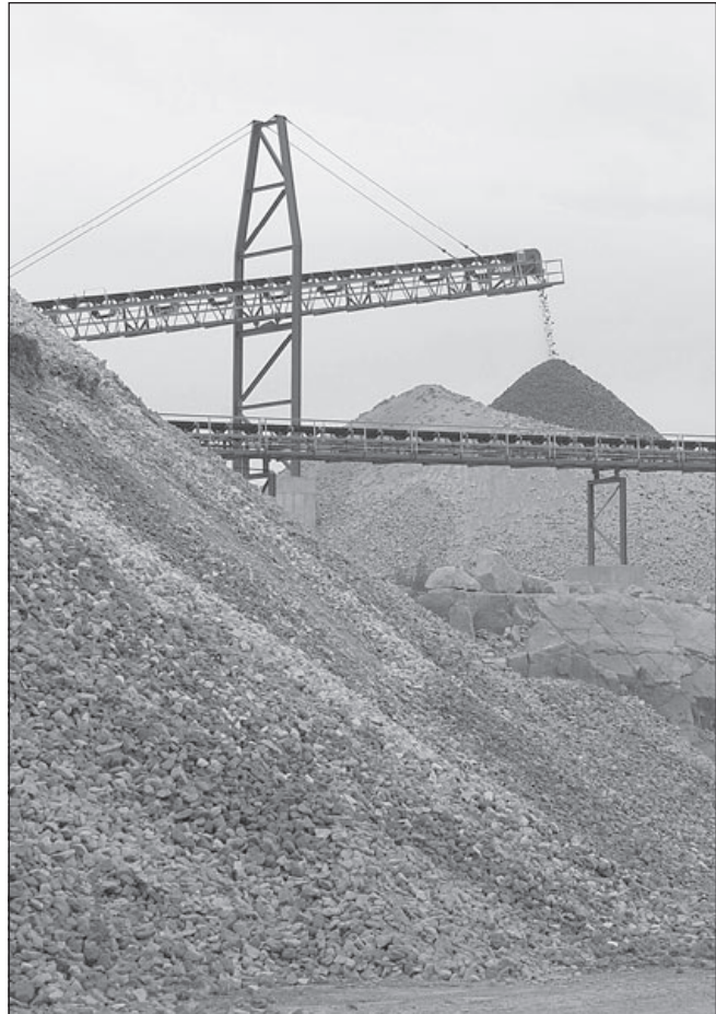
Stockpiling and stockpile management are critical to aggregate quality. Ohio Level 1 Aggregate Technician Training teaches proper methods. Pictured here is the conveyor and stockpile at the Shelly Materials, Inc., Plant #10 in Union County. Photo by Michael D. Williams, Ohio Department of Natural Resources.
