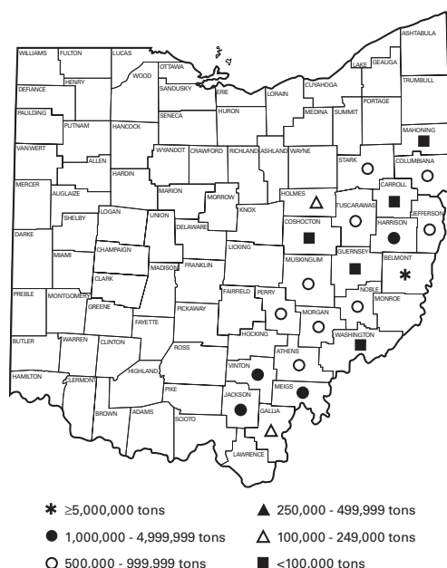
FIGURE 4.—Coal production in Ohio in 2000, by county.
