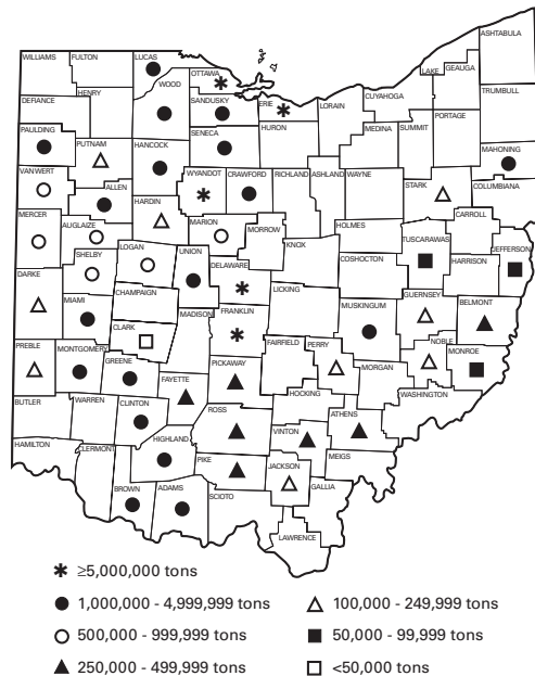
FIGURE 6.—Sales of limestone and dolomite in Ohio in 2000, by county.
