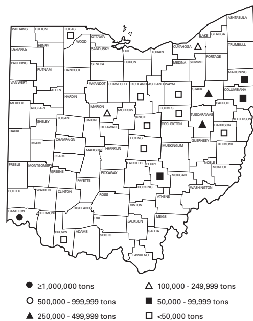
FIGURE 14.—Shale sales in Ohio in 2000, by county.
