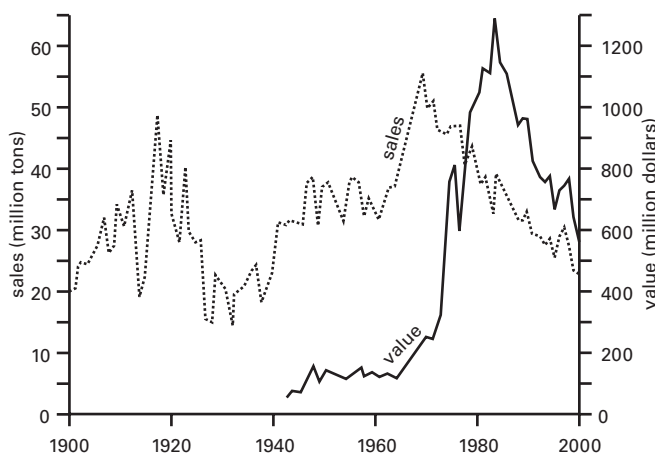
FIGURE 5.—Sales and value of coal in Ohio.
