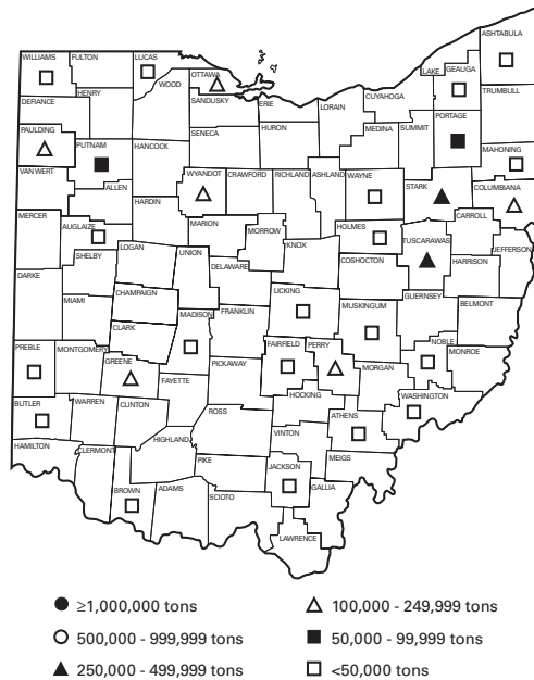
FIGURE 12.—Clay sales in Ohio in 2000, by county.
