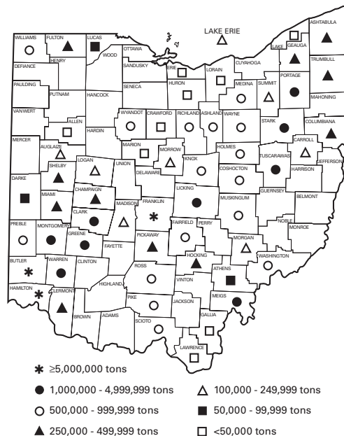
FIGURE 8.—Sales of sand and gravel in Ohio in 2000, by county.
