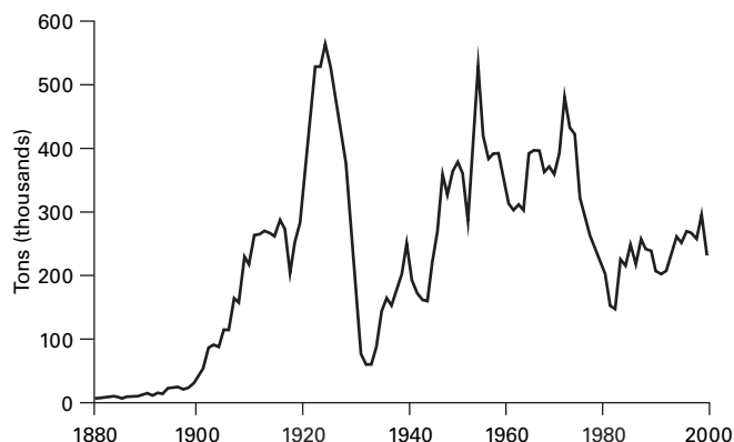
Annual production of gypsum in Ohio from 1881 to 2000. From the annual Ohio Division of Mines report , 1958-1980, and the annual Ohio Division of Geological Survey Report on Ohio mineral industries , 1981-2001.
