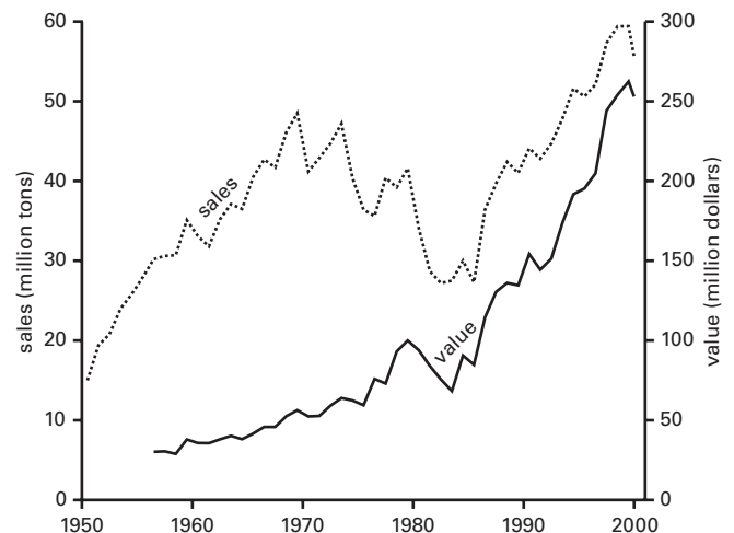
FIGURE 9.—Sales and value of sand and gravel in Ohio. Value line dashed where data not available. Figures from 1984 to 2000 include Lake Erie dredged material.
