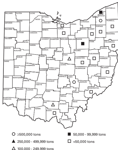
FIGURE 10.—Sales of sandstone and conglomerate in Ohio in 2000, by county.
