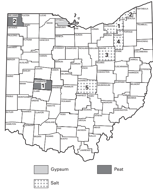
FIGURE 19.—Counties producing salt, gypsum, and peat in Ohio in 2000, and their ranking in sales.
