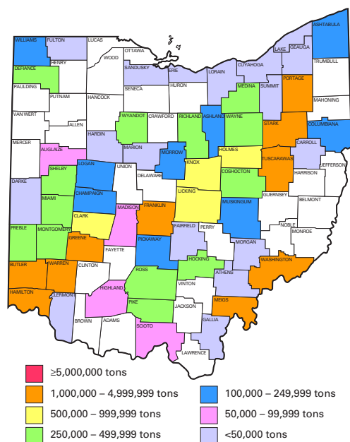
FIGURE 8.—Sales of sand and gravel in Ohio in 2011, by county and quantity.
