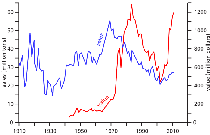
FIGURE 3.—Sales and value of coal in Ohio.
