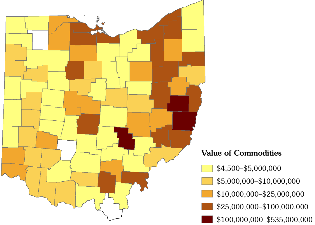
Total value of produced coal and/or industrial minerals in Ohio in 2011, by county.
