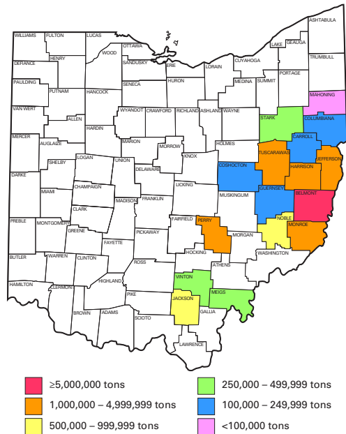
FIGURE 2.—Coal production in Ohio in 2011, by county and quantity.
