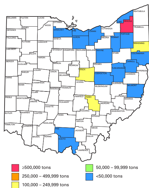
FIGURE 10.—Sales of sandstone and conglomerate in Ohio in 2011, by county and quantity.
