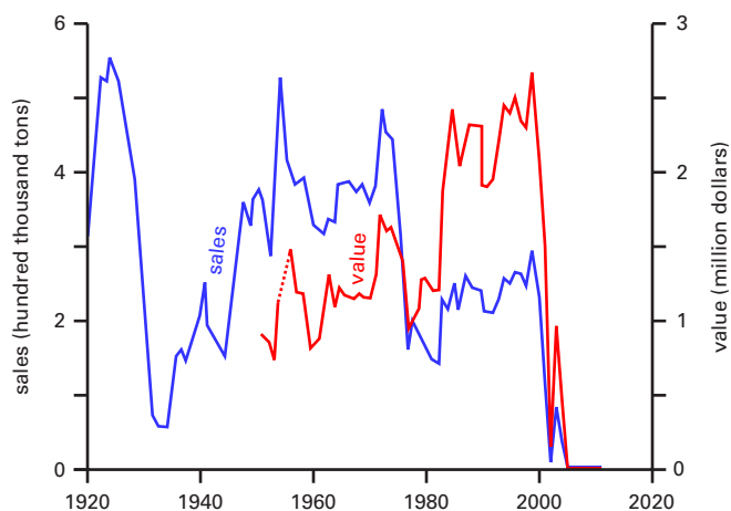
FIGURE 18.—Sales and value of gypsum in Ohio. Value line dashed where data not available. Some sales and values were estimated because in order to maintain confidentiality, actual sales and values were not reported.
