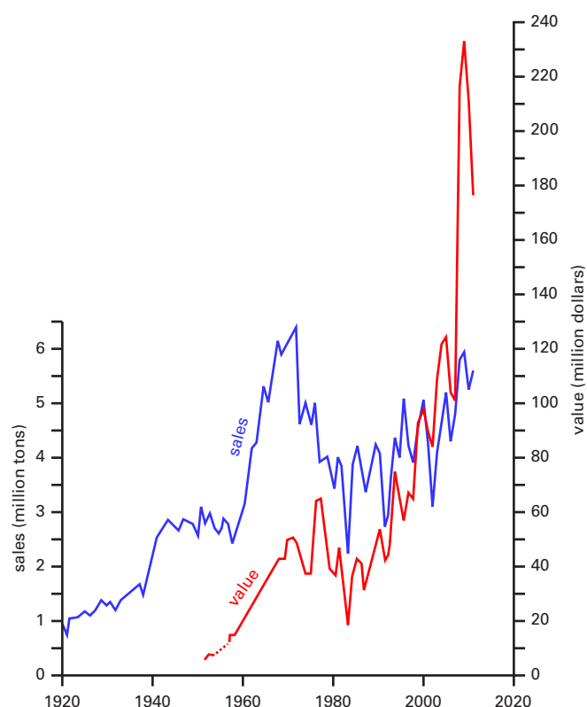
FIGURE 17.—Sales and value of salt in Ohio. Value line dashed where data not available.
