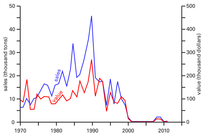
FIGURE 19.—Sales and value of peat in Ohio.
