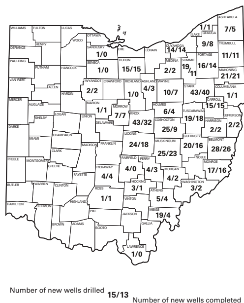
FIGURE 20.—New wells drilled and completed (including dry holes) for oil and gas in Ohio in 2011, by county (from DMRM, 2012).
