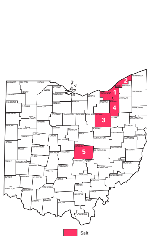
FIGURE 16.—Counties producing salt in Ohio in 2011 and their rankings in sales.
