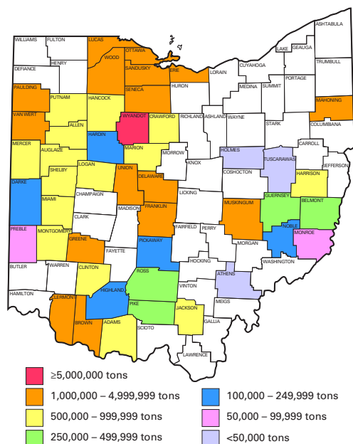
FIGURE 5.—Sales of limestone and dolomite in Ohio in 2011, by county and quantity.
