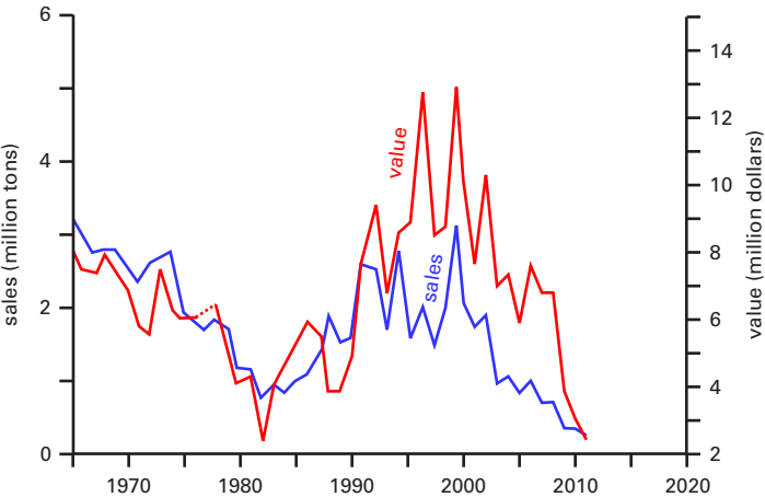
FIGURE 13.—Sales and value of clay in Ohio. Value line dashed where data not available.
