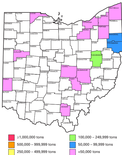
FIGURE 12.—Clay sales in Ohio in 2011, by county and quantity.
