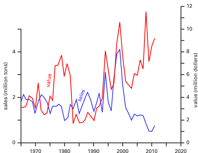
FIGURE 15.—Sales and value of shale in Ohio.
