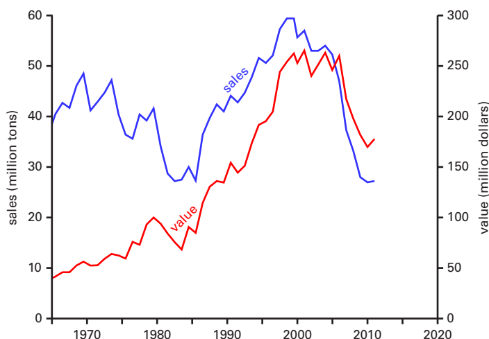
FIGURE 9.—Sales and value of sand and gravel in Ohio.
