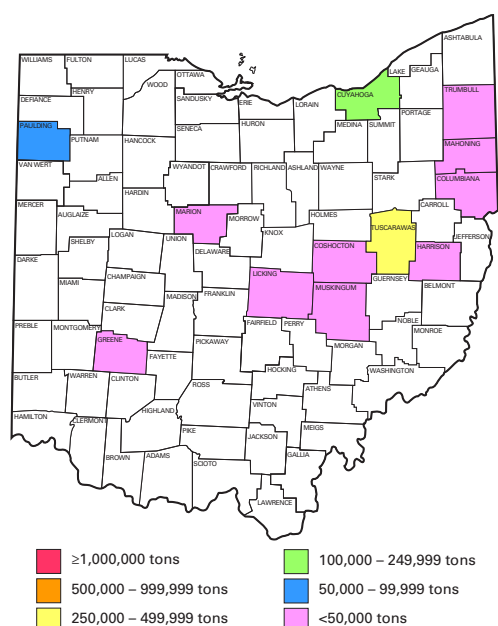
FIGURE 14.—Shale sales in Ohio in 2011, by county and quantity.
