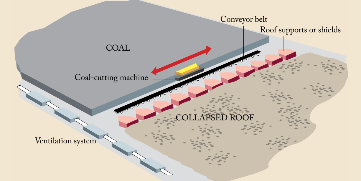
Figure 3—Longwall underground-mining method. In a longwall mine, a cutting machine moves back and forth across a panel of coal that can be up to 1,100 feet in width and 7,000 feet in length. The coal falls onto a flexible conveyor for removal. Hydraulic supports (shields) hold up the mine roof and protect the workers, and cutting machinery is advanced as the coal is cut. The roof in the mined-out area falls as the shields advance. (Graphic from The Columbus Dispatch , 2006, used with permission.)
