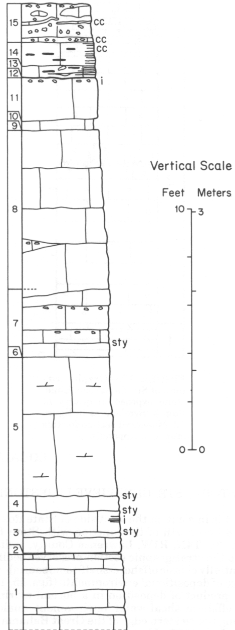
FIGURE 16.—Graphic column of upper part of Ste. Genevieve Limestone exposed at Stop 4. See figure 15 for explanation of symbols. Measured section for this stop is in Appendix.
