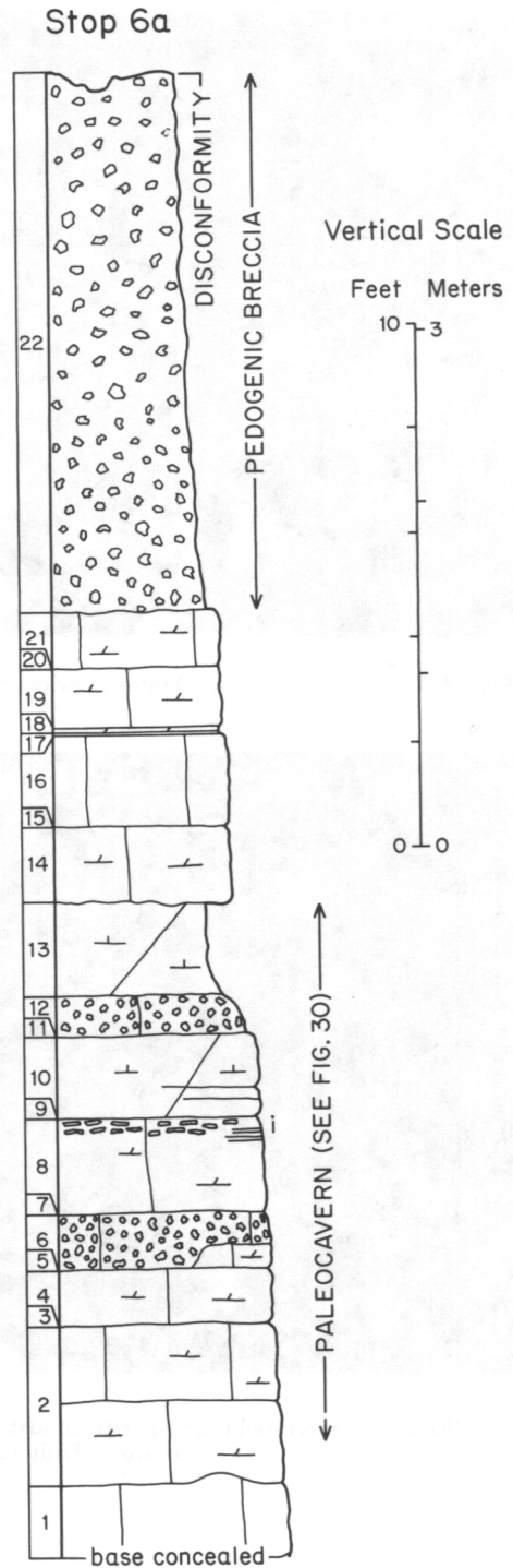
FIGURE 27.—Graphic section of St. Louis Limestone exposed at Stop 6a. Section was measured just to left of cliff-face cross section depicted in figure 30. See figure 15 for explanation of symbols. Measured section for this stop is in Appendix.
