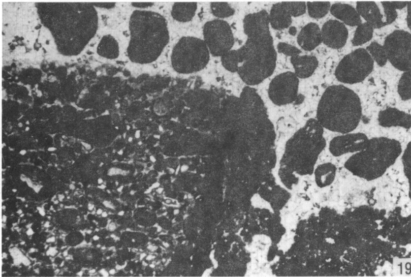
FIGURE 19.—Supratidal rock that has been affected by pedogenesis. Note clasts in birdseye structure and bit of calcrite crust on right side (lower left) of mixed-grain packstone. Unit 15, Stop 4. Plane-polarized light, X20.
