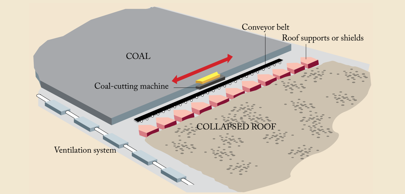
Figure 3—Longwall underground mining method. In a longwall mine, a cutting machine moves back and forth across a panel of coal that can be up to 1,100 feet in width and 7,000 feet in length. As mining progresses, roof supports are removed. Hydraulic supports (shields) hold up the mine roof and protect the workers, and cutting machinery is advanced as the coal is cut. The roof in the mined-out area falls as the shields advance. (Graphic from The Columbus Dispatch , 2006, used with permission.)
