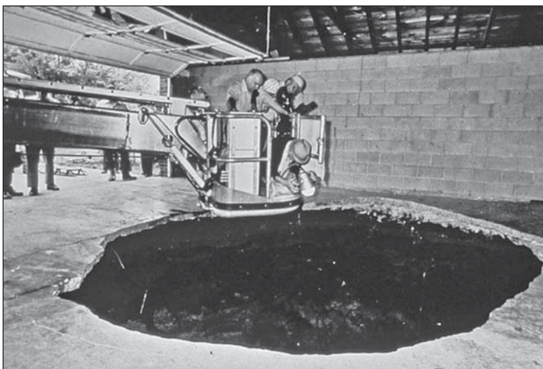
FIGURE 1.—Collapse of the mine shaft seal, Foster No. 1 mine, Youngstown, Ohio. Here a boom and bucket is used in examining the collapsed mine shaft seal in the homeowner's garage. Photo courtesy of The Vindicator .
