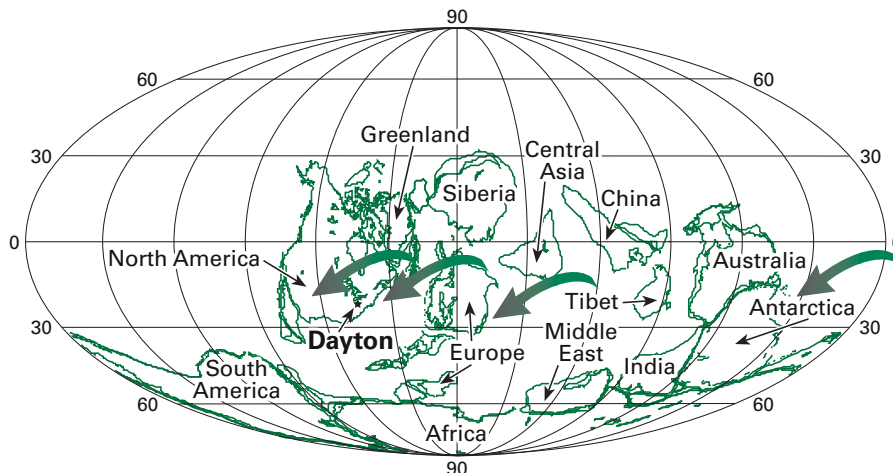
FIGURE 2.—Location of the Dayton region in Ordovician time. Large arrows depict the probable Ordovician hurricane tracks. Modified from Coogan (1996).
