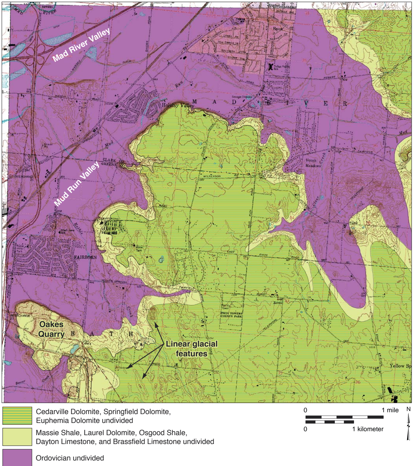
FIGURE 5.—Bedrock geologic map of Oakes Quarry Park area illustrating the broad valleys of Mud Run and the Mad River. These valleys would have been the first areas filled with advancing glacial ice. As the glacial ice thickness increased above the elevation of the adjacent uplands, ice would flow laterally over Oakes Quarry and to areas eastward. The southeastward flowing ice produced linear glacial features that parallel ice and meltwater flow direction.
