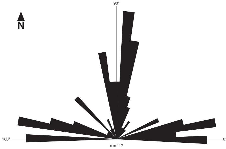
FIGURE 8.—Rose diagram illustrating the prominent joint orientations preserved within the Belfast Member of the Brassfield Formation as exposed in the floor of Oakes Quarry Park. Measured by Emily Denlinger, Matt Erenpriess, Jonathan Pratt, Steve Riley, Greg Schumacher, and Claire Westervelt.
