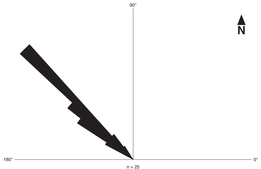
FIGURE 11.—Rose diagram showing that the movement of glacial ice and meltwater at Oakes Quarry Park was from the northwest to the southeast. Figure 5 illustrates a similar pattern of linear glacial features that correspond to a northwest-southeast ice or meltwater flow.
