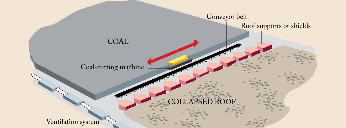
Figure 3—Longwall underground-mining method. In a longwall mine, a cutting machine moves back and forth across a panel of coal that can be up to 1,100 feet in width and 7,000 feet in length. As mining progresses through a panel, no roof-supporting pillars are left in the extraction areas; instead, the roof-rock is allowed to collapse into the mined-out area. Hydraulic supports (shields) hold up the mine roof and protect the workers, and cutting machinery is advanced as the coal is cut. The roof in the mined-out area falls as the shields advance. (Graphic from The Columbus Dispatch , 2006, used with permission.)
