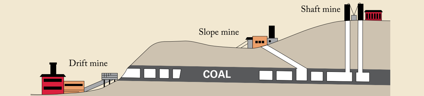
Figure 1—Types of underground mining methods used in Ohio (modified from Crowell, 2000).
