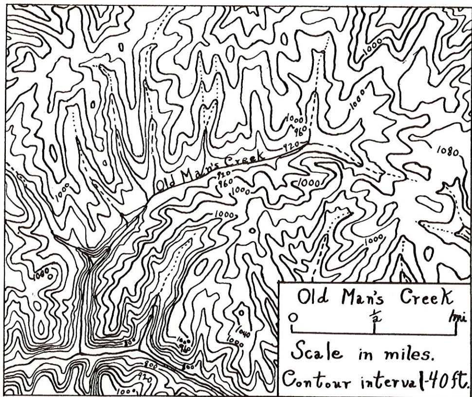
Fig. 22. Topographic map of the area drained by Old Man's Creek, Hocking County.
