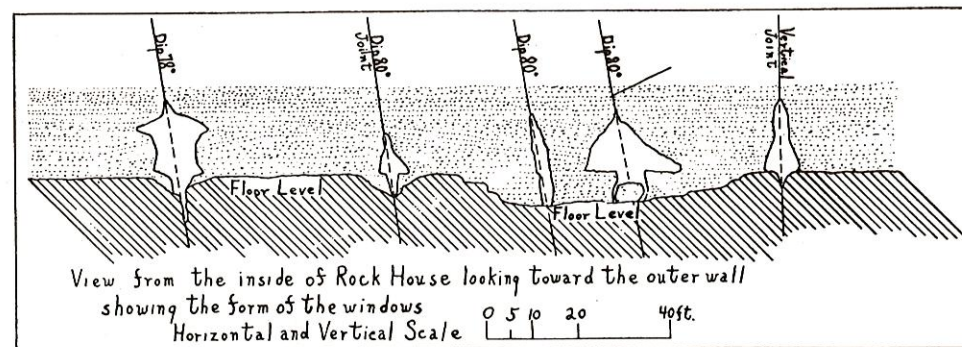
Fig. 32. View from the inside of Rock House looking toward the outer wall showing the form of the windows, and the position of the cross joints.
