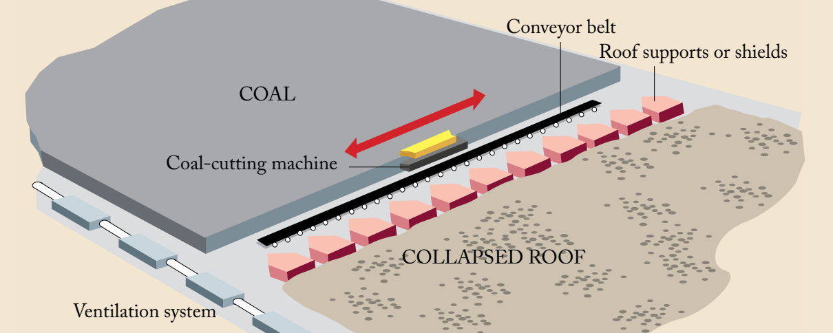
Figure 3—Longwall underground mining method. In a longwall mine, a cutting machine moves back and forth across a panel of coal that can be up to 1,100 feet in width and 7,000 feet in length. The cut coal falls onto a flexible conveyor or return airway. Hydraulic supports (shields) hold up the mine roof and cutting machinery as the coal is cut. The roof in the mined-out area falls as the shields advance. (Graphic from The Columbus Dispatch , 2006, used with permission.)
