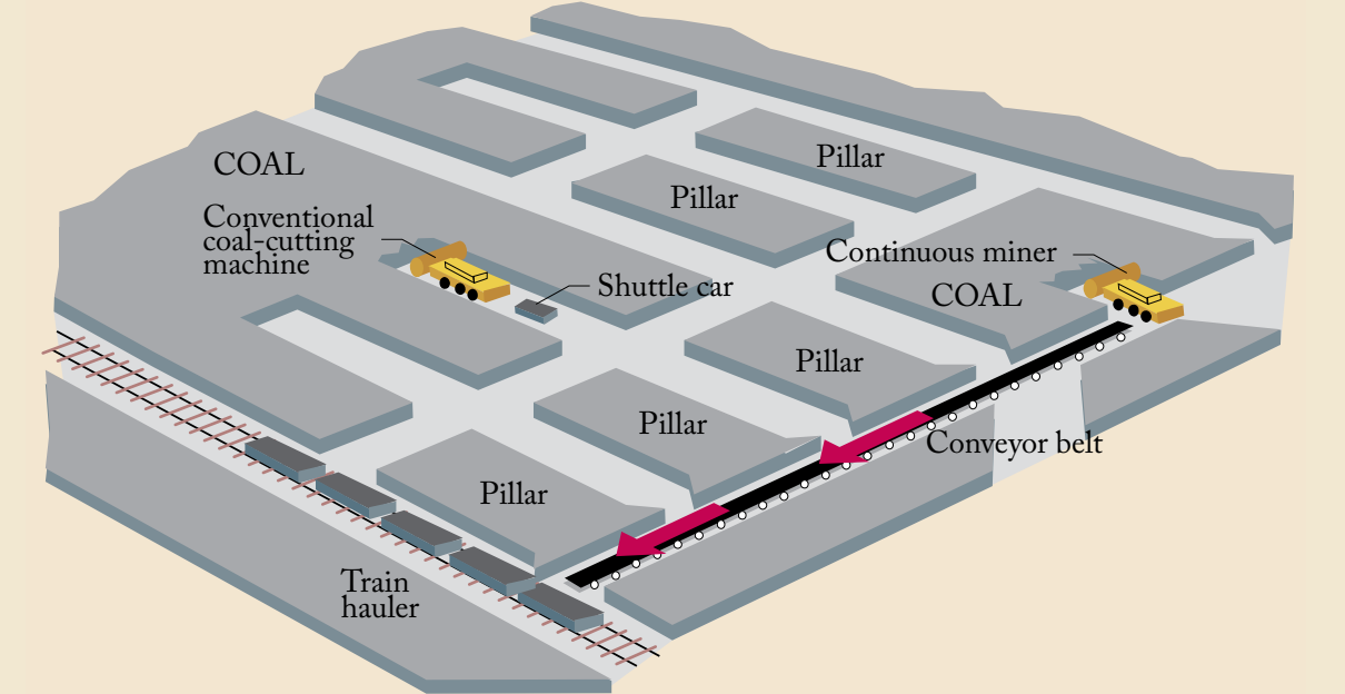
Figure 2—Room-and-pillar mining method. In most older mines, the rooms were created by blasting and excavating the coal into shuttle cars that hauled coal to the surface. Most modern room-and-pillar mines use continuous-miner machinery to cut and directly feed the coal to a conveyor system that transports it to the surface. (Graphic from The Columbus Dispatch , 2006, used with permission.)
