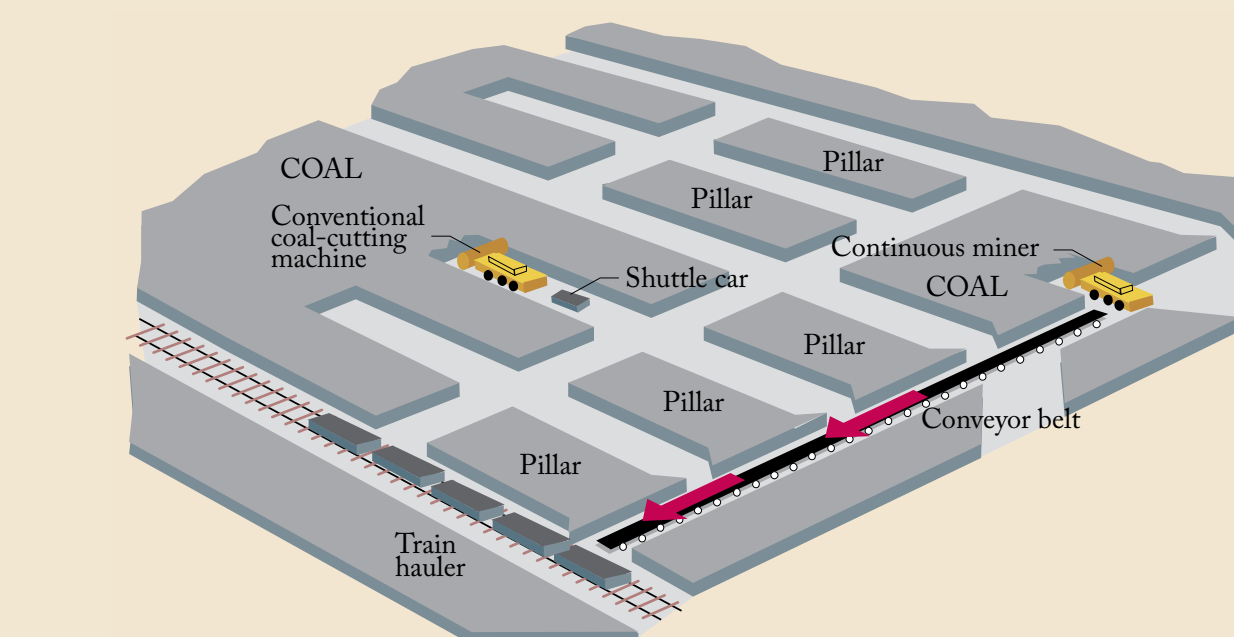
Figure 2—Room-and-pillar underground mining method. In most older mines, the rooms were created by blasting and excavating the coal into shuttle cars that hauled coal to the surface. Most modern room-and-pillar mines use continuous-miner machinery to cut and directly feed the coal to a conveyor system that transports it to the surface. (Graphic from The Columbus Dispatch , 2006, used with permission.)
