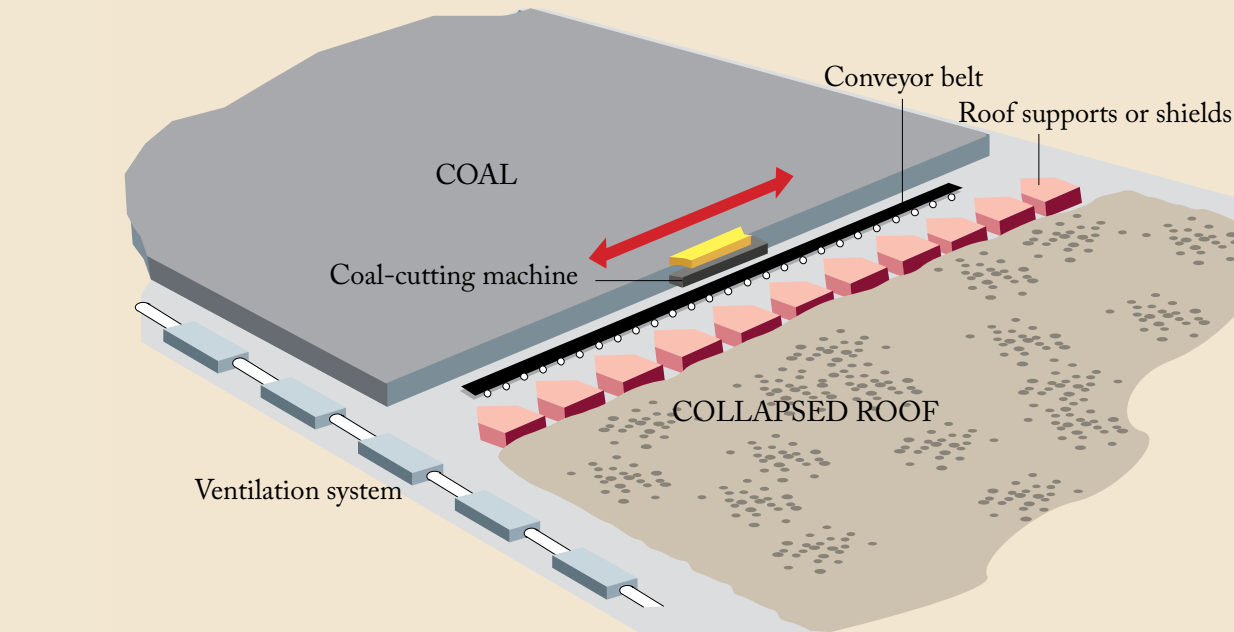
Figure 3—Longwall underground-mining method. In a longwall mine, a cutting machine moves back and forth across a panel of coal that can be up to 1,100 feet in width and 7,000 feet in length. The cut coal falls onto a flexible conveyor for removal. Hydraulic supports (shields) hold up the mine roof and protect the workers and cutting machinery as the coal is cut. The roof in the mined-out area falls as the shields advance. (Graphic from The Columbus Dispatch , 2006, used with permission.)
