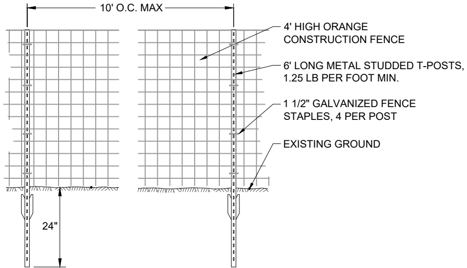
TEMPORARY FENCE DETAIL NOT TO SCALE
