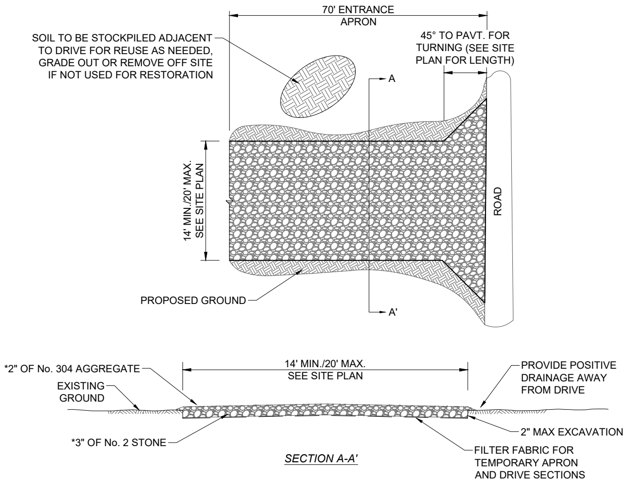
(TEMPORARY) ENTRANCE APRON & ACCESS DRIVE NOT TO SCALE
