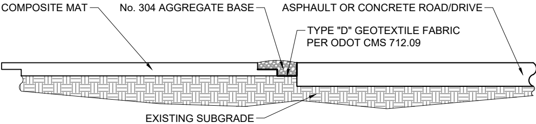
PAVEMENT TO MATTING ACCESS OVERLAY NOT TO SCALE
