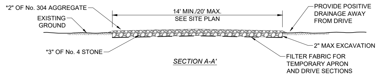
(TEMPORARY) ENTRANCE APRON & ACCESS DRIVE NOT TO SCALE
