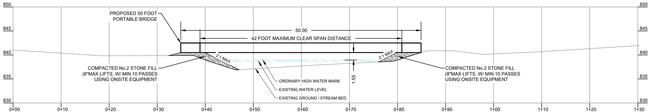
50 FOOT BRIDGE AND STONE ABUTMENT PROFILE SCALE: HORIZ.=1:10 VERT.=1:10
