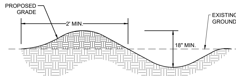
WATER BAR DETAIL NOT TO SCALE
