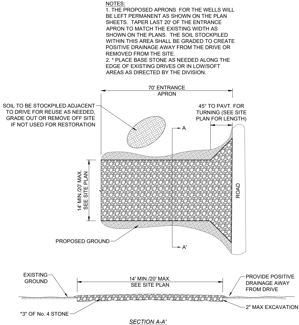
ENTRANCE APRON & ACCESS DRIVE NOT TO SCALE
