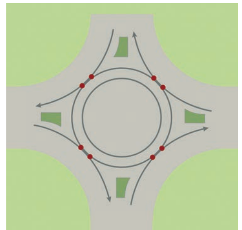
● Potential vehicle conflict points in roundabout intersections – head-on and high-speed right angle crashes are virtually eliminated. Drivers may not be looking for motorcycles. Stay MORE alert.
