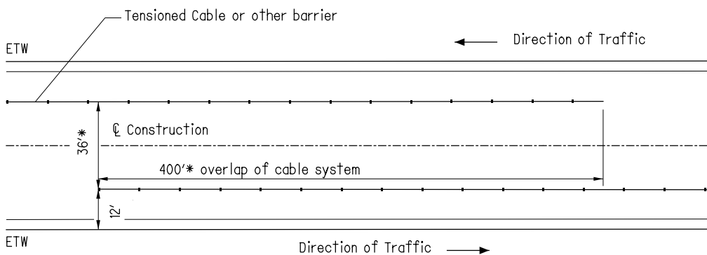
TENSIONED CABLE ANCHOR ASSEMBLY OVERLAP
