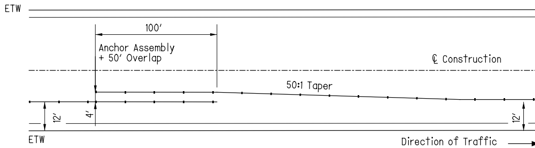
TENSIONED CABLE ANCHOR ASSEMBLY OVERLAP (on same side of median)
