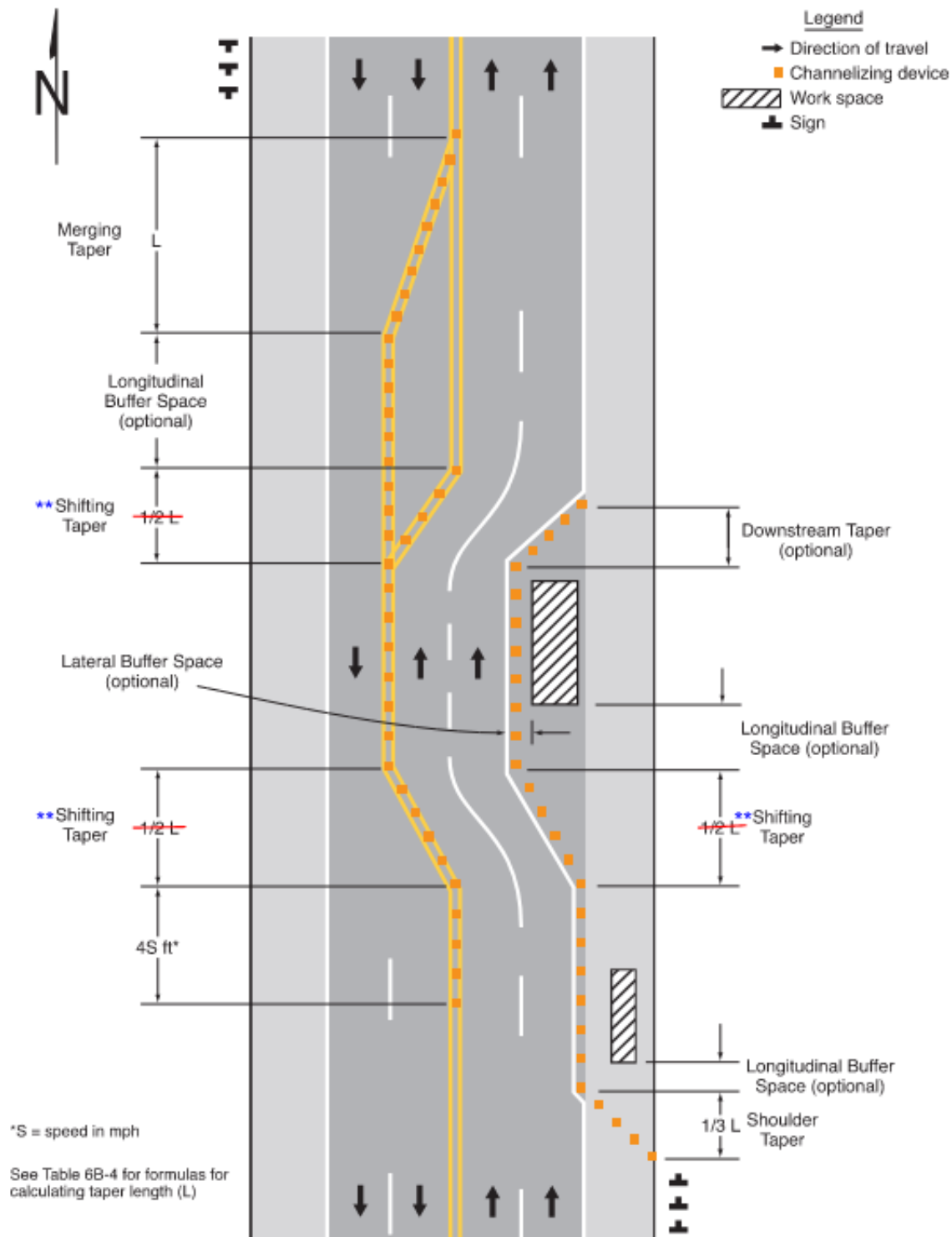
Figure 6B-2. Types of Tapers and Buffer Spaces
