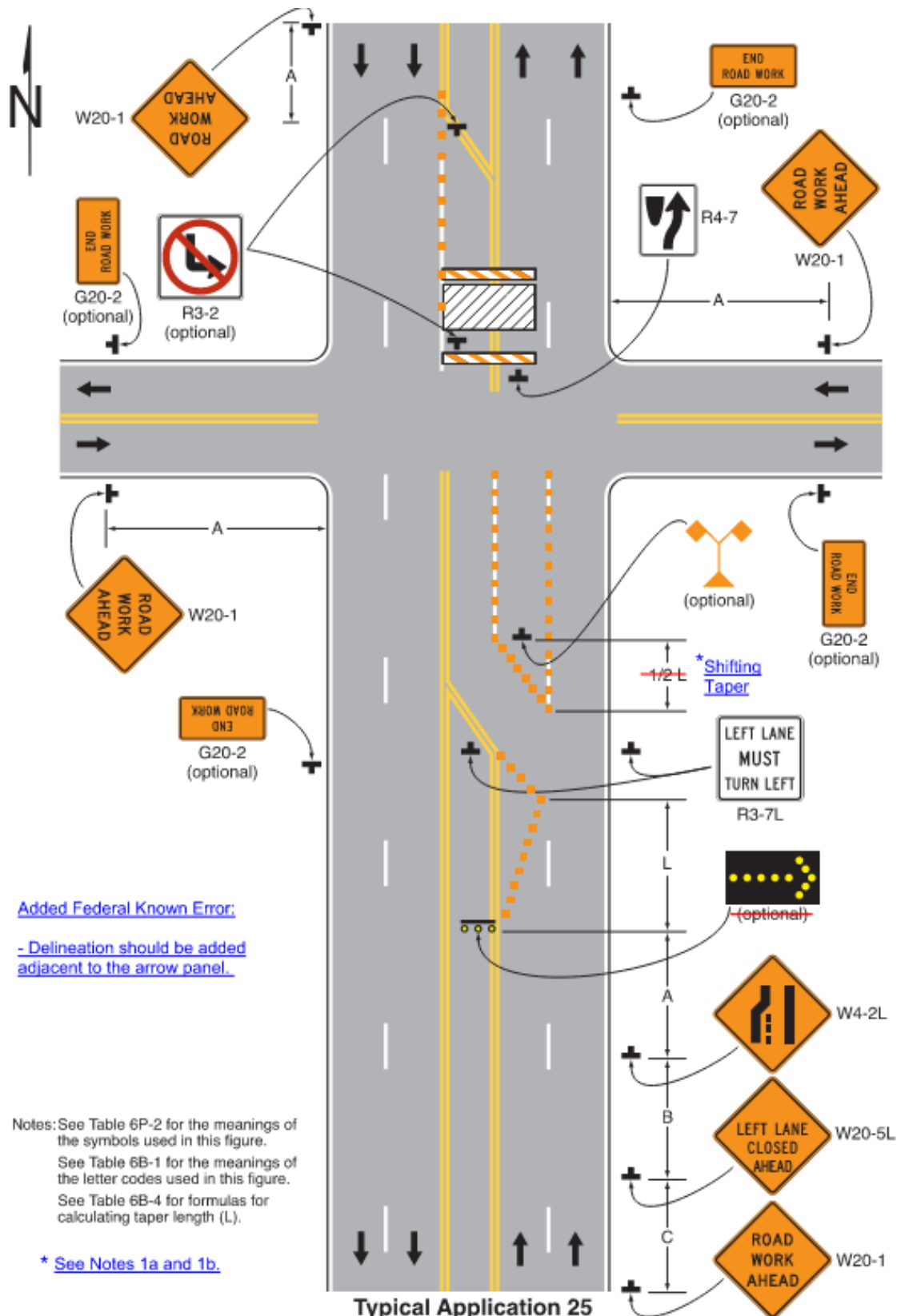
Figure 6P-25. Multiple Lane Closures at an Intersection
